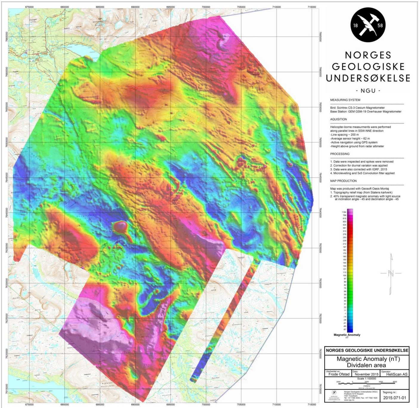
Figure 4: Total Magnetic Field Anomaly
