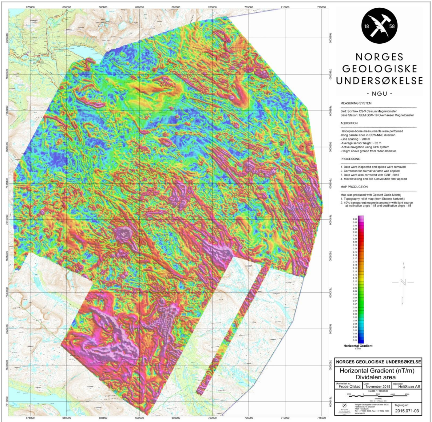
Figure 6: Magnetic Horizontal Derivative
