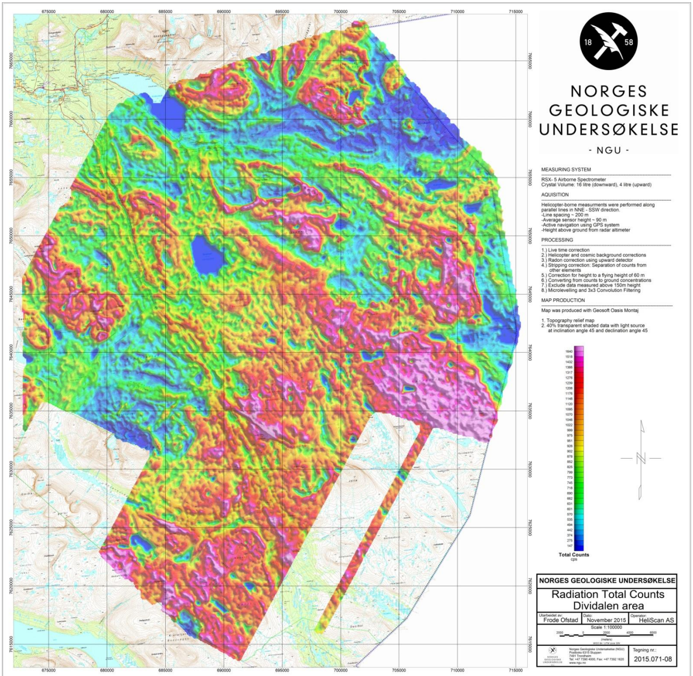
Figure 8: Radiation Total Counts
