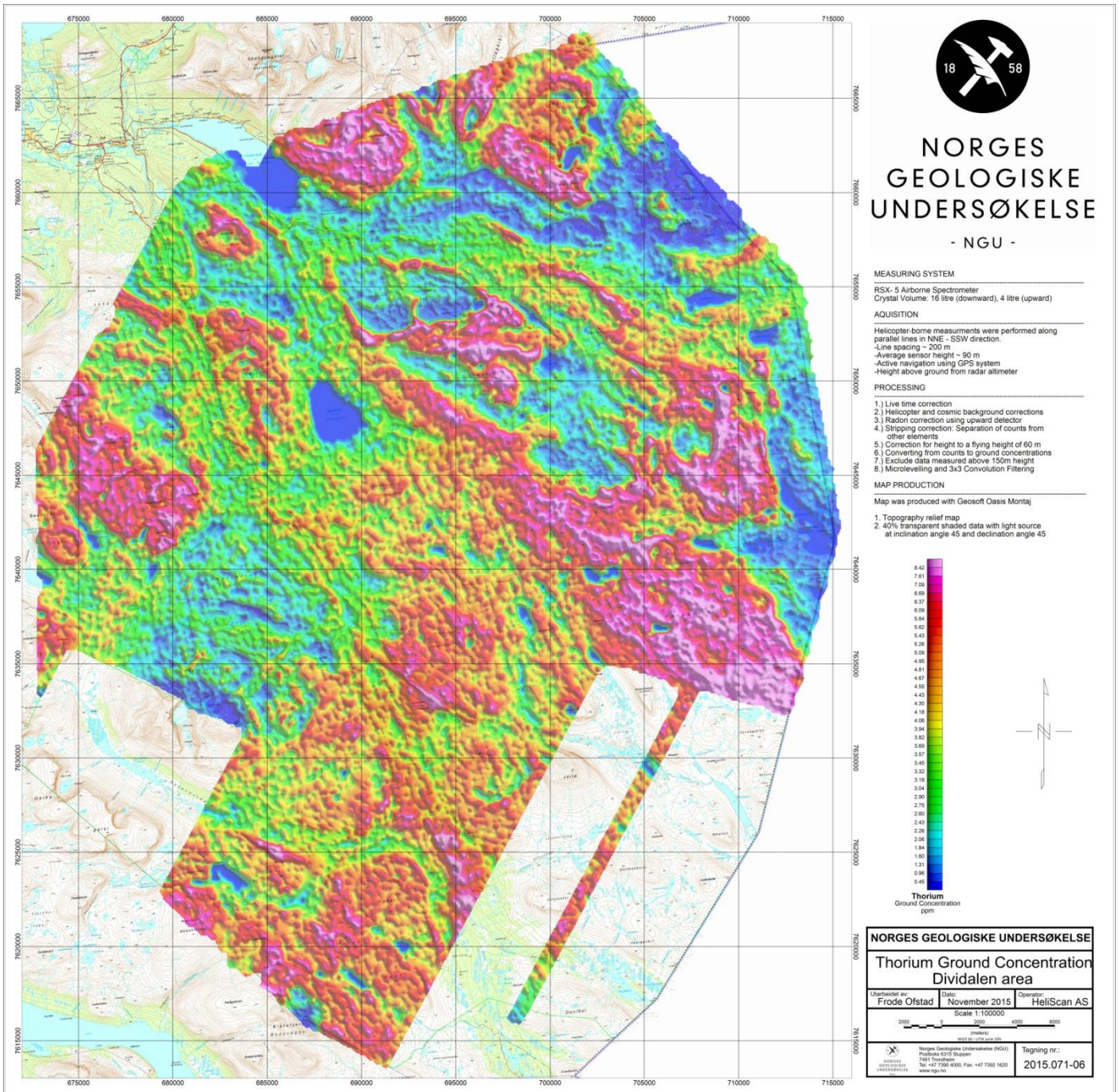
Figure 10: Thorium Ground Concentration
