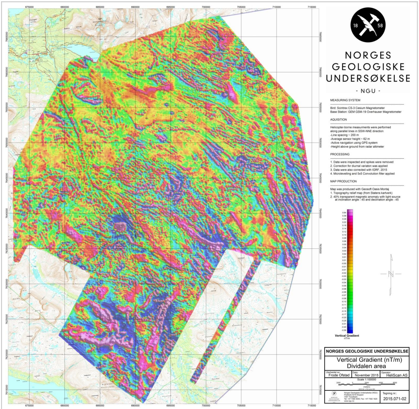
Figure 5: Magnetic Vertical Derivative
