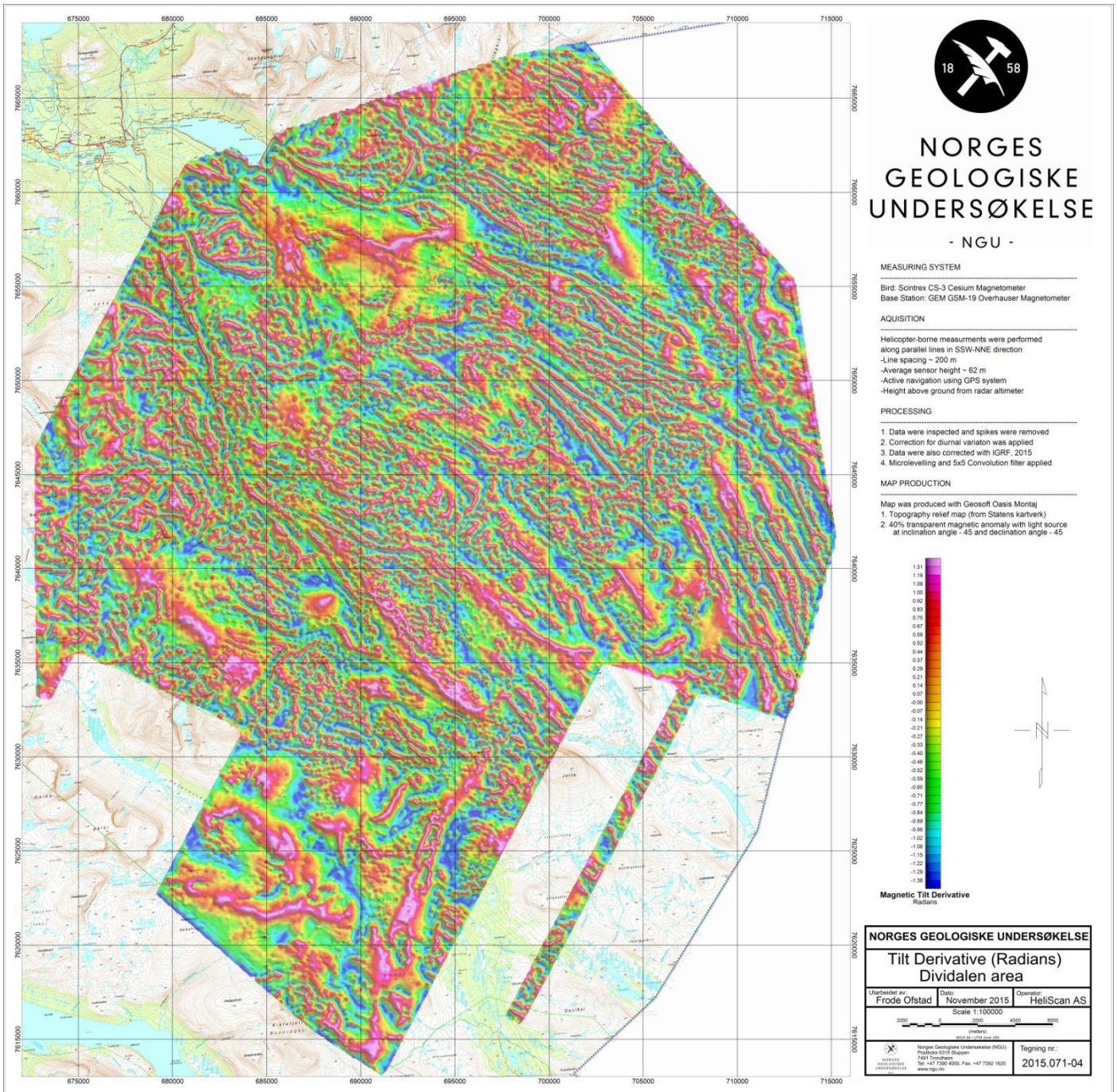
Figure 7: Magnetic Tilt Derivative
