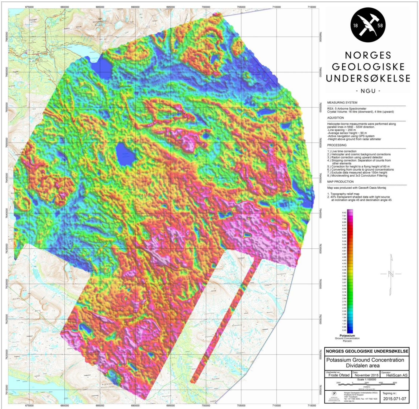
Figure 11: Potassium Ground Concentration
