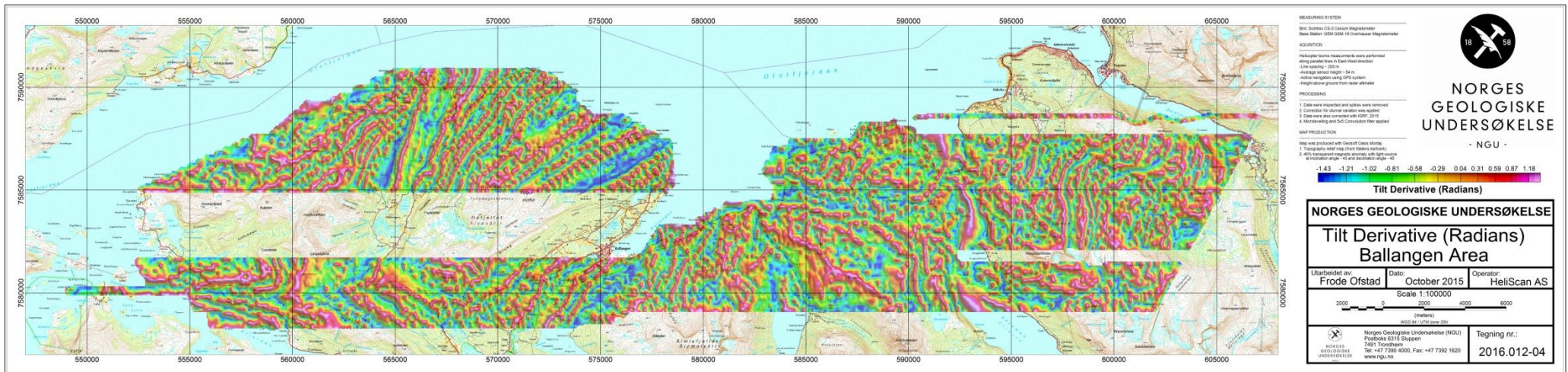
Figure 7: Magnetic Tilt Derivative
