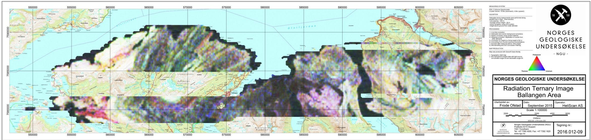
Figure 12: Radiometric Ternary Image
