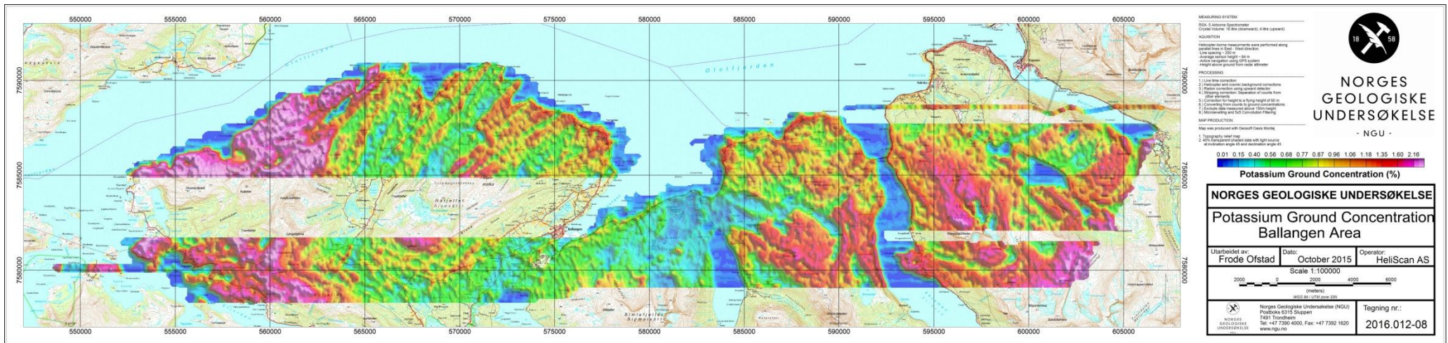
Figure 11: Potassium ground concentration
