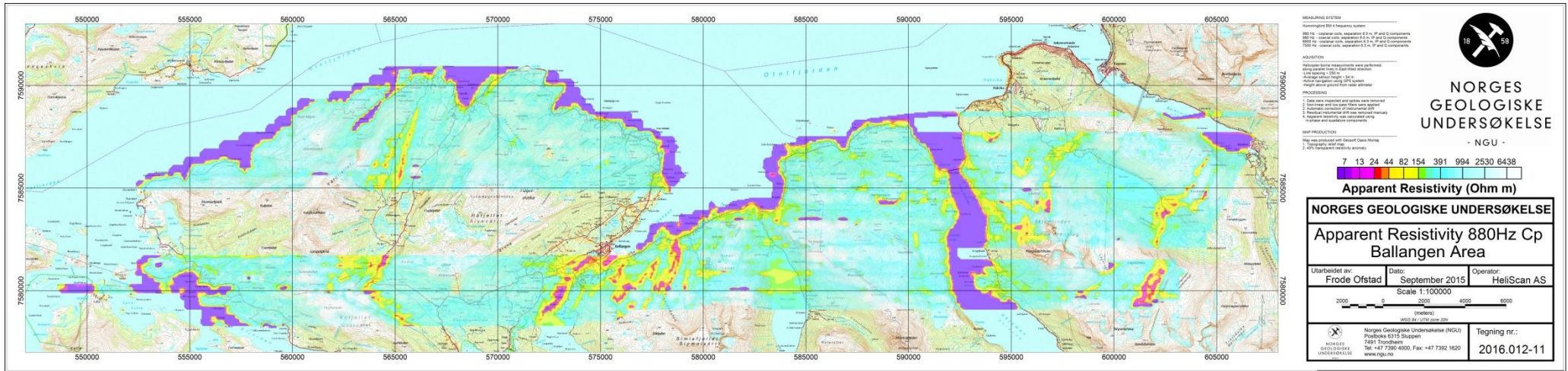
Figure 14: Apparent resistivity. Frequency 880 Hz, Coplanar coils
