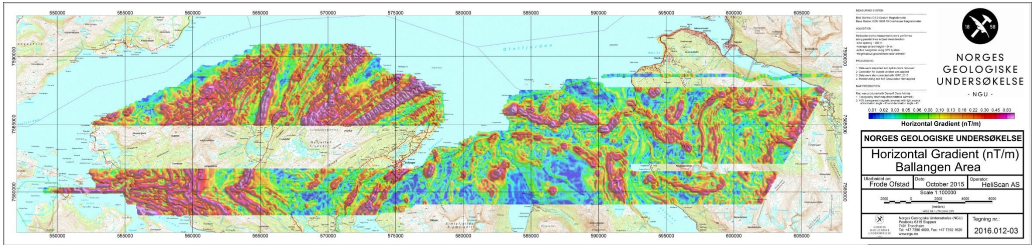
Figure 6: Magnetic Horizontal Derivative
