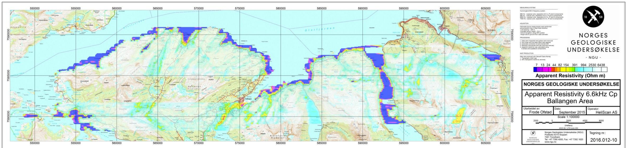
Figure 13: Apparent resistivity. Frequency 6600 Hz, Coplanar coils
