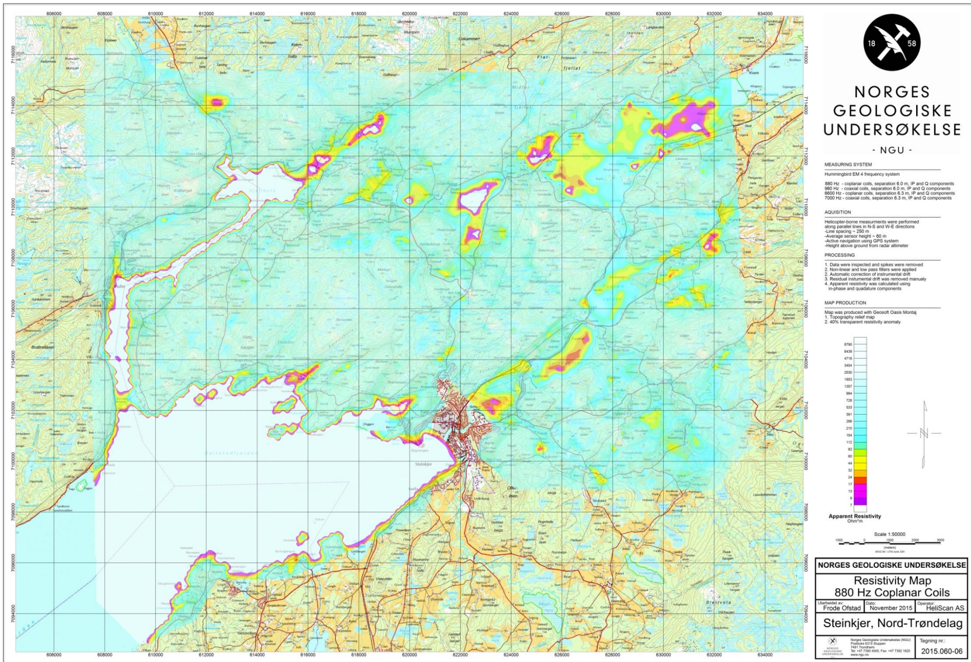
Figure 10: Apparent resistivity. Frequency 880 Hz, Coplanar coils
