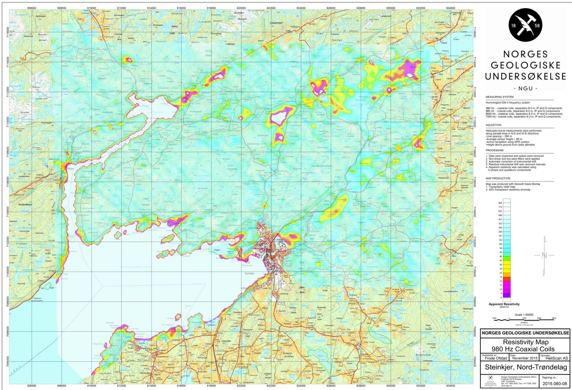
Figure 12: Apparent resistivity. Frequency 980 Hz, Coaxial coils
