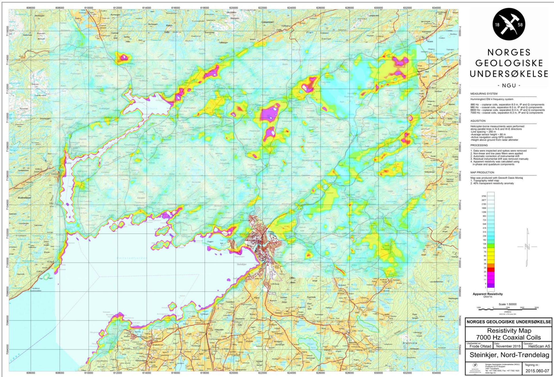
Figure 11: Apparent resistivity. Frequency 7000 Hz, Coaxial coils
