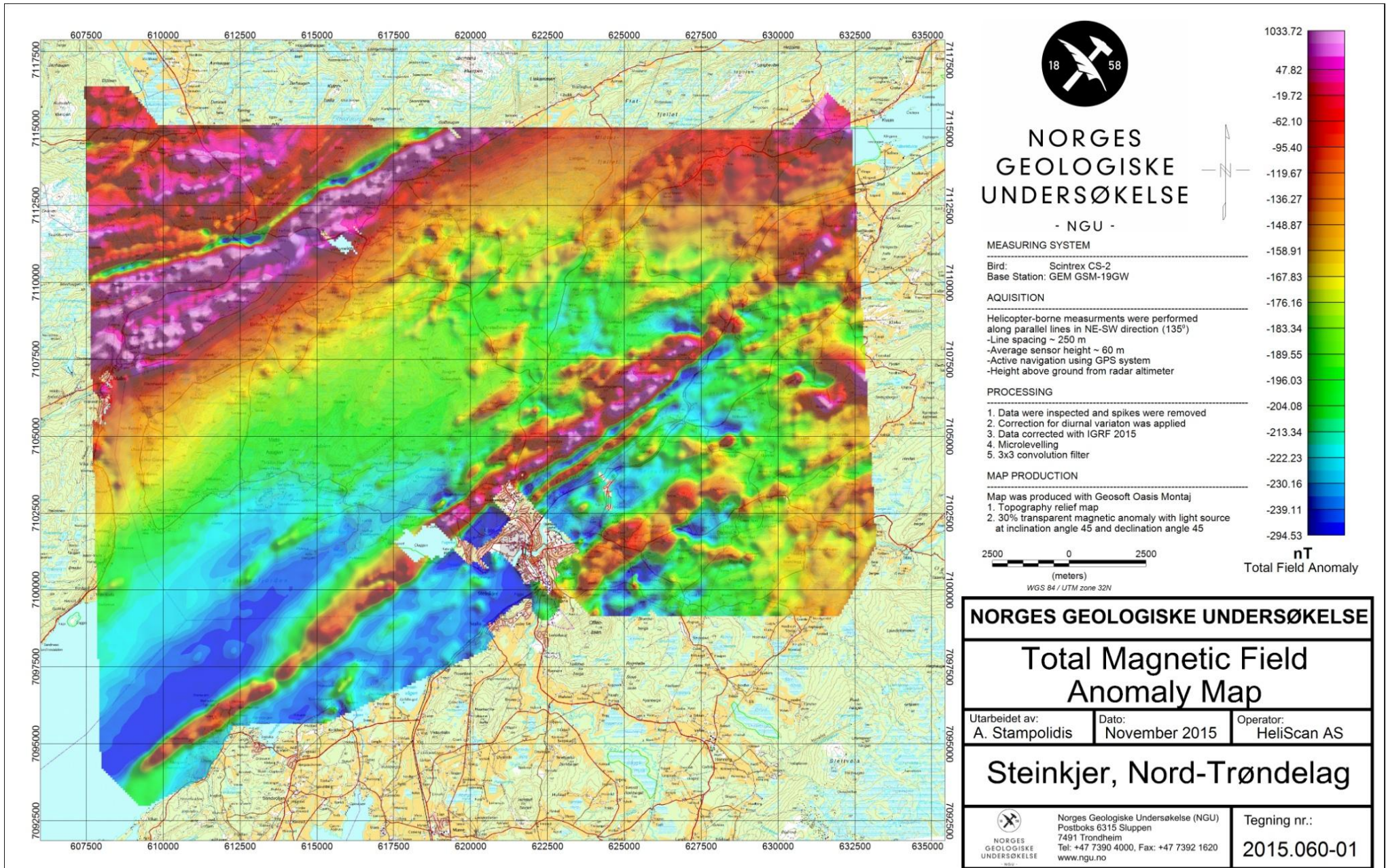
Figure 5: Total Magnetic Field Anomaly
