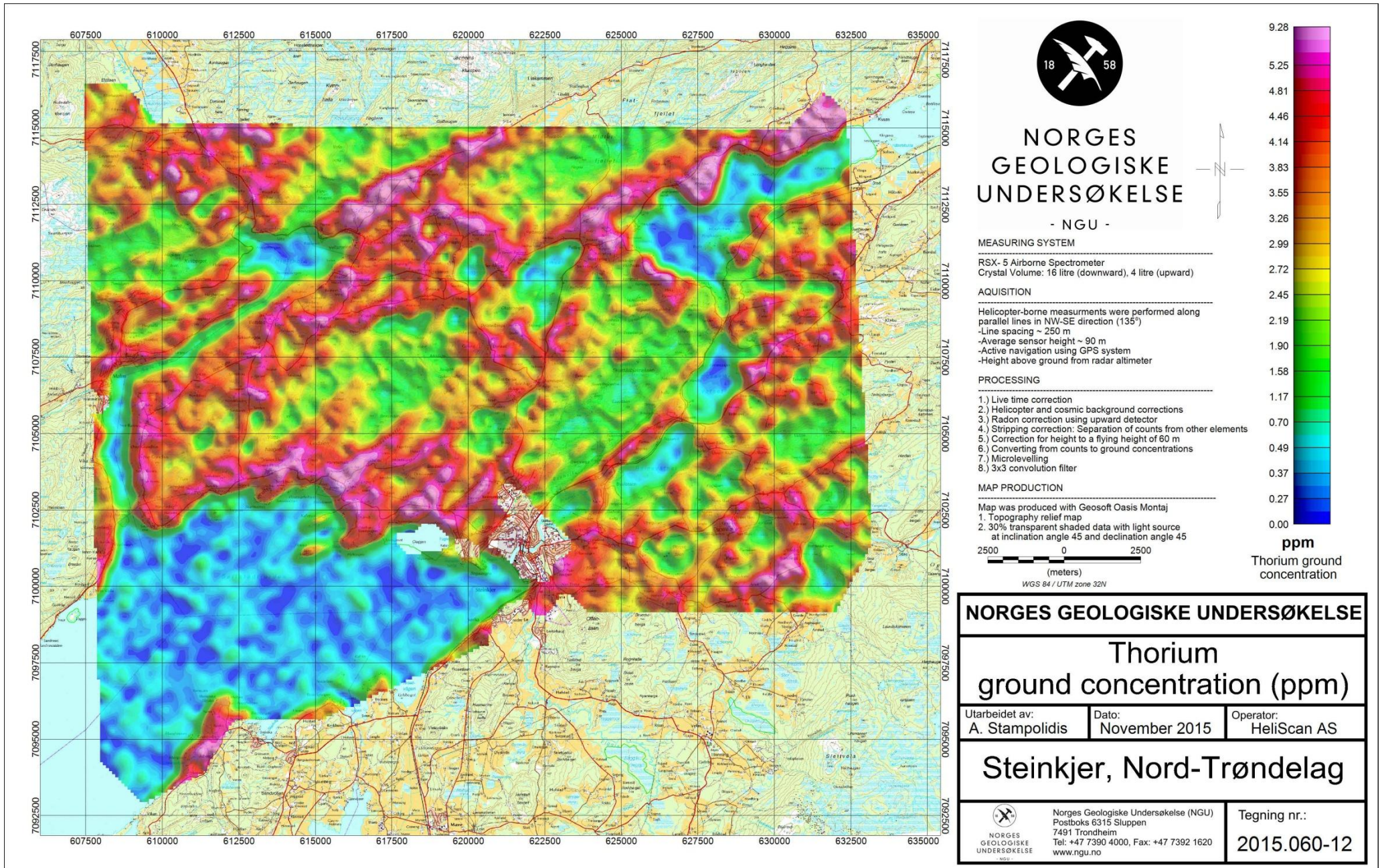
Figure 16: Thorium ground concentration
