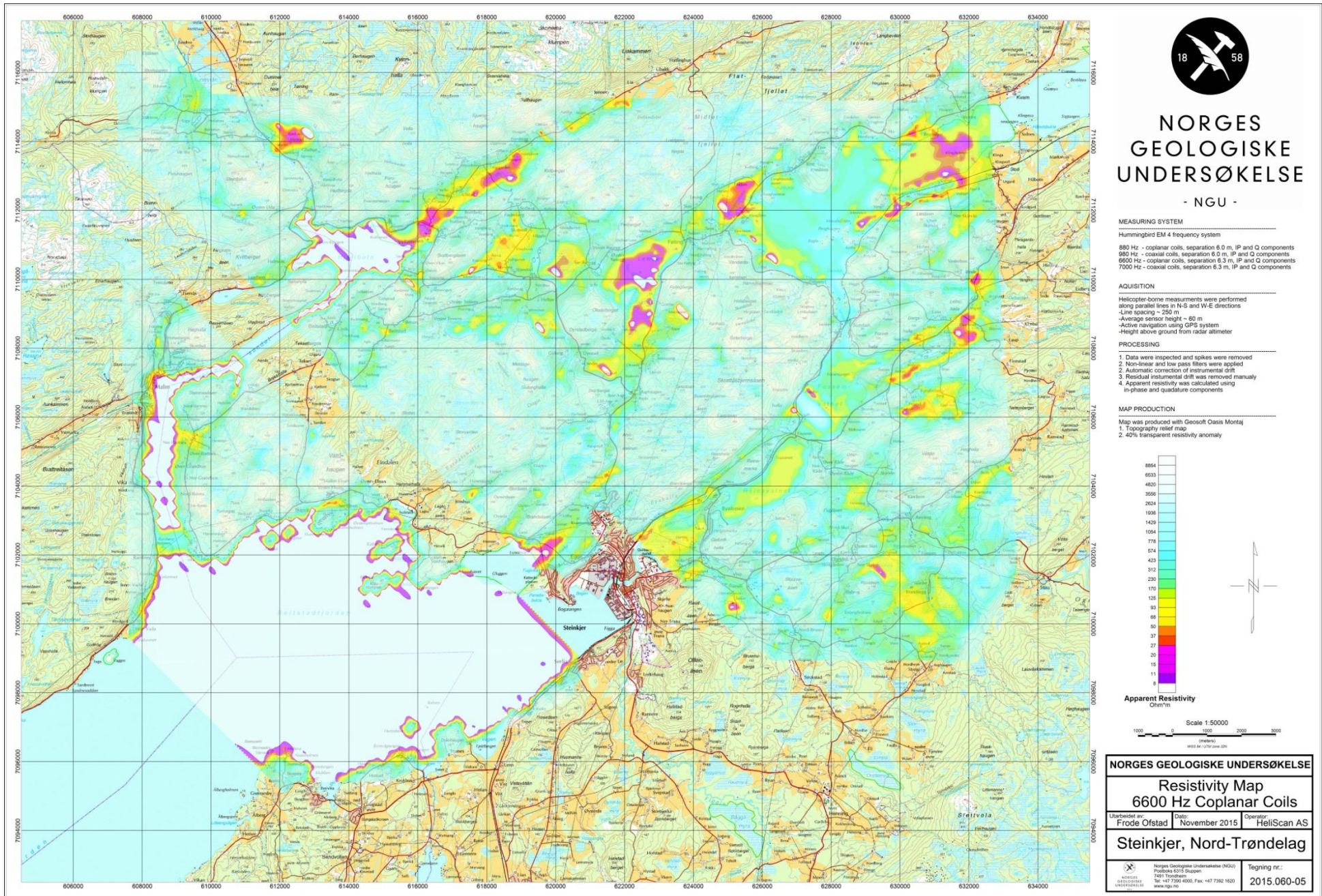
Figure 9: Apparent resistivity. Frequency 6600 Hz, Coplanar coils
