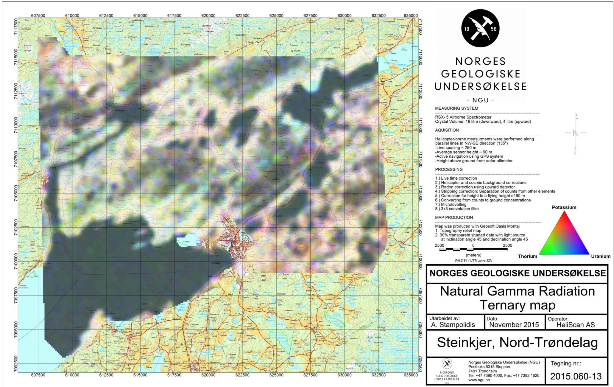
Figure 17: Radiometric Ternary map
