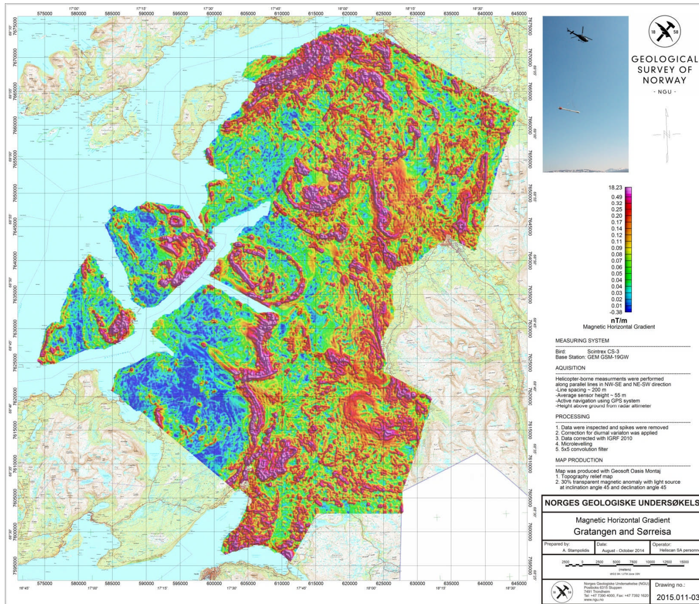
Figure 6: Magnetic Horizontal Gradient map
