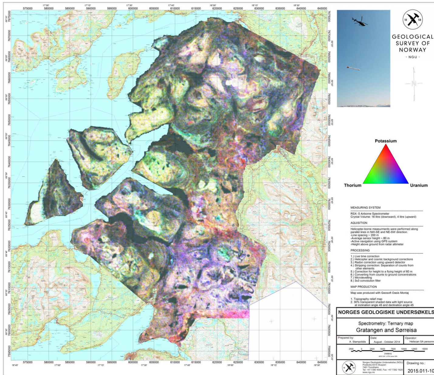
Figure 13: Ternary Image of Radiation Concentration
