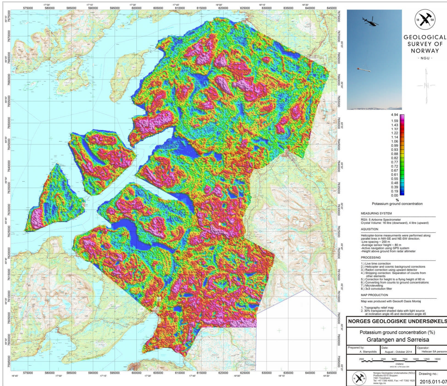
Figure 10: Potassium Ground Concentration map
