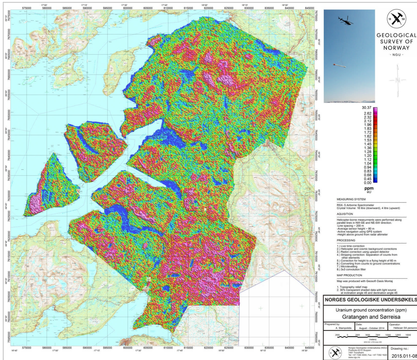
Figure 11: Uranium Ground Concentration map
