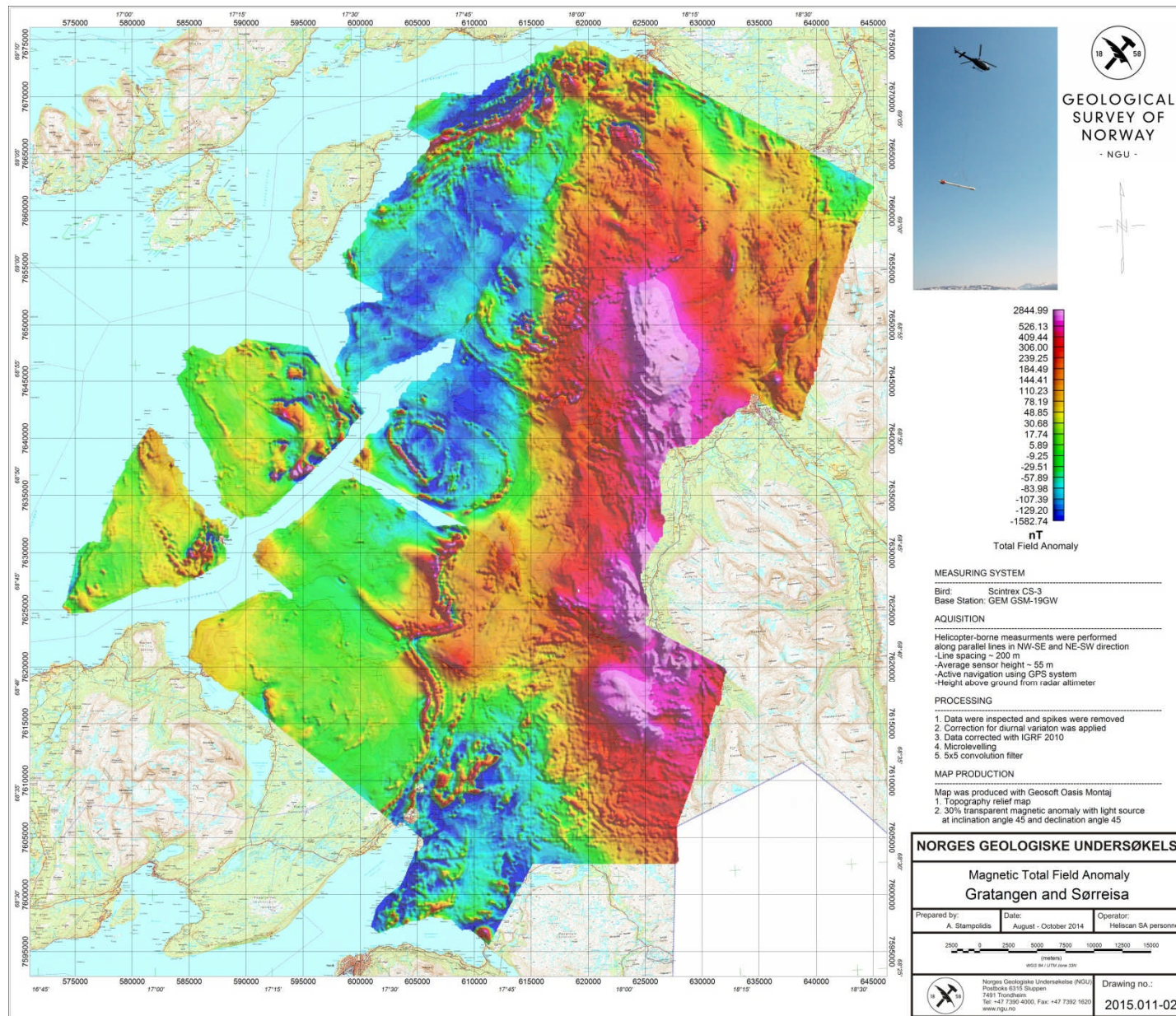
Figure 5: Total Magnetic Field anomaly map
