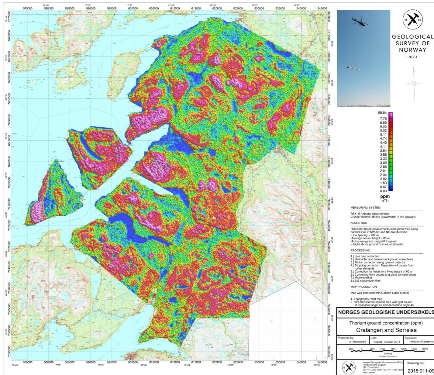
Figure 12: Thorium Ground Concentration map
