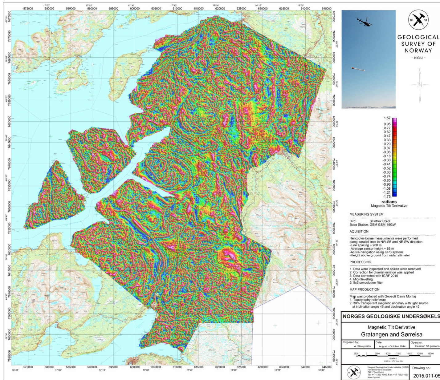
Figure 8: Magnetic Tilt Derivative map
