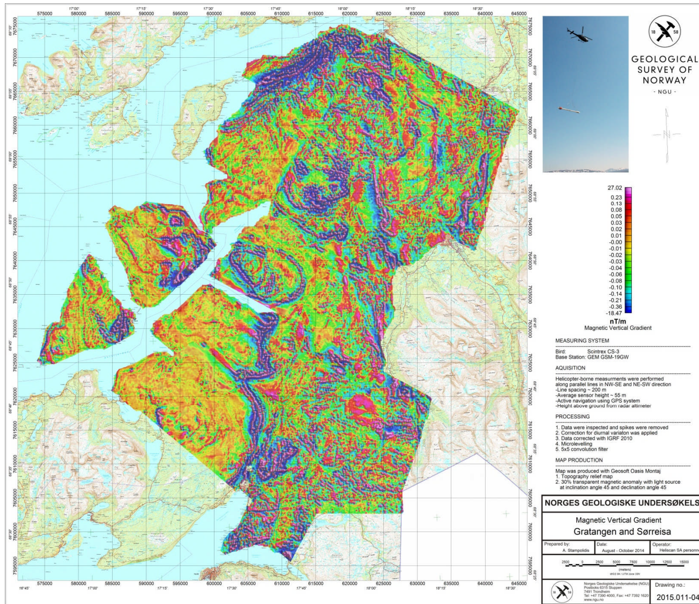
Figure 7: Magnetic Vertical Gradient map
