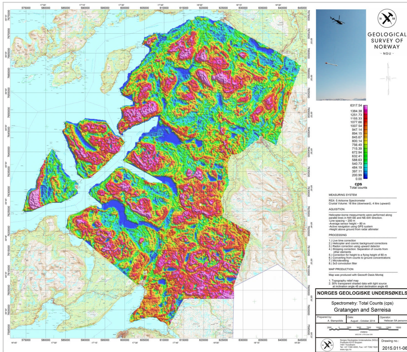
Figure 9: Radiometry: Total Counts map
