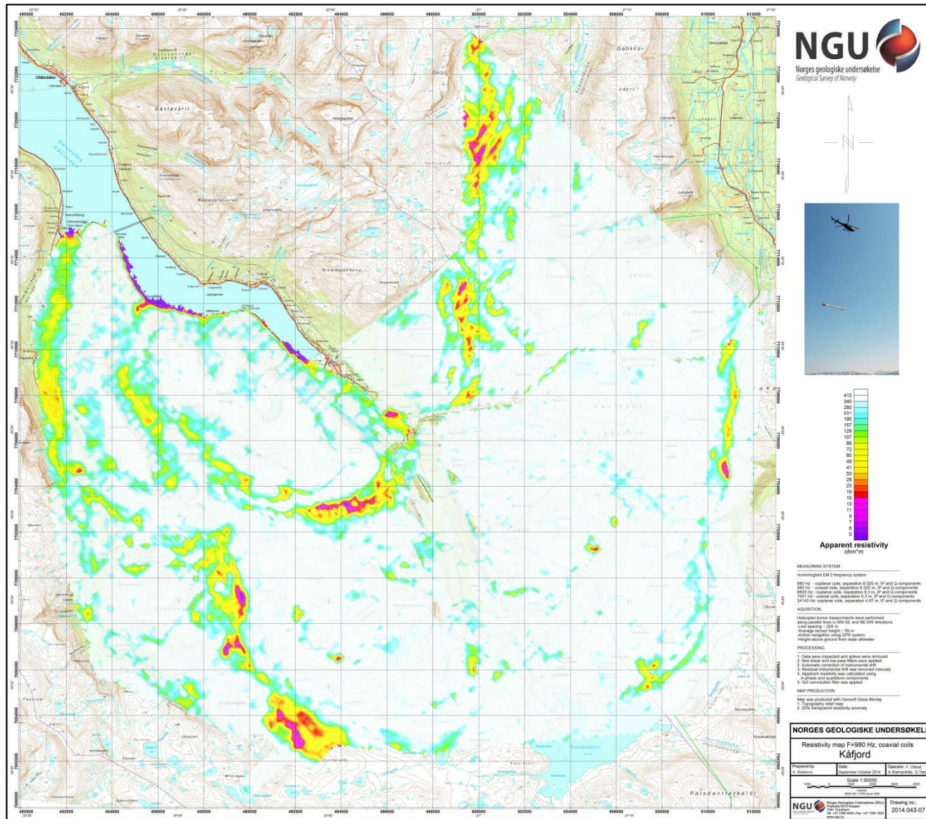
Figure 11: Apparent resistivity. Frequency 980 Hz, Coaxial coils
