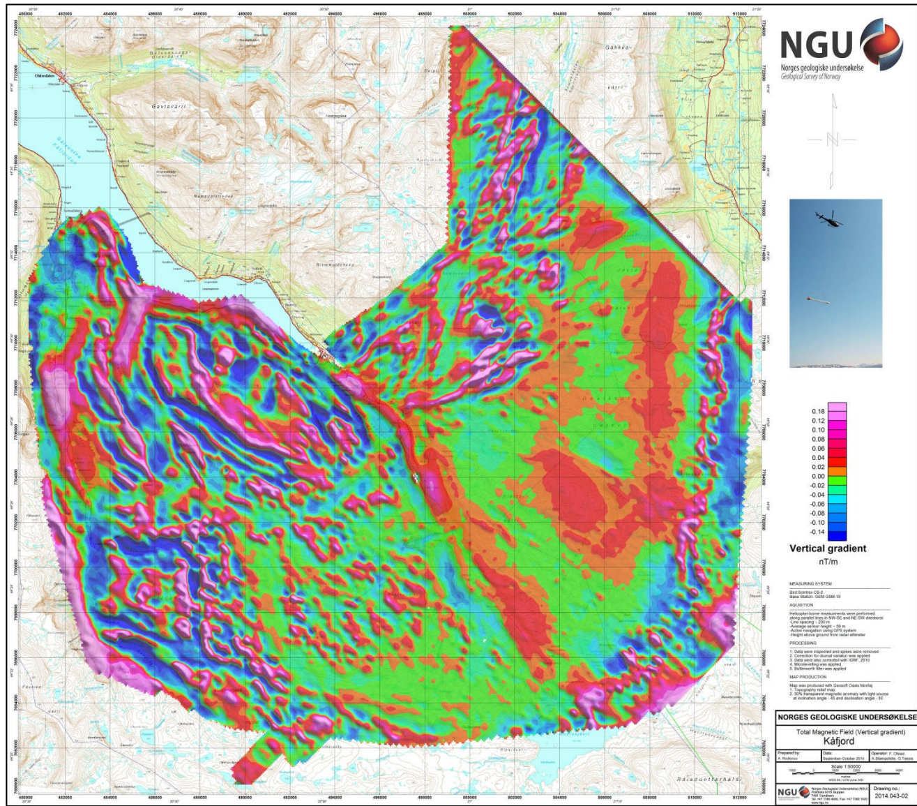
Figure 6: Magnetic Vertical Derivative
