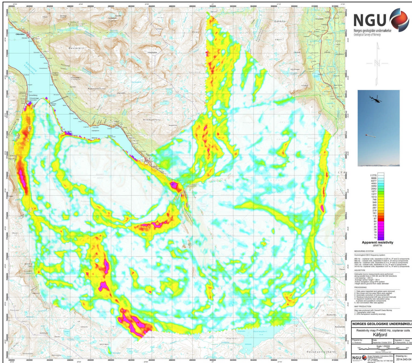
Figure 8: Apparent resistivity. Frequency 6600 Hz, Coplanar coils
