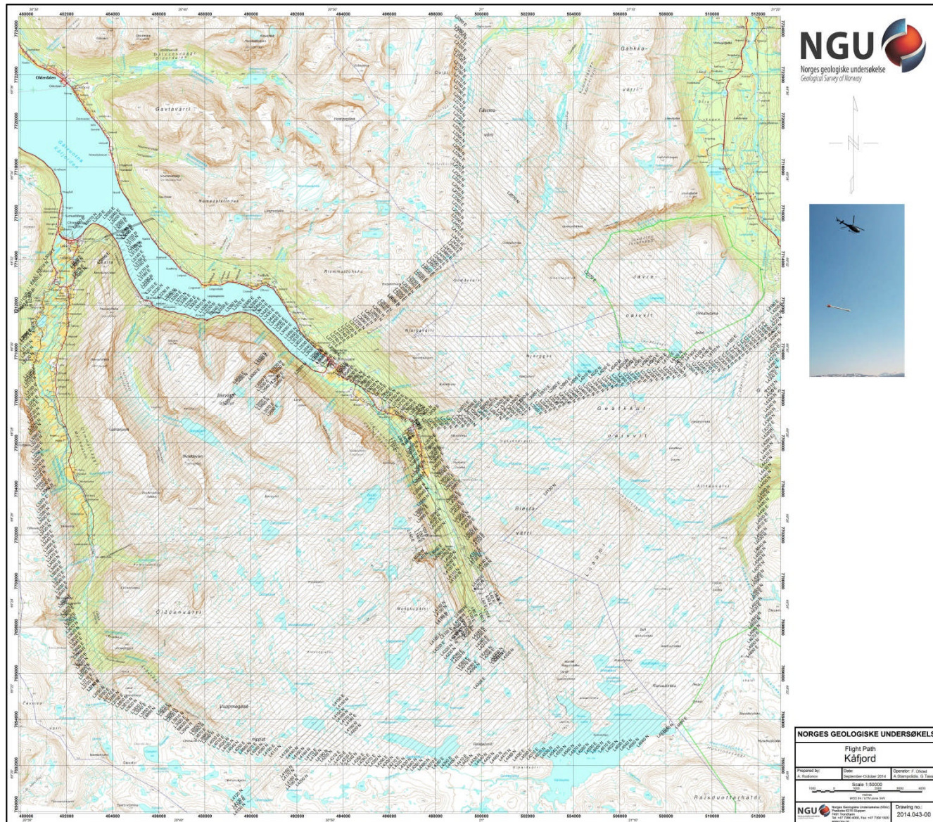
Figure 4: Kåfjord survey area with flight path
