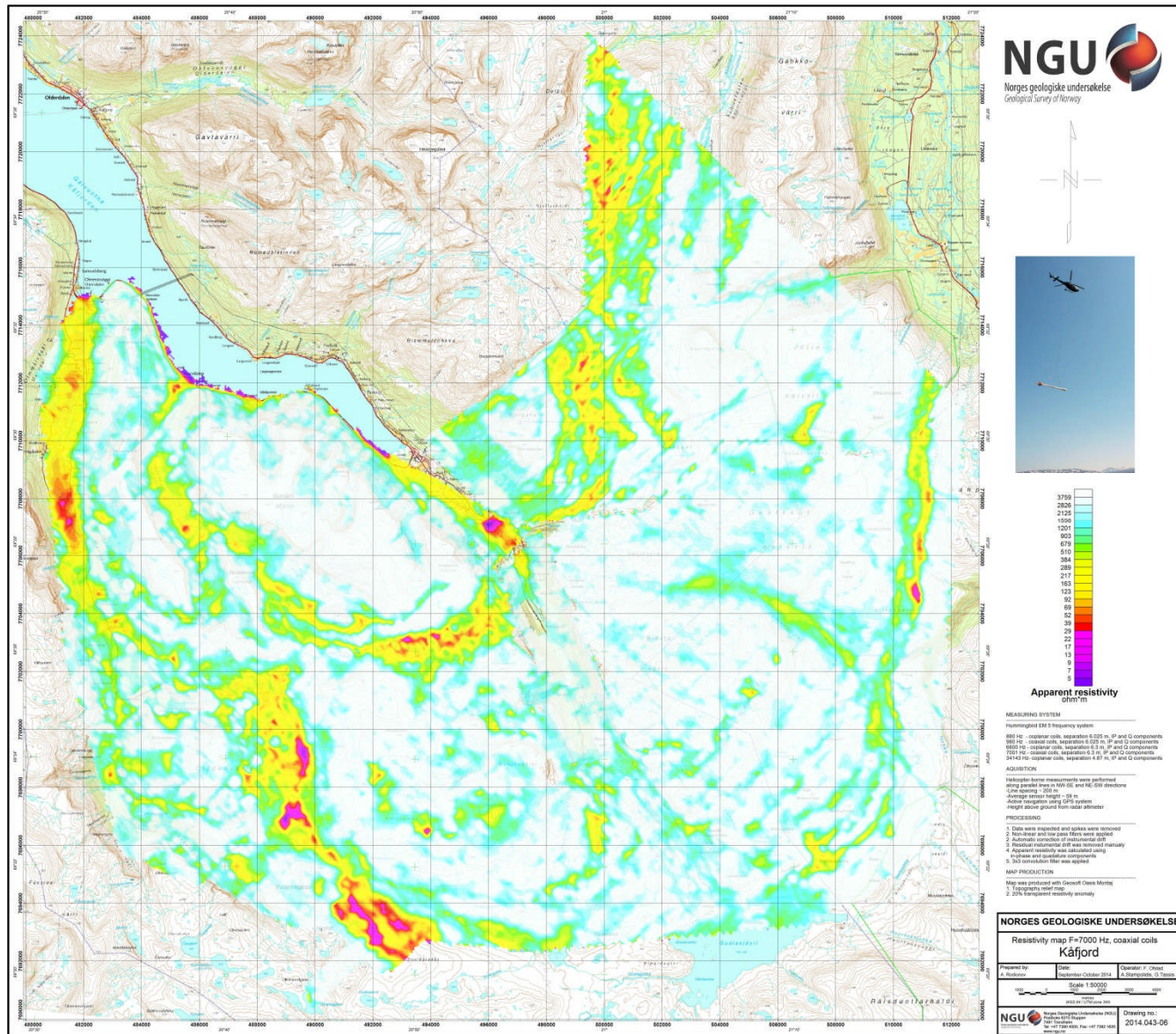
Figure 10: Apparent resistivity. Frequency 7000 Hz, Coaxial coils
