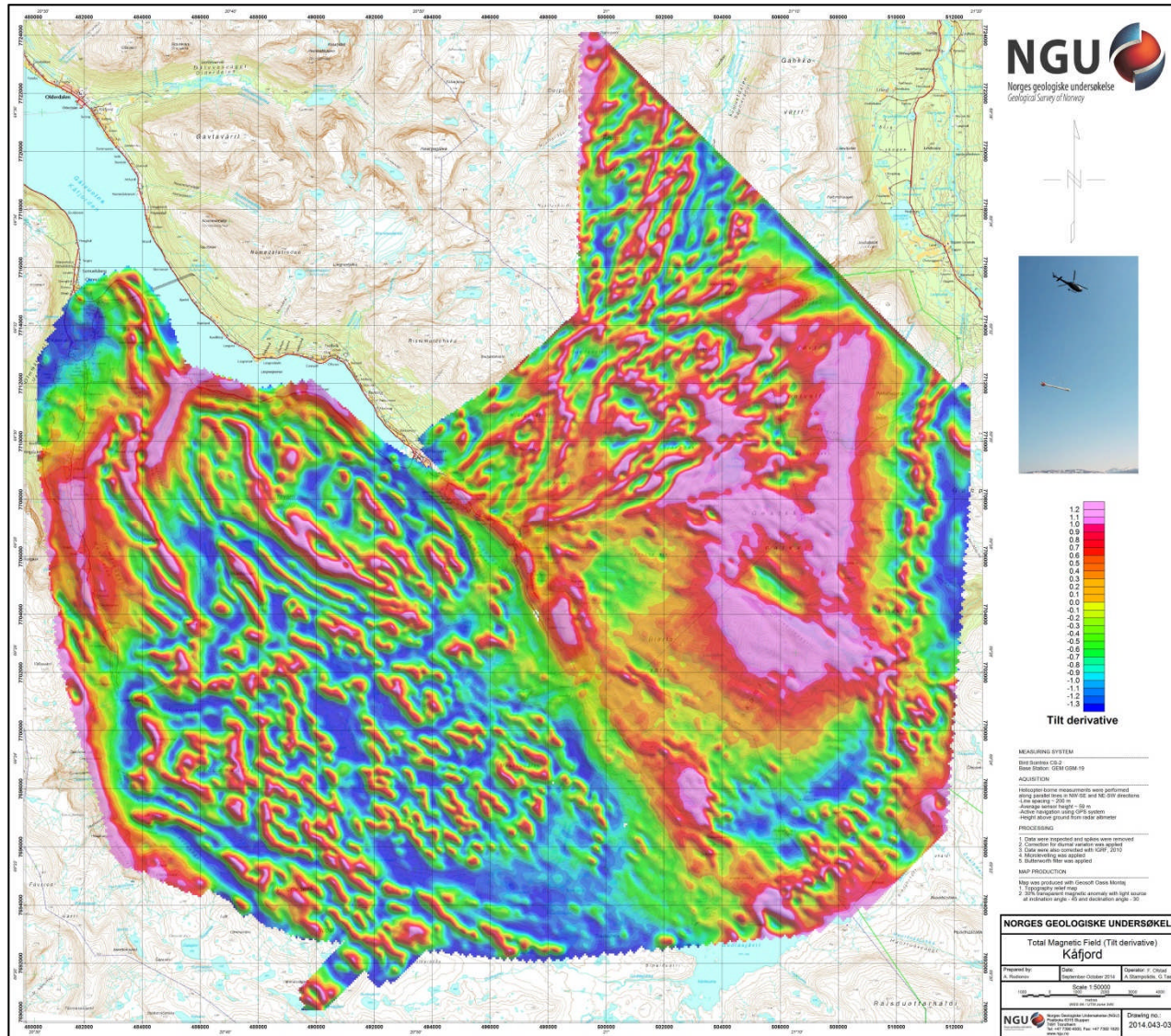
Figure 7: Magnetic Tilt Derivative
