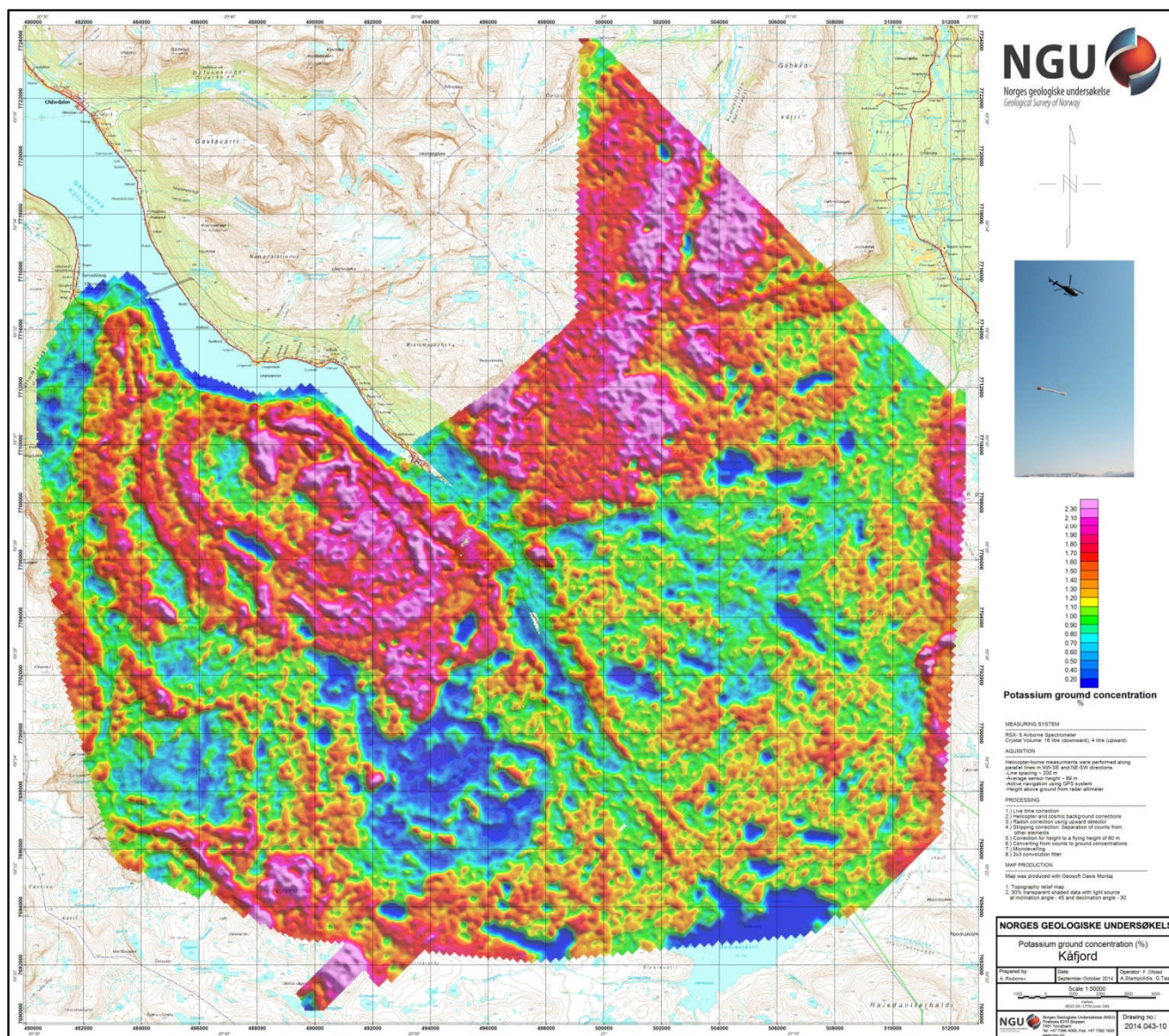
Figure 14: Potassium ground concentration
