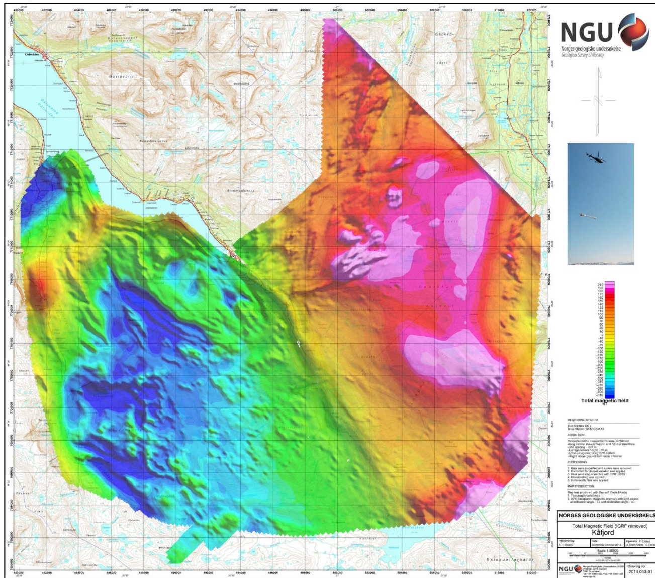
Figure 5: Total Magnetic Field
