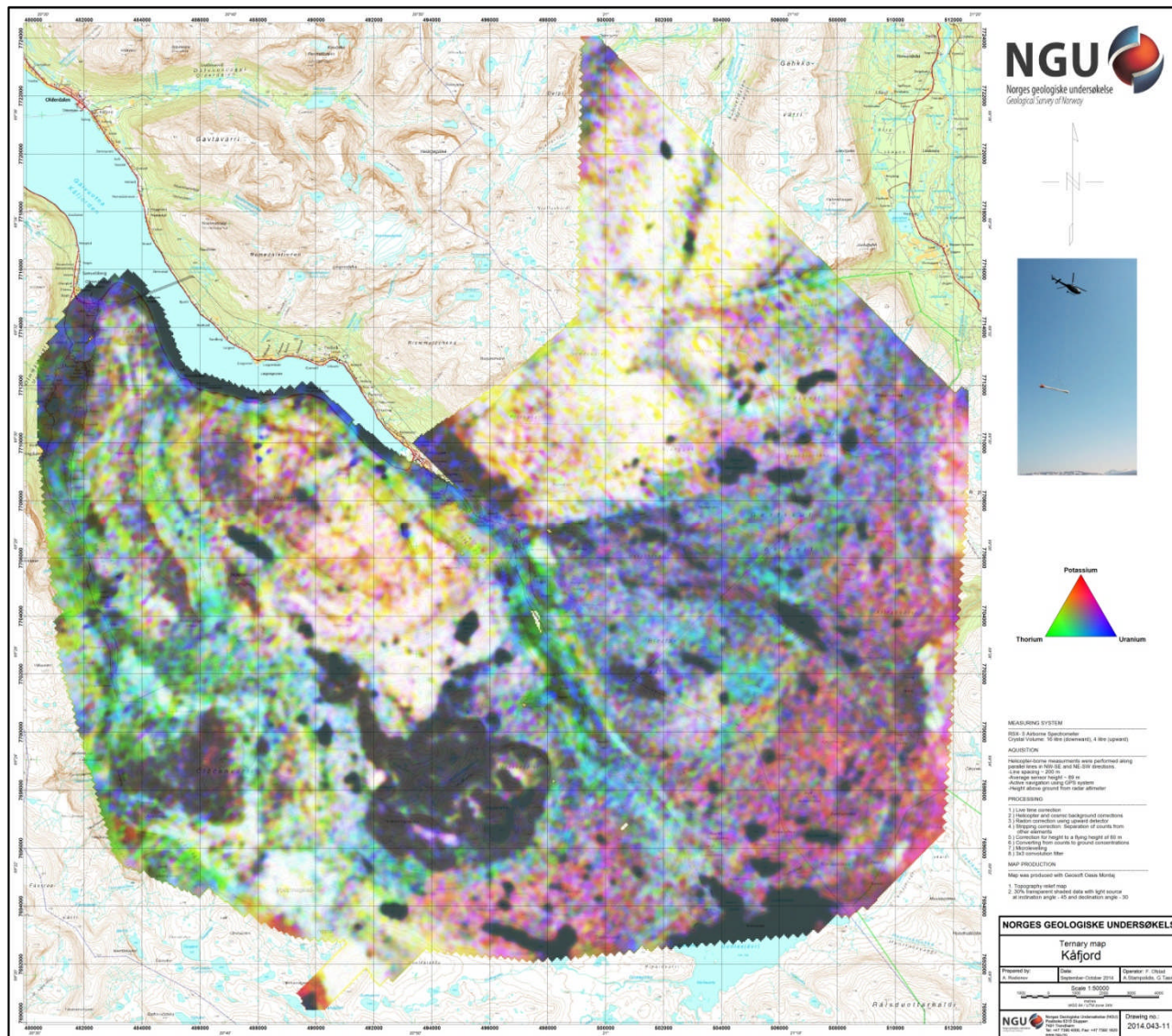
Figure 15: Radiometric Ternary map
