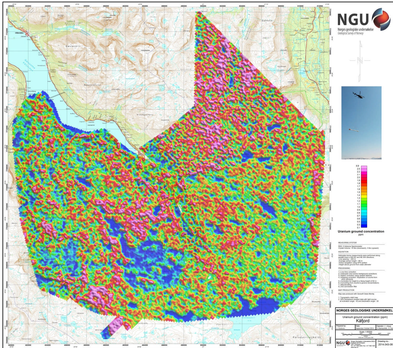
Figure 12: Uranium ground concentration
