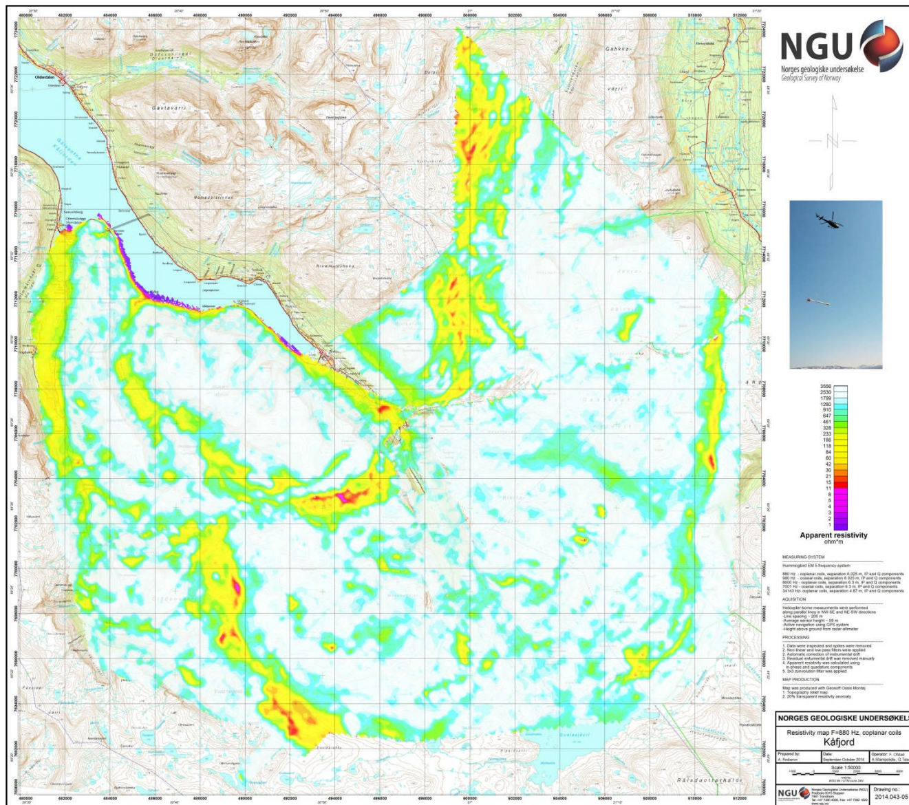
Figure 9: Apparent resistivity. Frequency 880 Hz, coplanar coils
