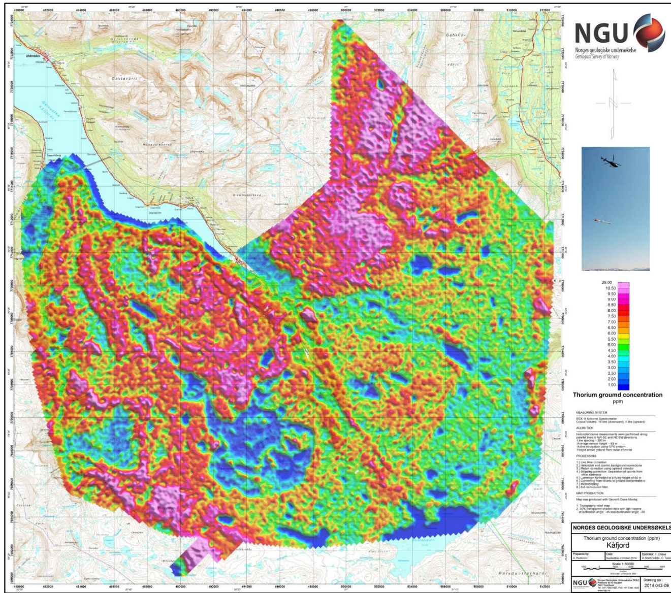
Figure 13: Thorium ground concentration
