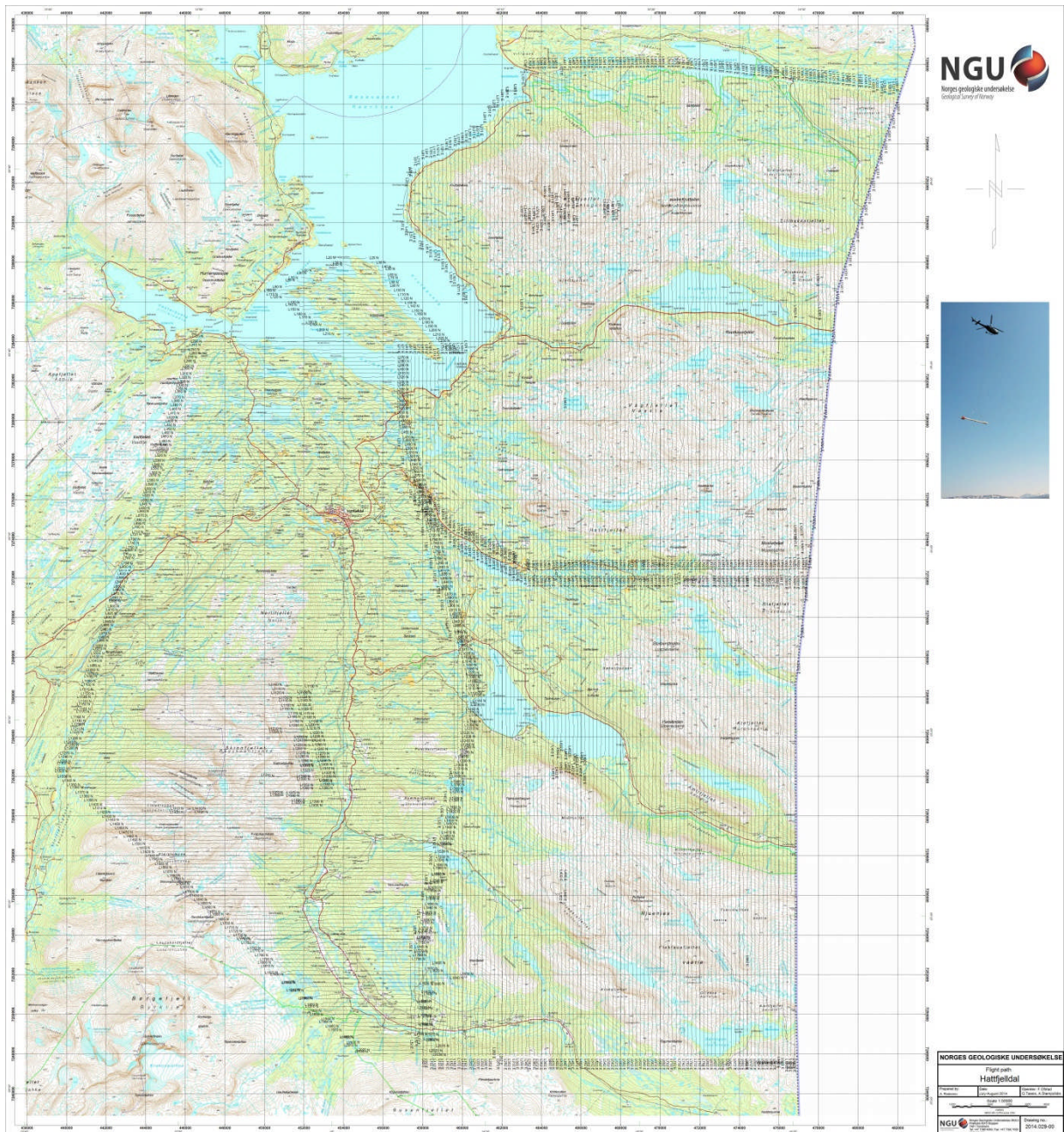
Figure 4: Hattfjelldal survey area with flight path
