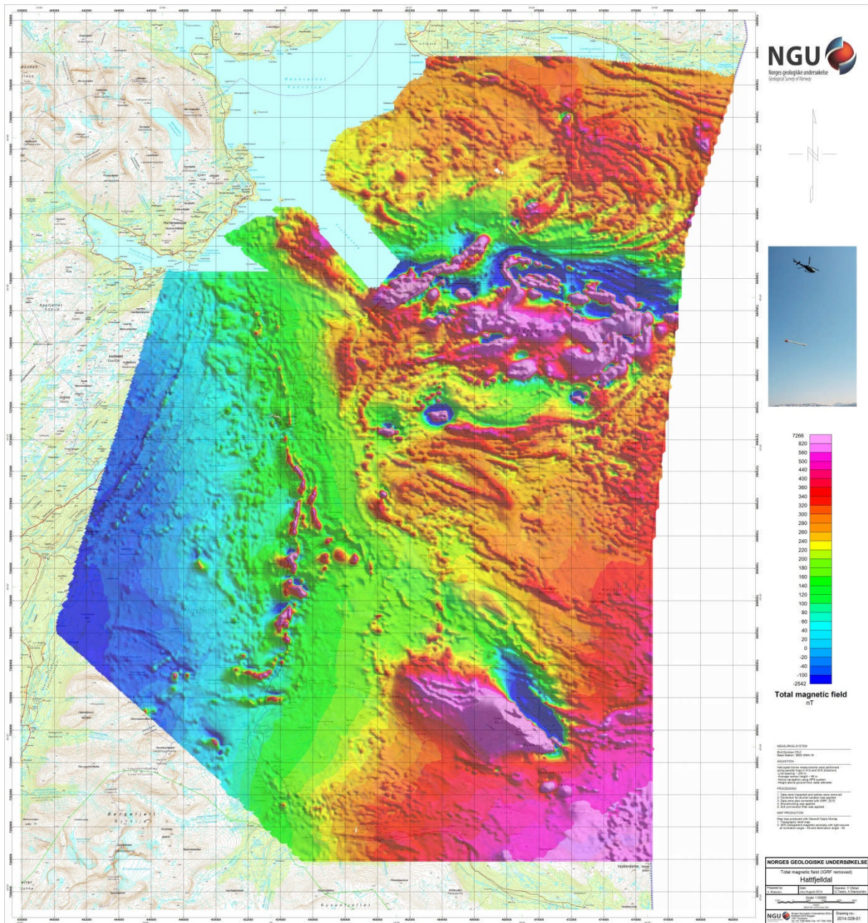
Figure 5: Total Magnetic Field
