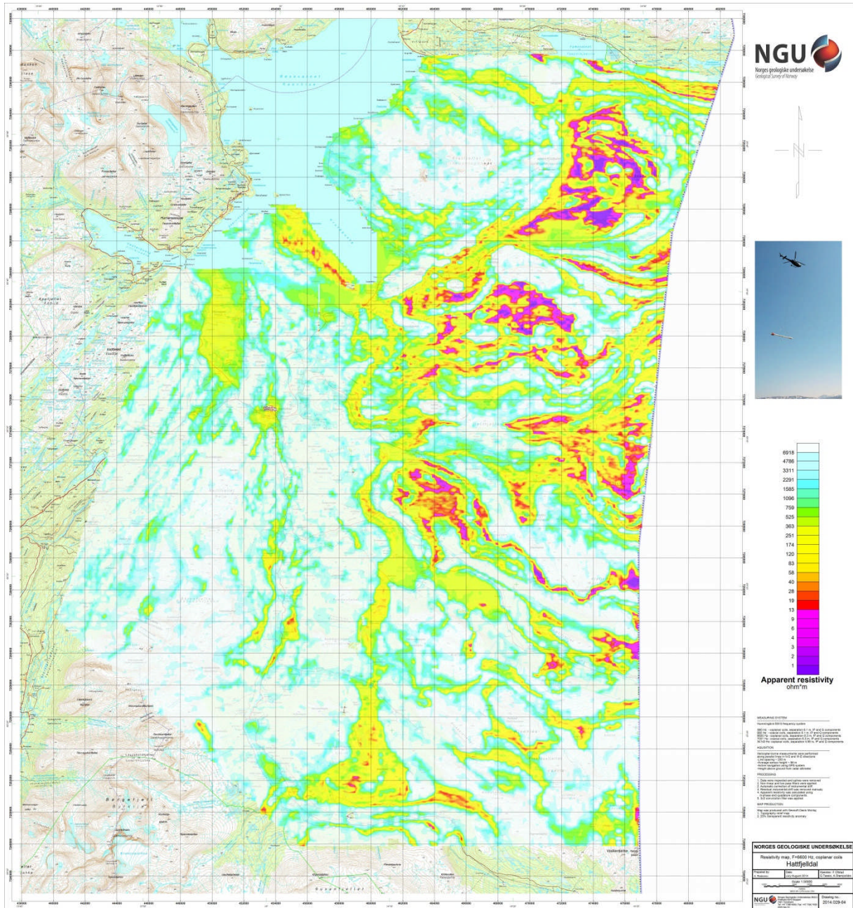
Figure 8: Apparent resistivity. Frequency 6600 Hz, Coplanar coils
