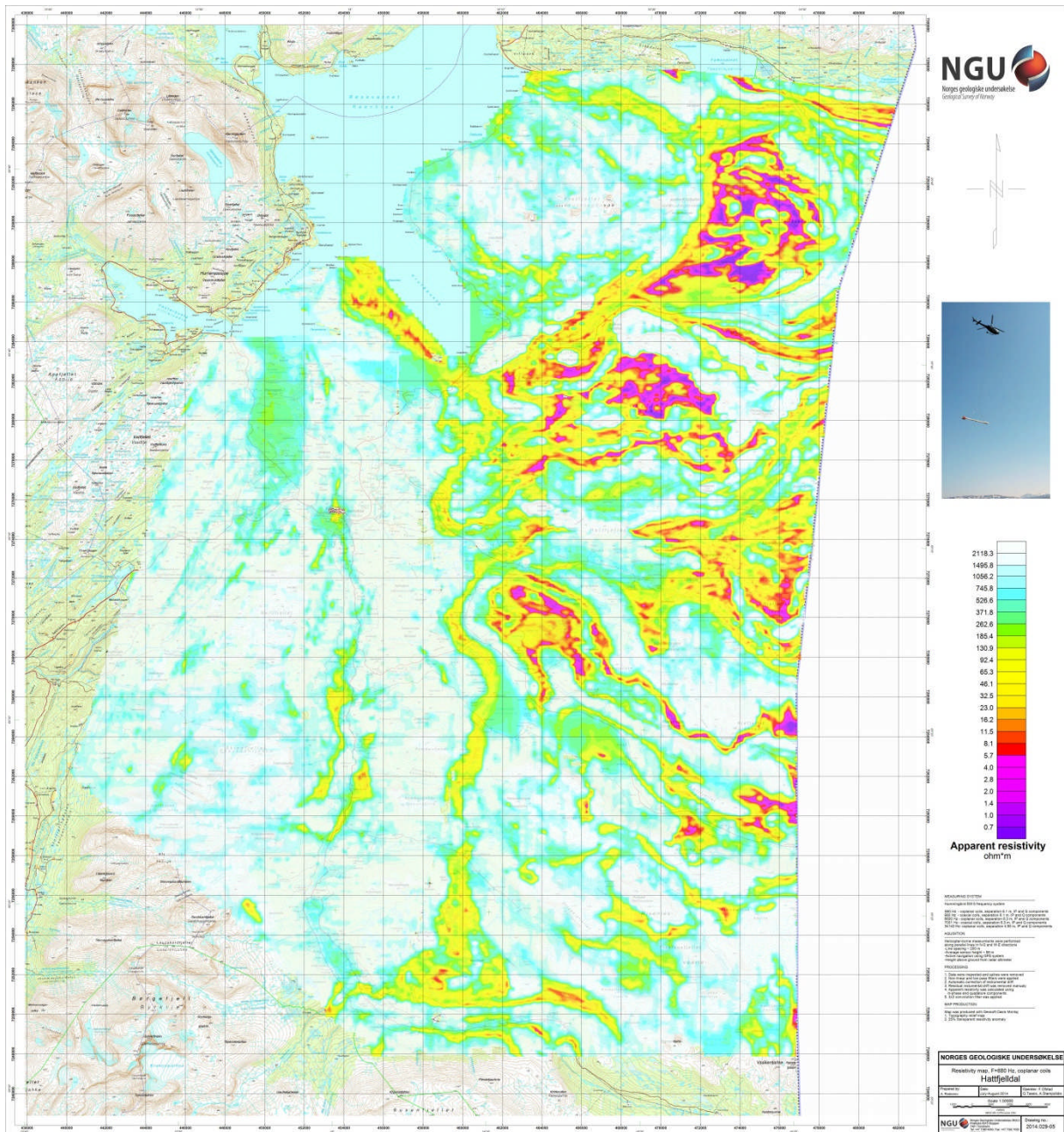
Figure 9: Apparent resistivity. Frequency 880 Hz, coplanar coils
