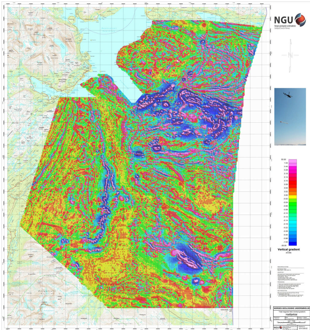
Figure 6: Magnetic Vertical Derivative
