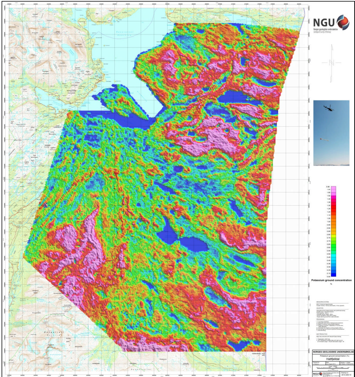
Figure 14: Potassium ground concentration
