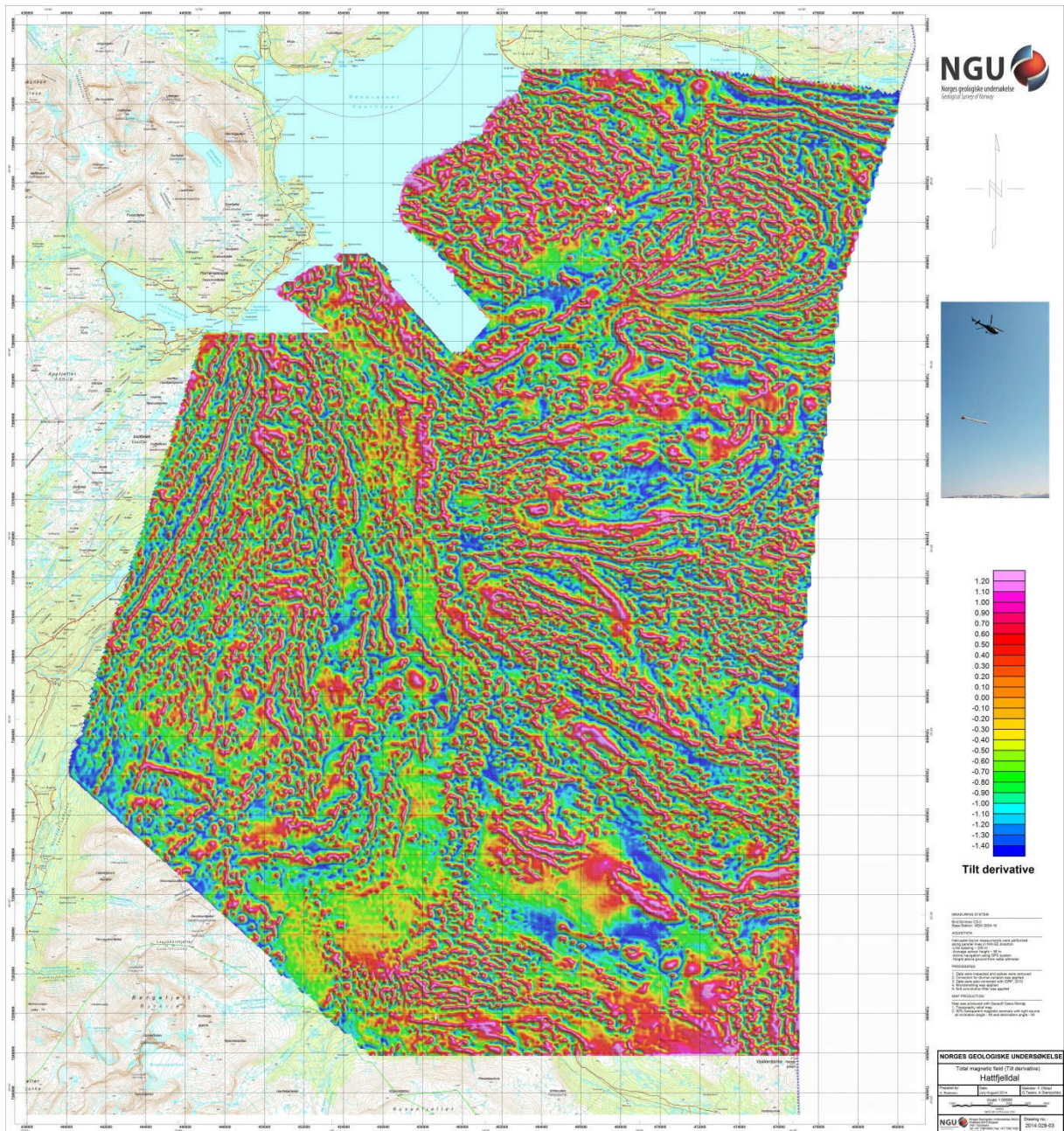
Figure 7: Magnetic Tilt Derivative
