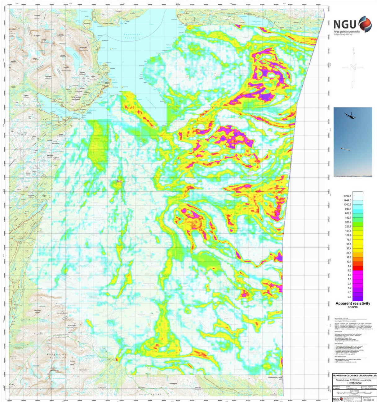
Figure 10: Apparent resistivity. Frequency 7000 Hz, Coaxial coils
