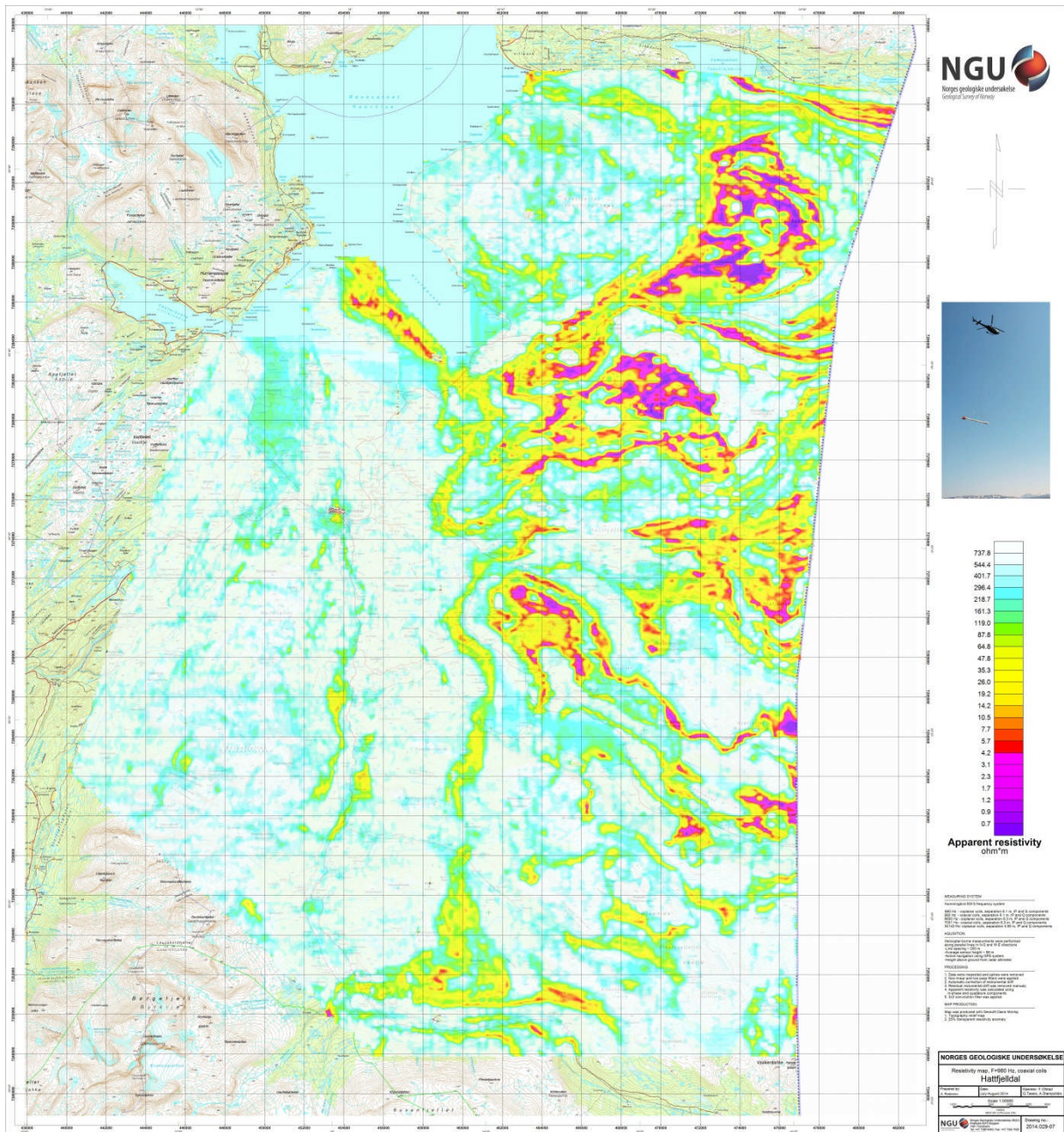
Figure 11: Apparent resistivity. Frequency 7000 Hz, Coaxial coils
