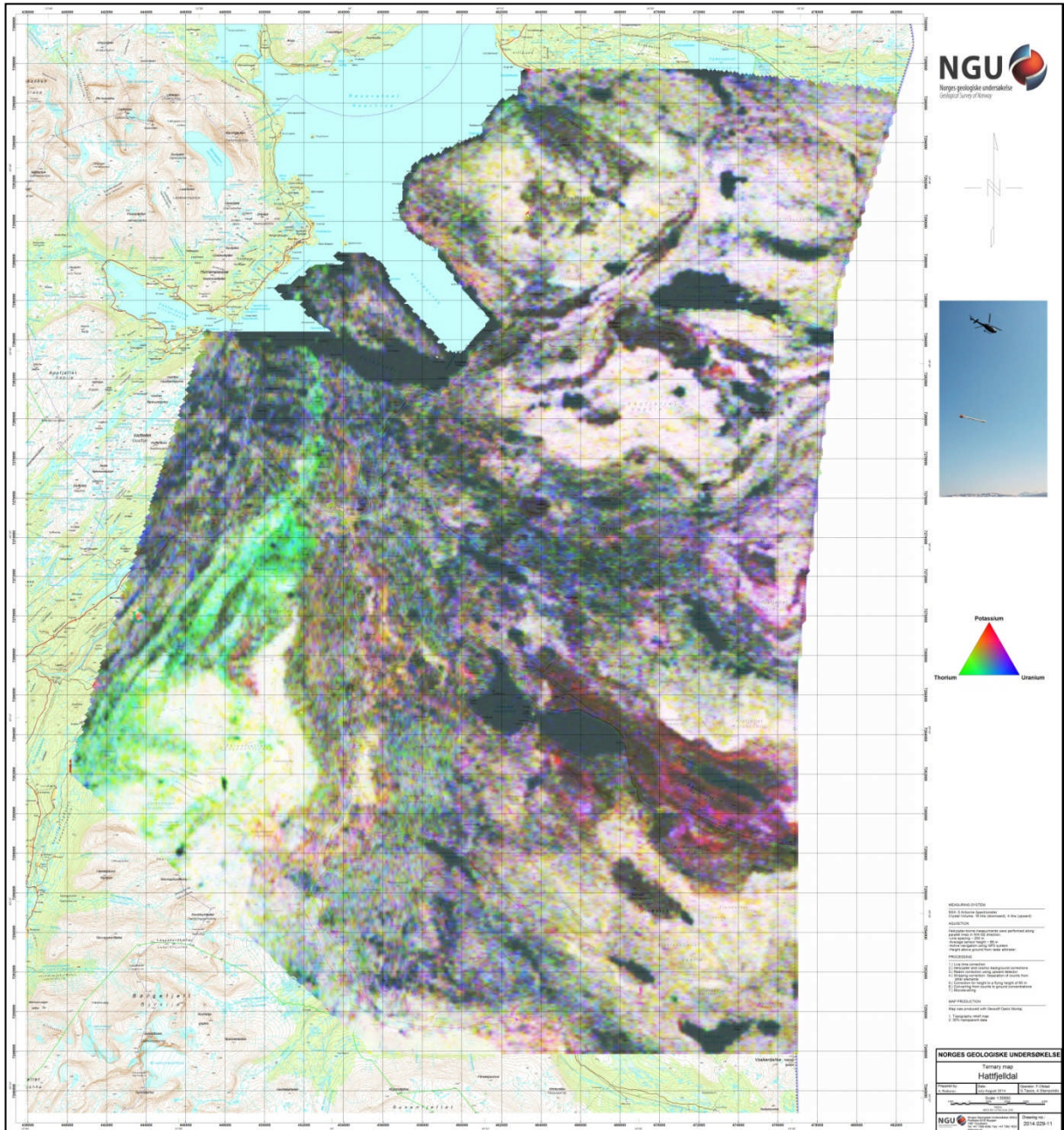
Figure 15: Radiometric Ternary map
