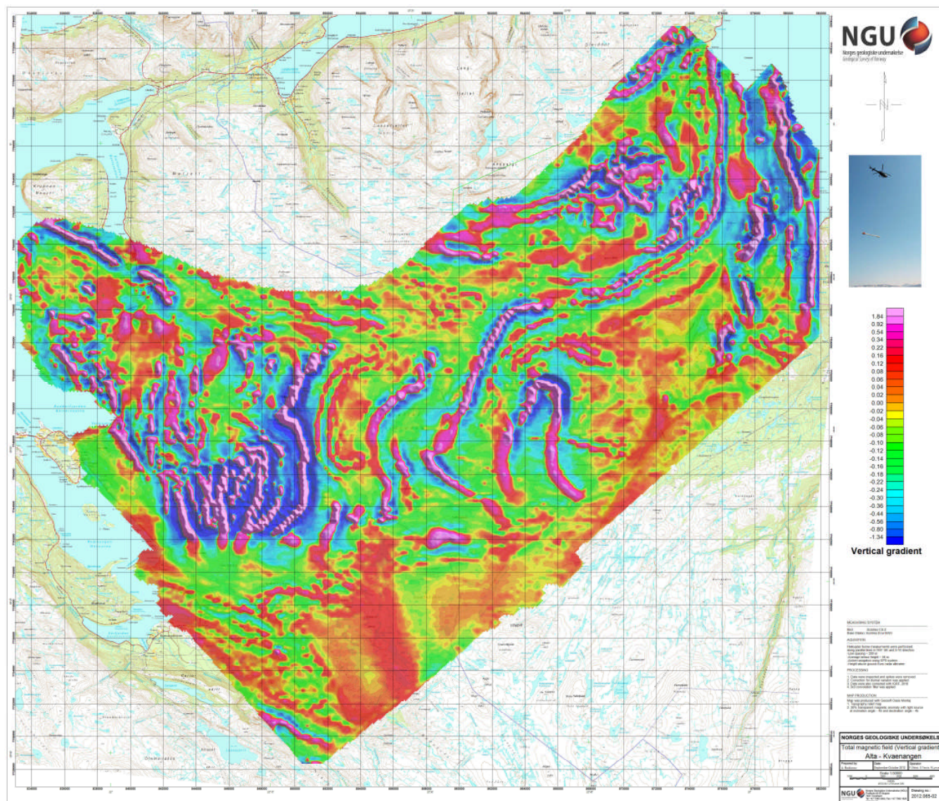
Figure 6: Total magnetic field. Vertical gradient.
