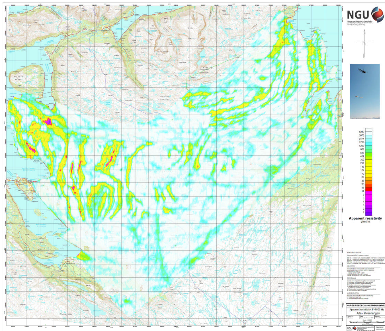
Figure 10: Apparent resistivity. Frequency 7000 Hz, Coaxial coils
