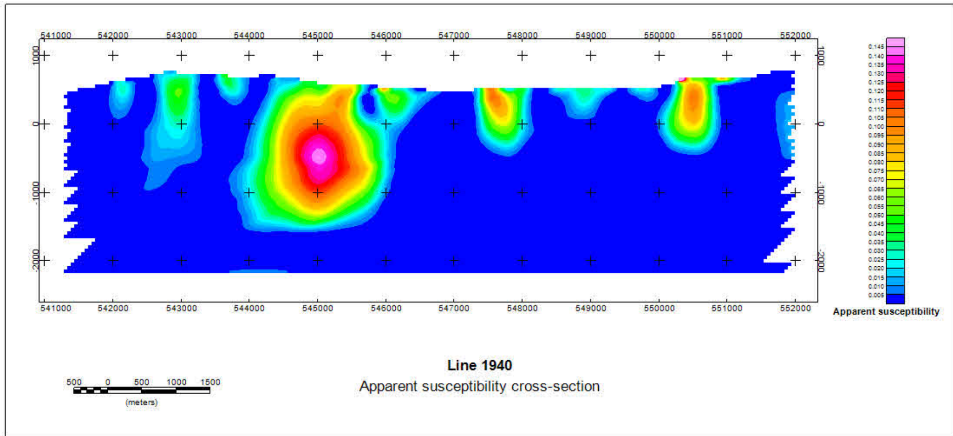
Figure 2: Apparent susceptibility cross-section, line 1940 (see Figure 4).
