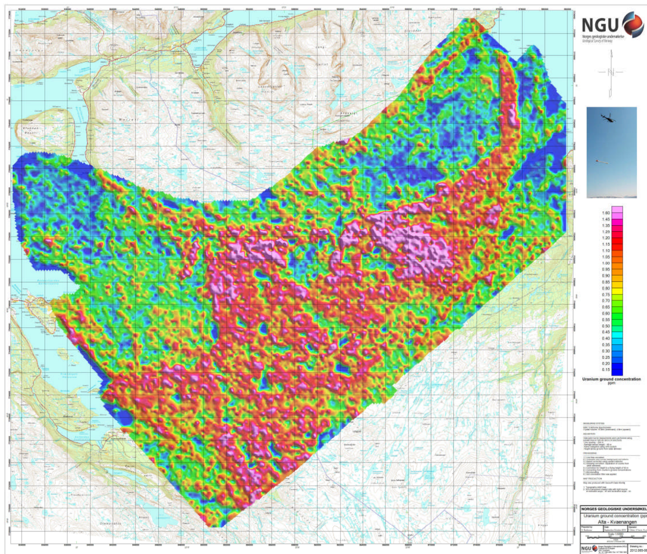
Figure 12: Uranium ground concentration
