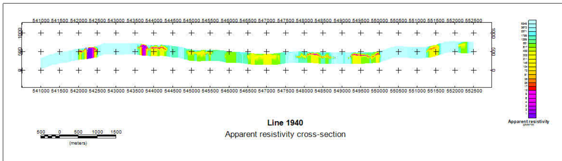
Figure 3: Apparent resistivity cross-section, line 1940 (see figure 4).
