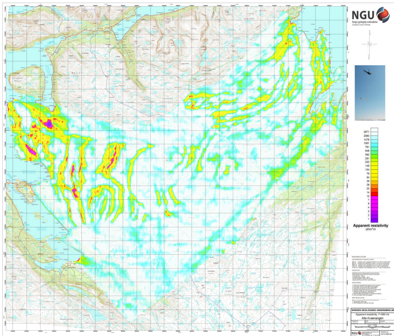
Figure 9: Apparent resistivity. Frequency 880 Hz, Coplanar coils
