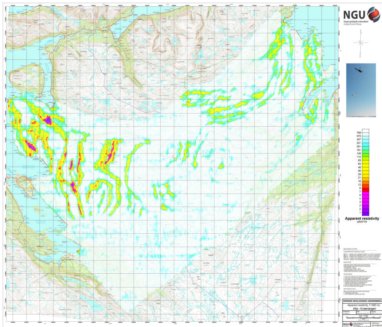
Figure 11: Apparent resistivity. Frequency 980 Hz, Coaxial coils
