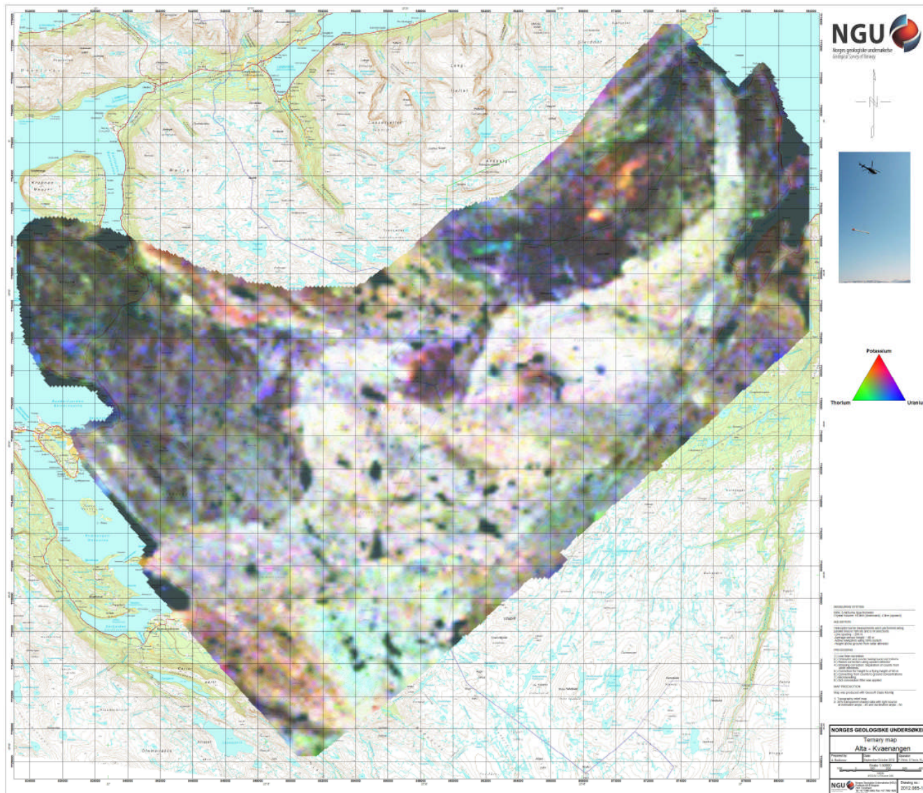
Figure 15: Radiometric ternary map
