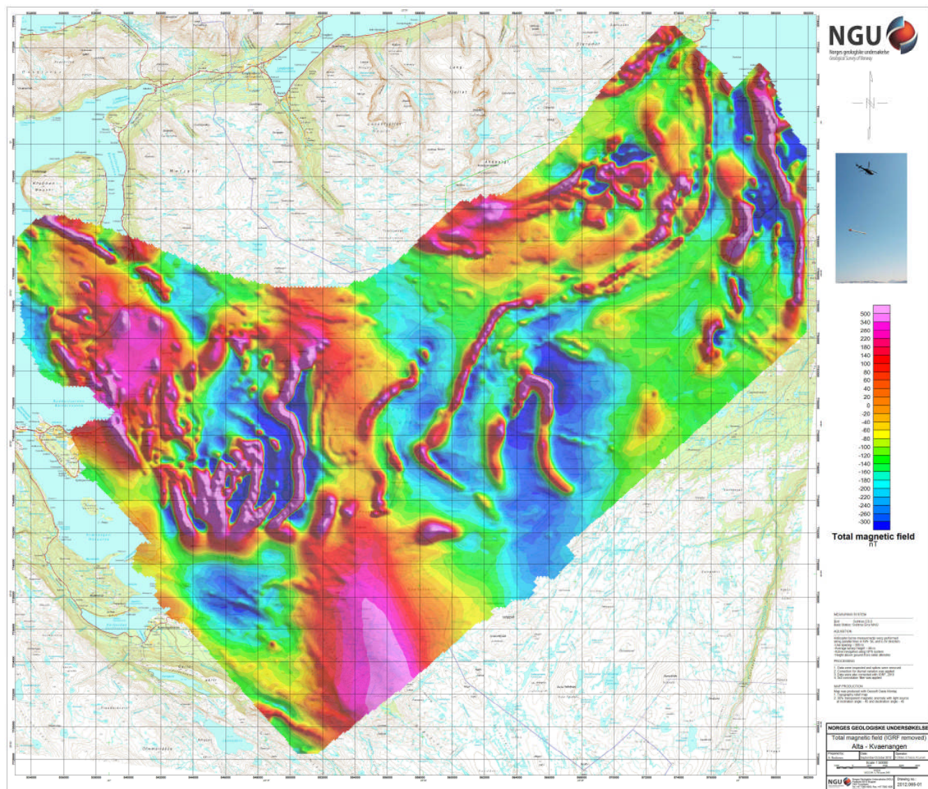
Figure 5: Total magnetic field
