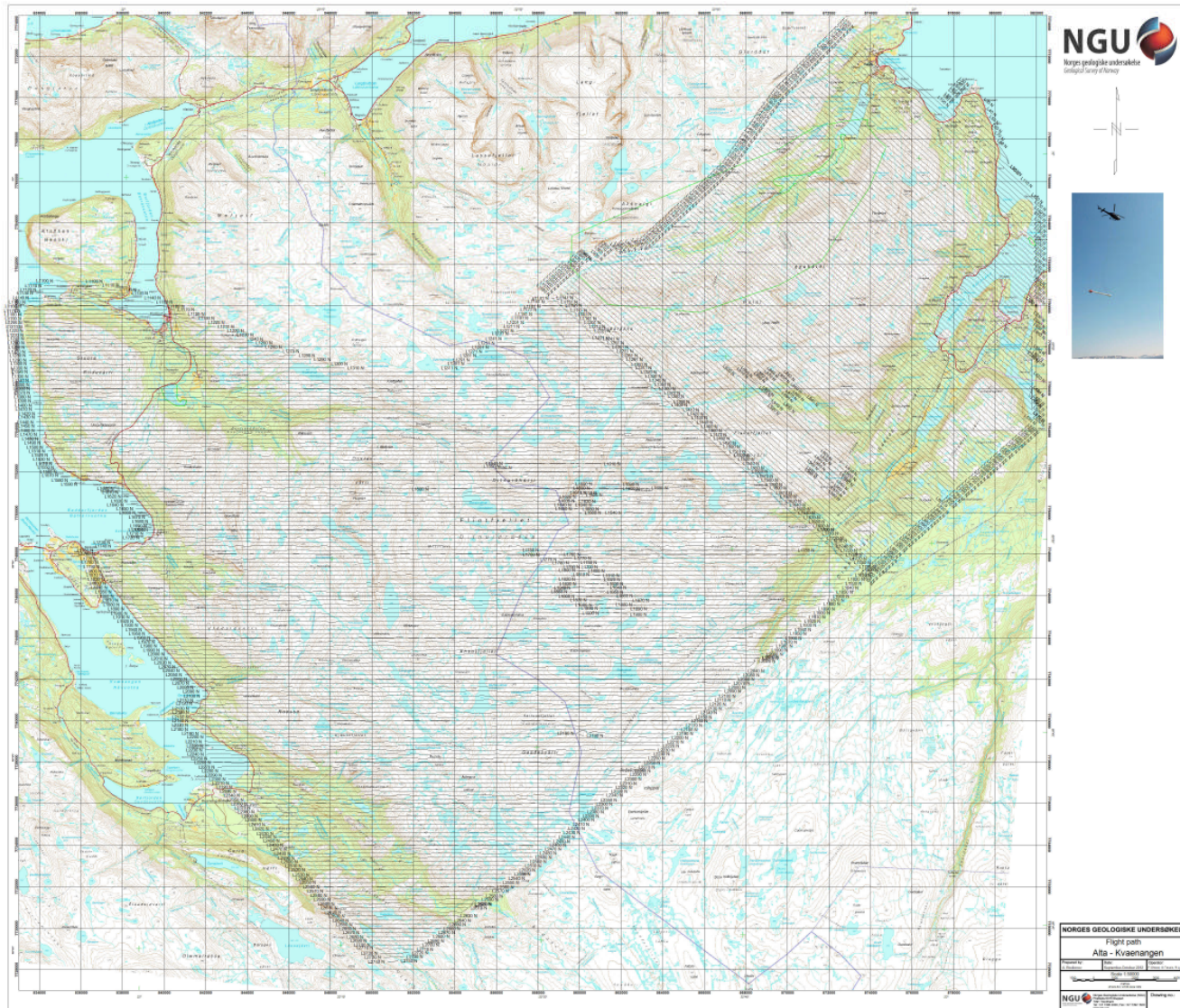
Figure 4: Kvænangen survey. Flight path.
