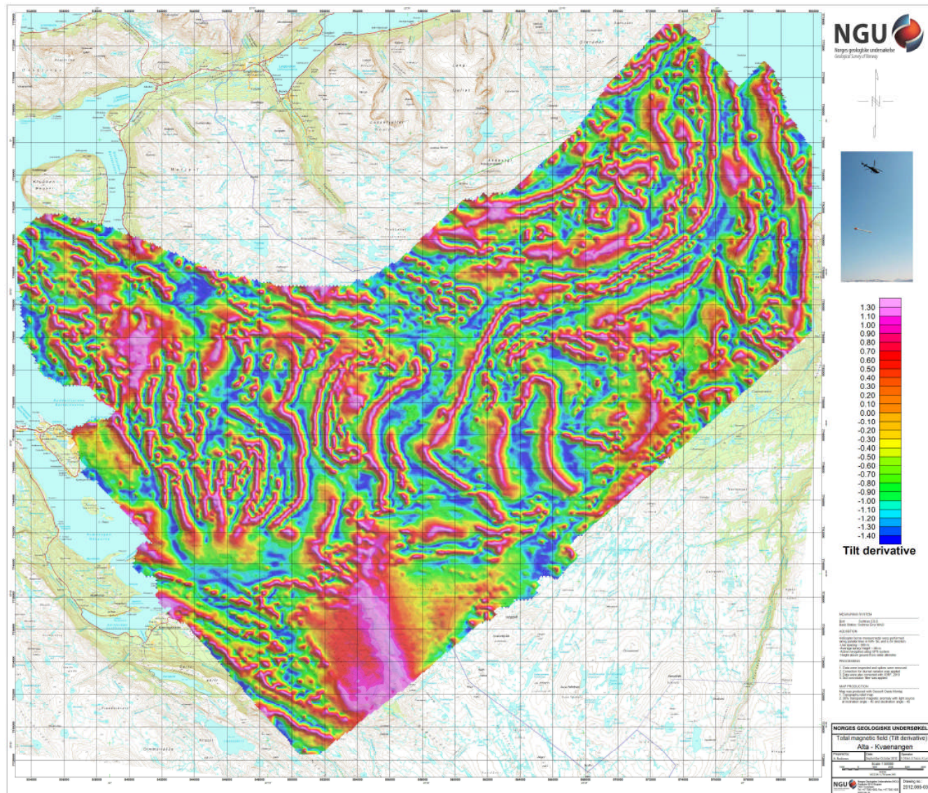
Figure 7: Total magnetic field. Tilt derivative.
