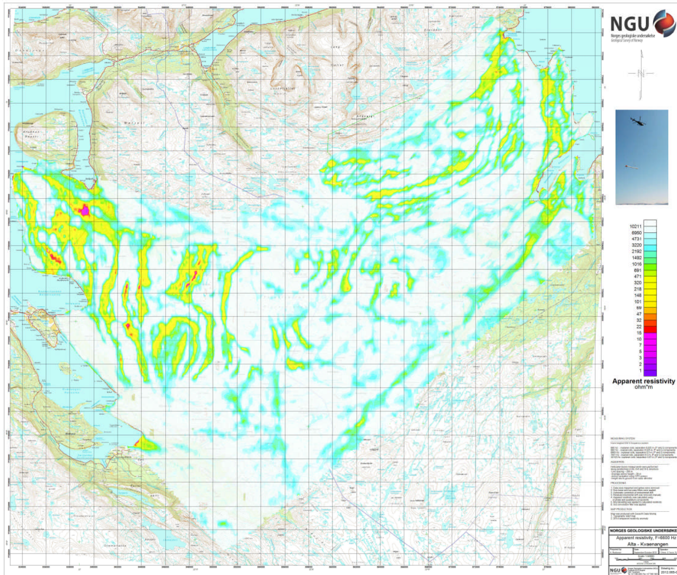
Figure 8: Apparent resistivity. Frequency 6600 Hz, Coplanar coils
