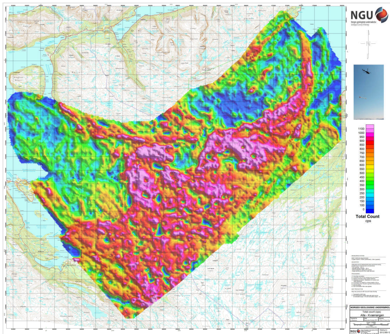
Figure 16: Radiometric total count.
