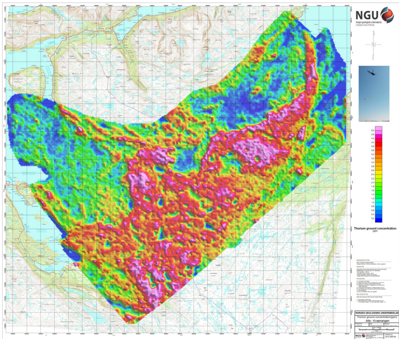
Figure 13: Thorium ground concentration
