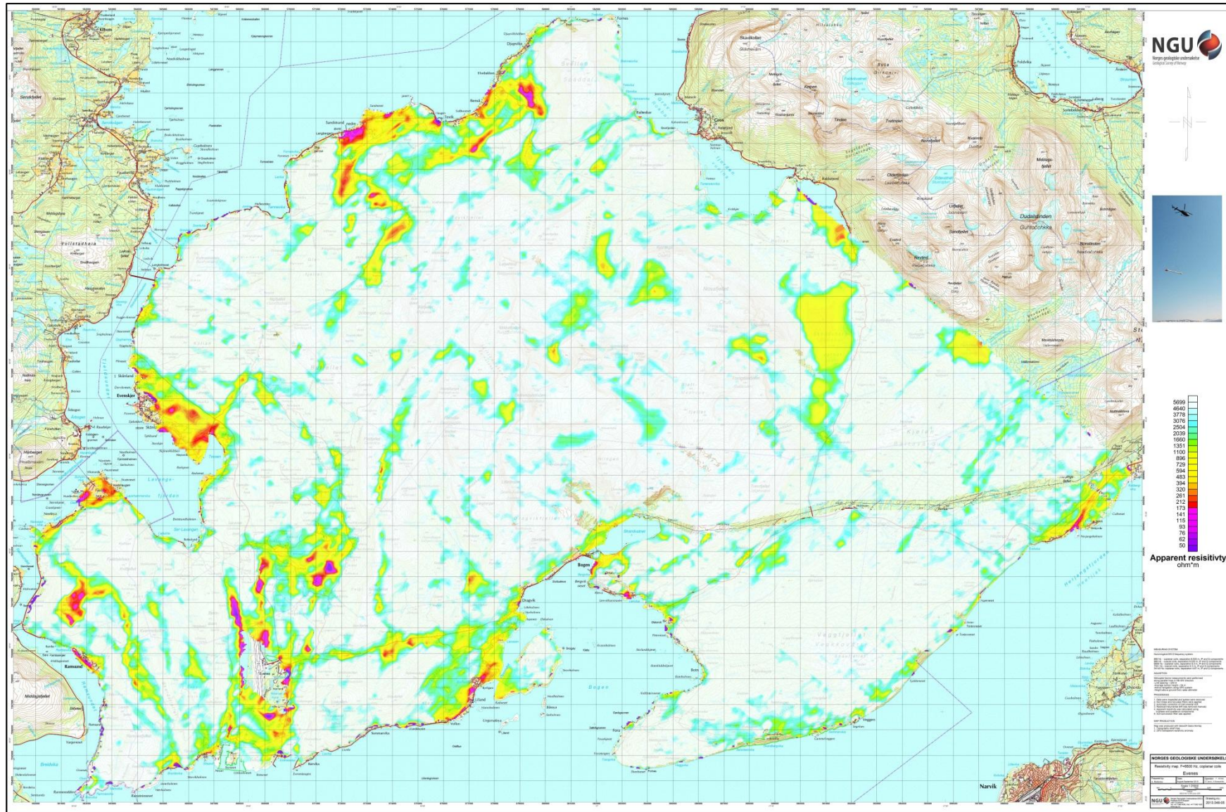
Figure 8: Apparent resistivity. Frequency 6600 Hz, Coplanar coils
