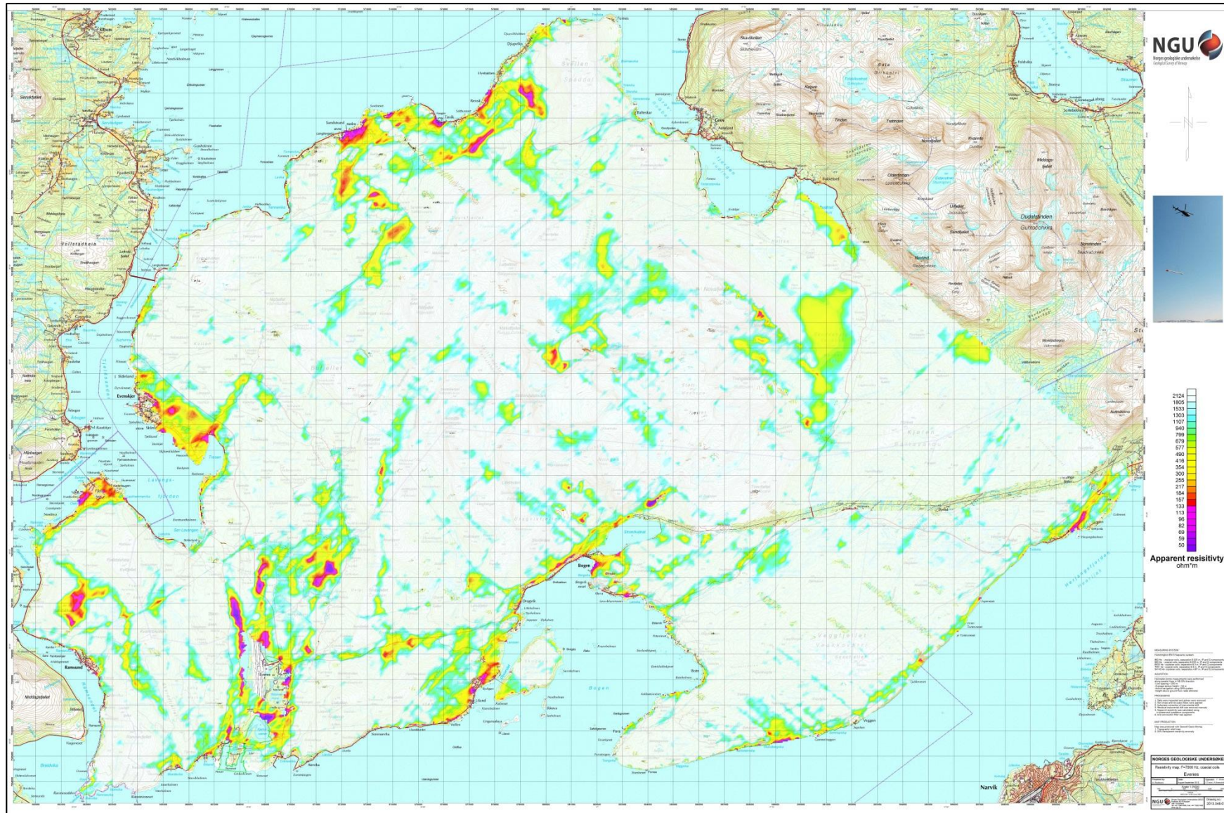
Figure 10: Apparent resistivity. Frequency 7000 Hz, Coaxial coils
