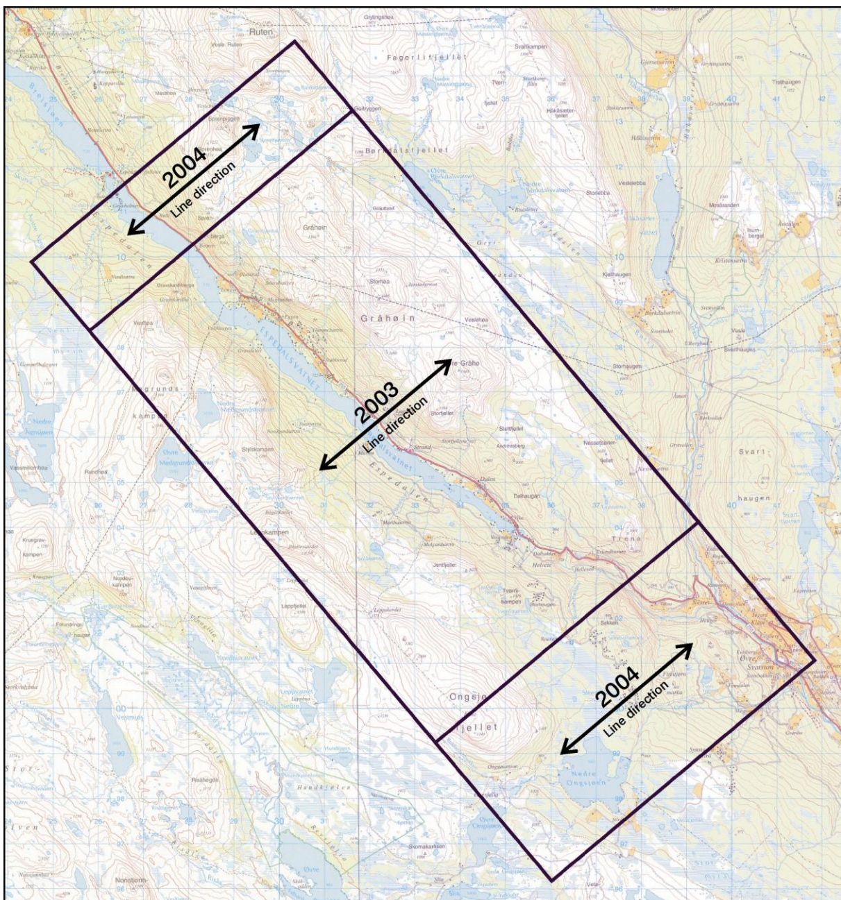
Fig. 1: Outline of the surveyed area (flight direction 050/230°)
