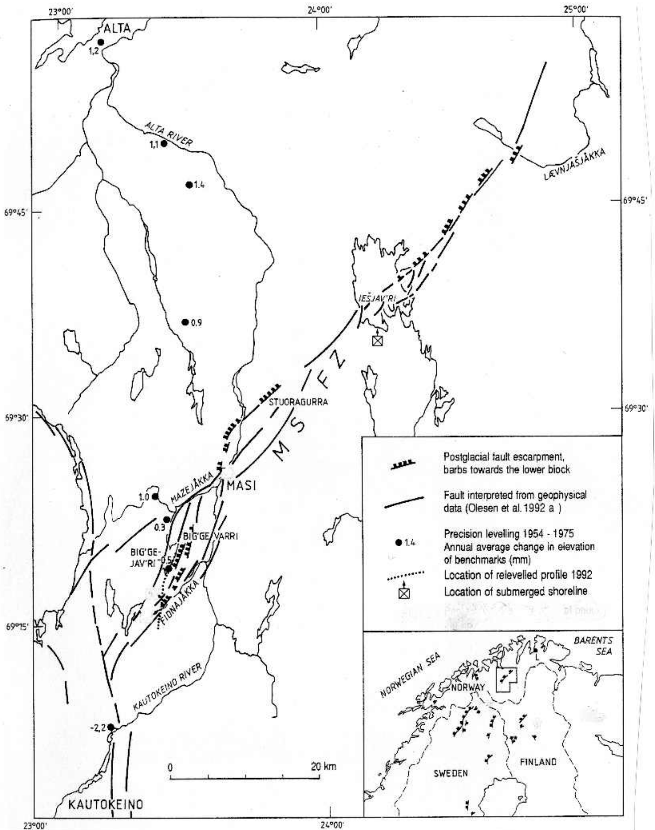
Figure 2. Postglacial faults on Finnmarksvidda. MSFZ — Mierujavri-Sværholt Fault Zone. The annual average change in elevation of benchmarks is based on precision levelling in 1954 and 1975 (Sørensen et al. 1987). Inset map shows Late Quaternary faults in northern Fennoscandia (Olesen 1991). L — offset drillhole locality southwest of Lebesby, Finnmark (Roberts 1991).
