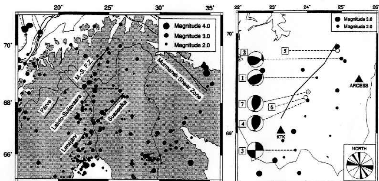
Figure 5. a) Earthquakes from 1979-1992 and postglacial faults (Bungum & Lindholm 1997). b) Focal mechanisms (Bungum & Lindholm 1997) calculated for five earthquakes and earthquakes from 1979-1992 along the Stuoragurra postglacial fault. The trend of horizontal compression as indicated by the fault plane solutions is seen in the rose diagram in the lower-right corner. Earthquake No. 7 represents the magnitude 4.0 earthquake on 21 January 1996.
