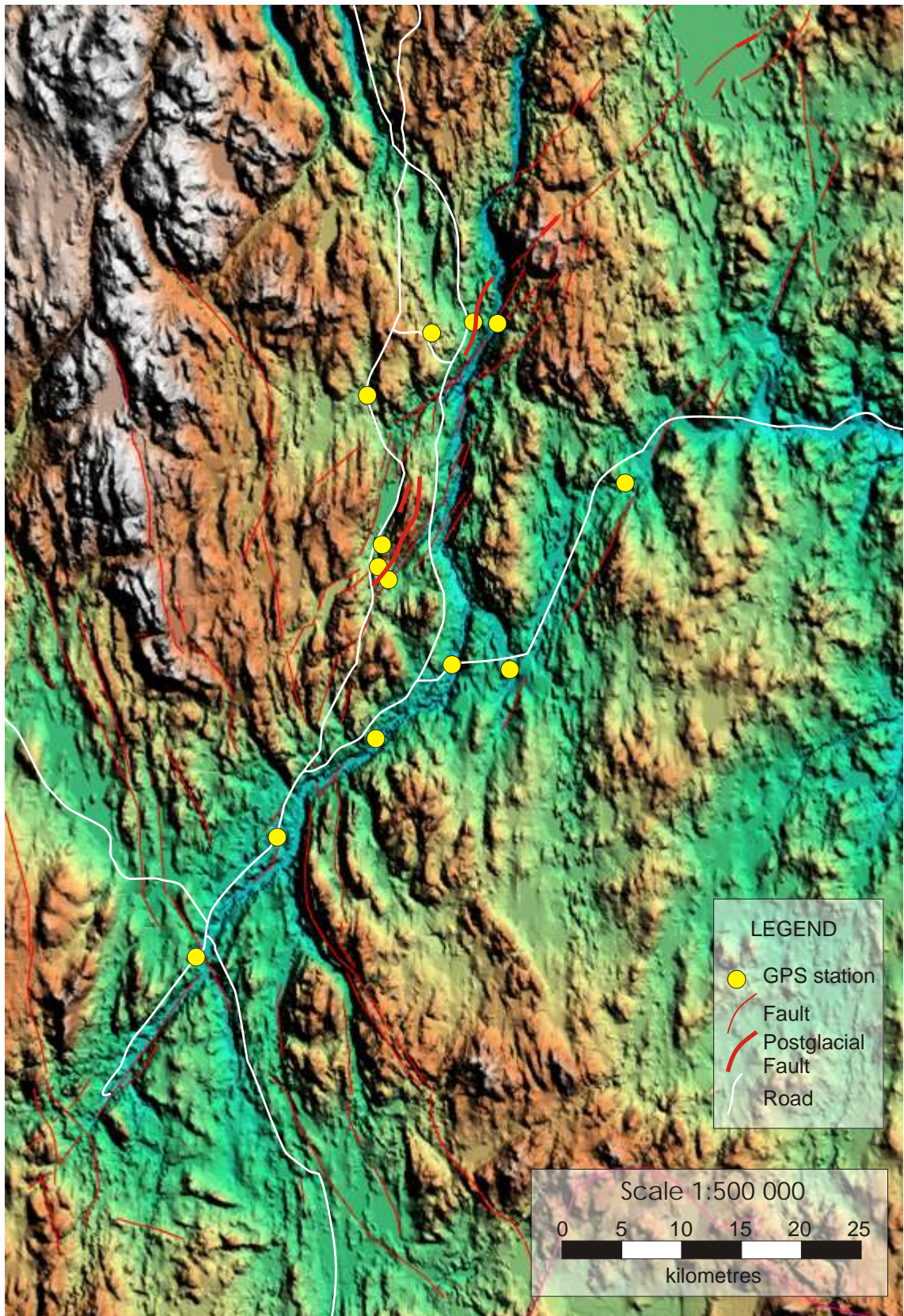
Figure 27. Locations of the GPS stations setup around the Stuaragurra postglacial fault during the summer of 1997.
