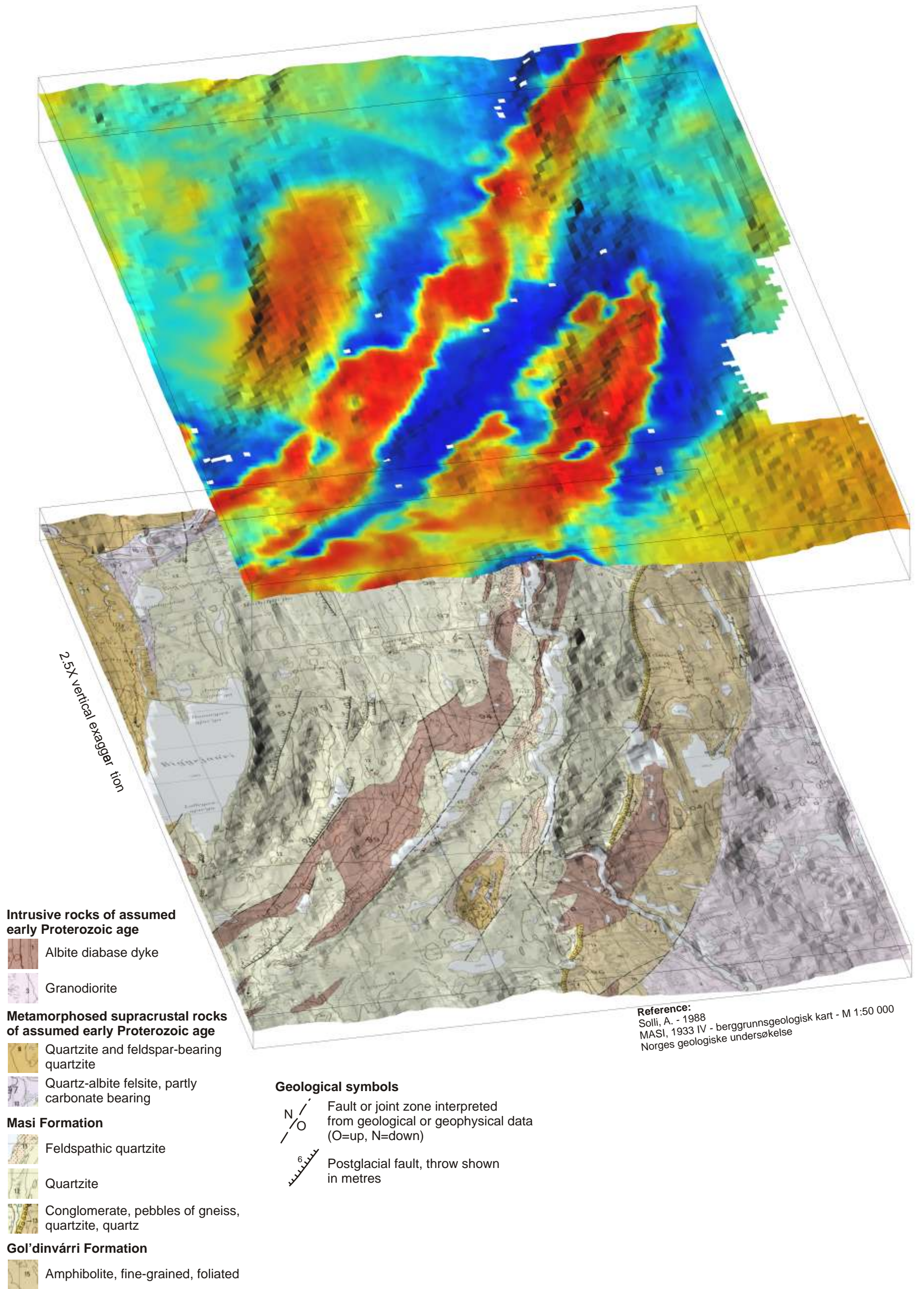
Figure 3. Aeromagnetic map (Olesen and Sandstad 1993) and bedrock geology map (Solli, 1988) from the Skarrevjavre-Biggearri area. Magnetic albite diabases occur along the regional Mierujavri-Sværholt Fault Zone. Postglacial faults are reactivated along this fault zone.
