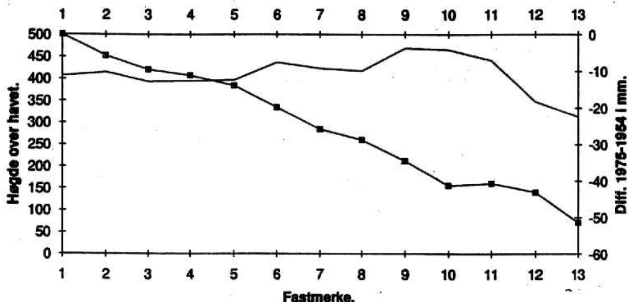
Fig. 24. Difference in elevation (filled squares) along relevelled profile in 1975 relative to levelling in 1954 (Skjøthaug, pers. comm., 1992; Olesen et al., 1992c). The profile is located along the old road between Masijåkka and Mierujavri (Mieron). The uplift decreases to the south, which is opposite to the regional trend.
