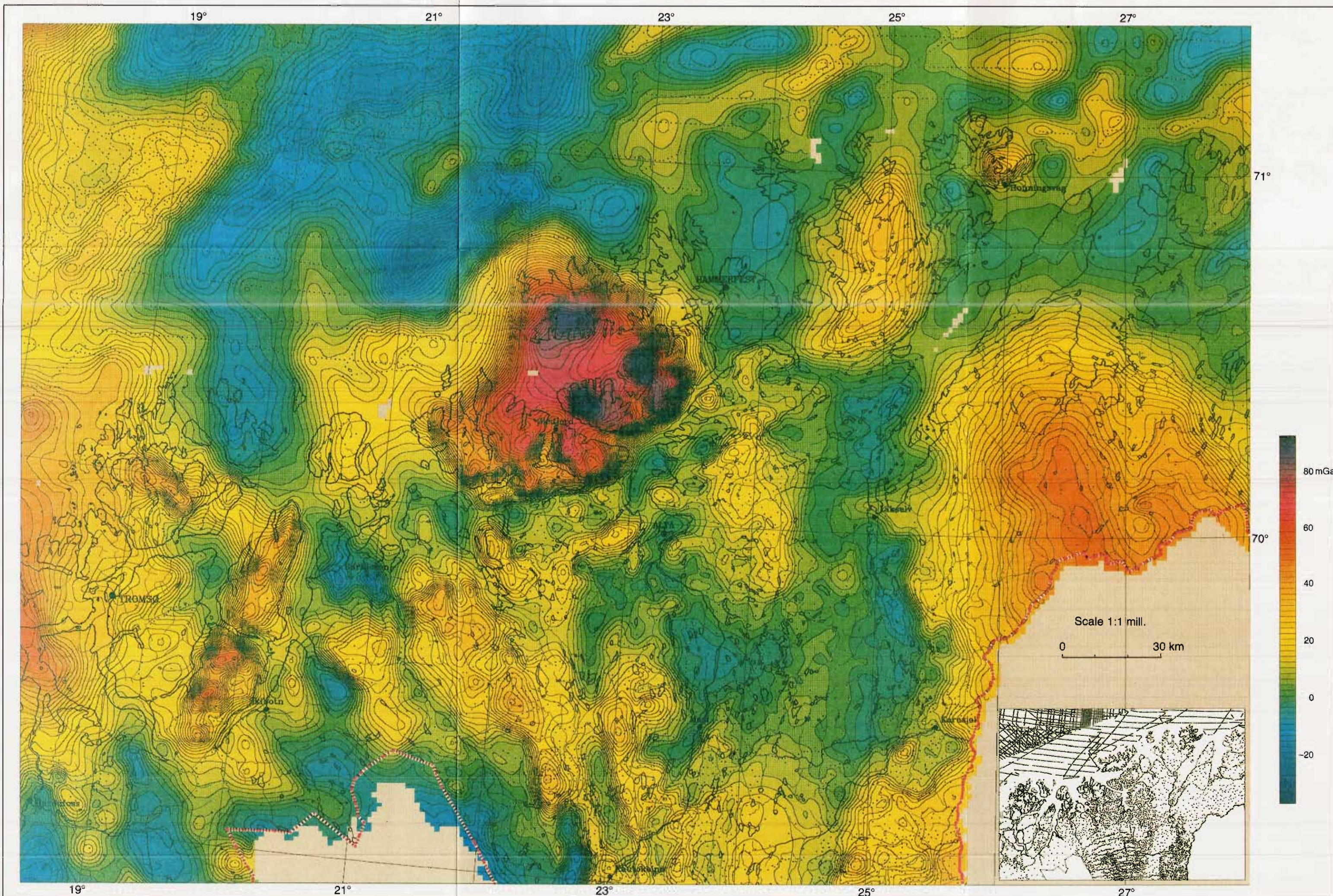
Plate 3: Residual gravity map of western Finnmark and northern Troms. 1500 x 1500 m grid cells interpolated from the Bouguer gravity data-set (G.S.N.71) using the minimum curvature method. Regional gravity field subtracted. Distribution of the original observation sites shown in index map.
