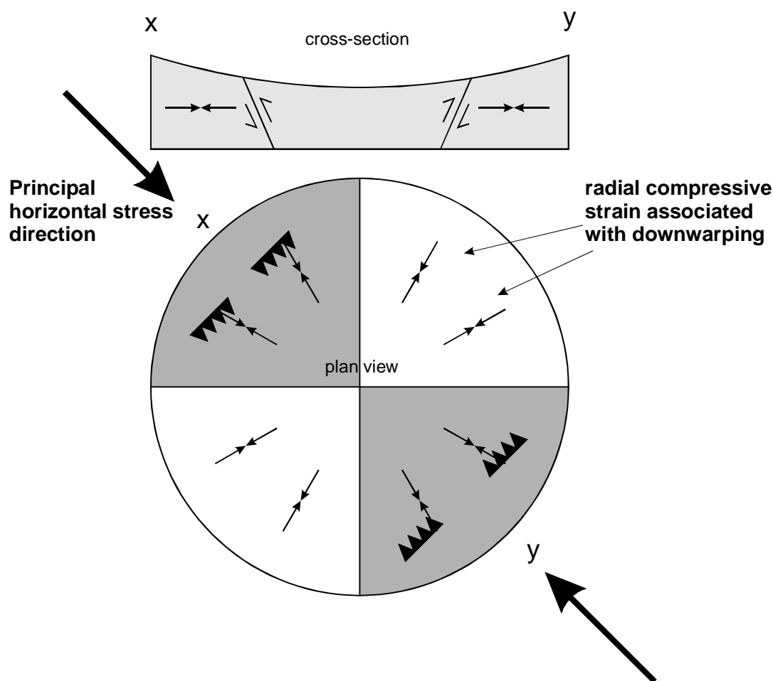
Figure 1. Model for the concentration of major strain release immediately following rapid glacial unloading proposed by Muir Wood (1993). Assuming a circular ice-cap located on a flat laterally homogenous crust, the flanks of the downwarped crust will have suffered a radial increase in stress during glacial loading. On the flanks of the downwarped bowl facing the principal horizontal stress direction (ridge-push stress oriented NW-SE in Scandinavia), radial strain raises \sigma_1 during downwarping, and on glacial unloading this will cause postglacial faulting. This model will explain the reverse faults within the Lapland Province, but not the normal faults. The model would also imply postglacial faulting to the southeast of the rebound dome in Finland where postglacial faults have not been observed.
