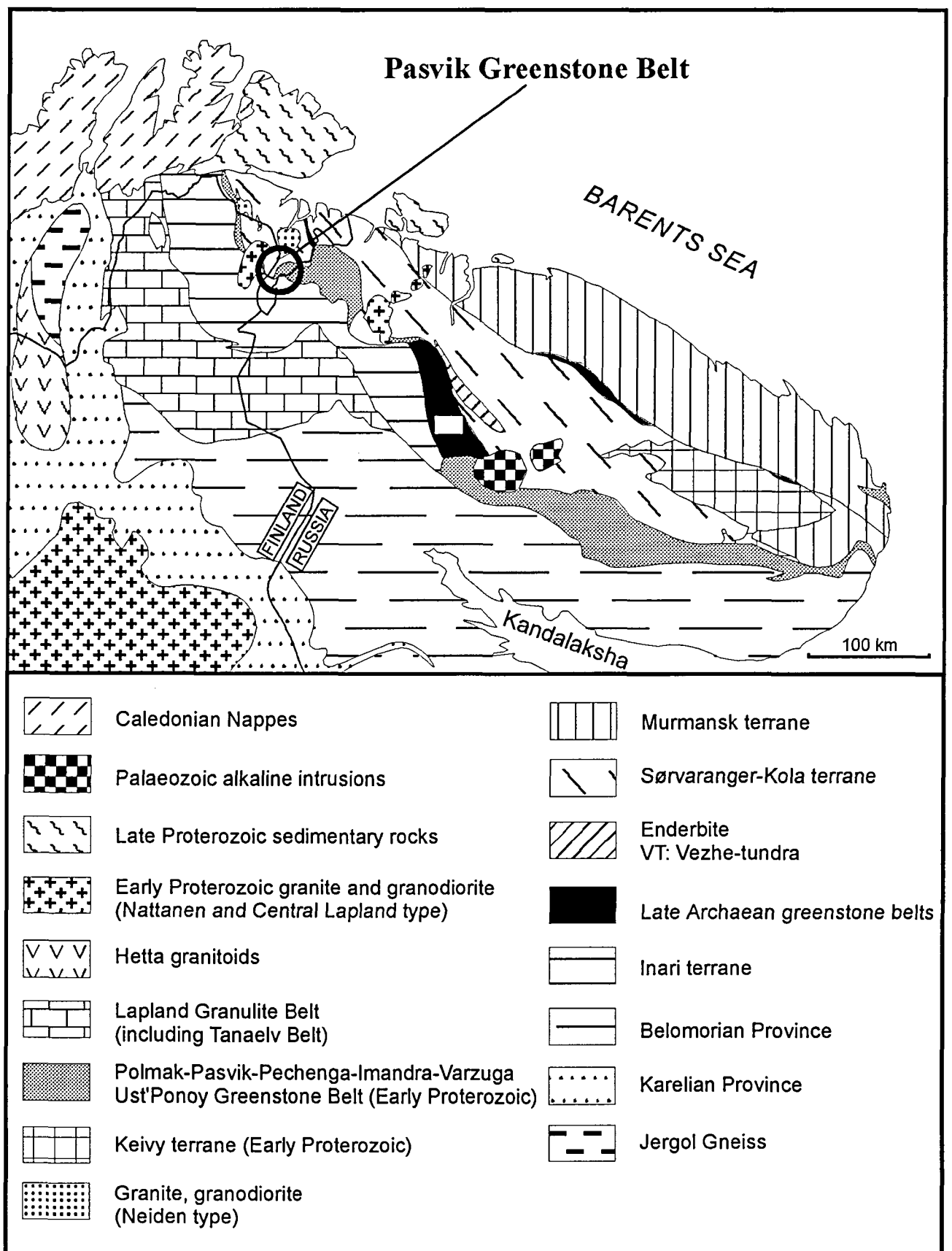
Fig. 2. Location of the Early Proterozoic Pasvik Greenstone Belt
