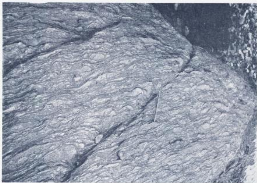
Fig. 9. The Steinkjer conglomerate at Tiltnes.
