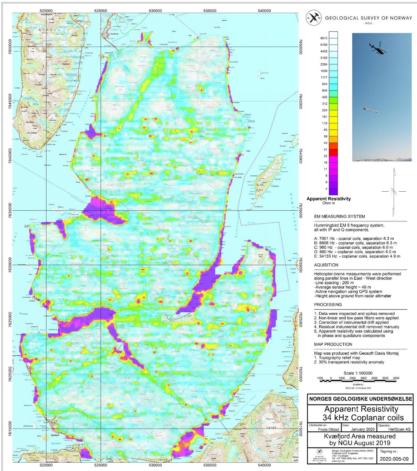
Figure 13 Apparent resistivity. Frequency 34133 Hz, Coplanar coils
