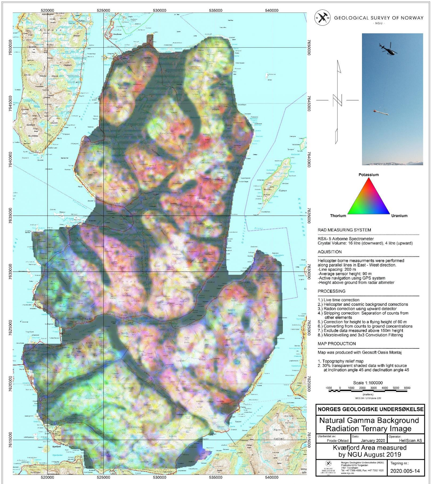
Figure 18: Radiometric Ternary Image
