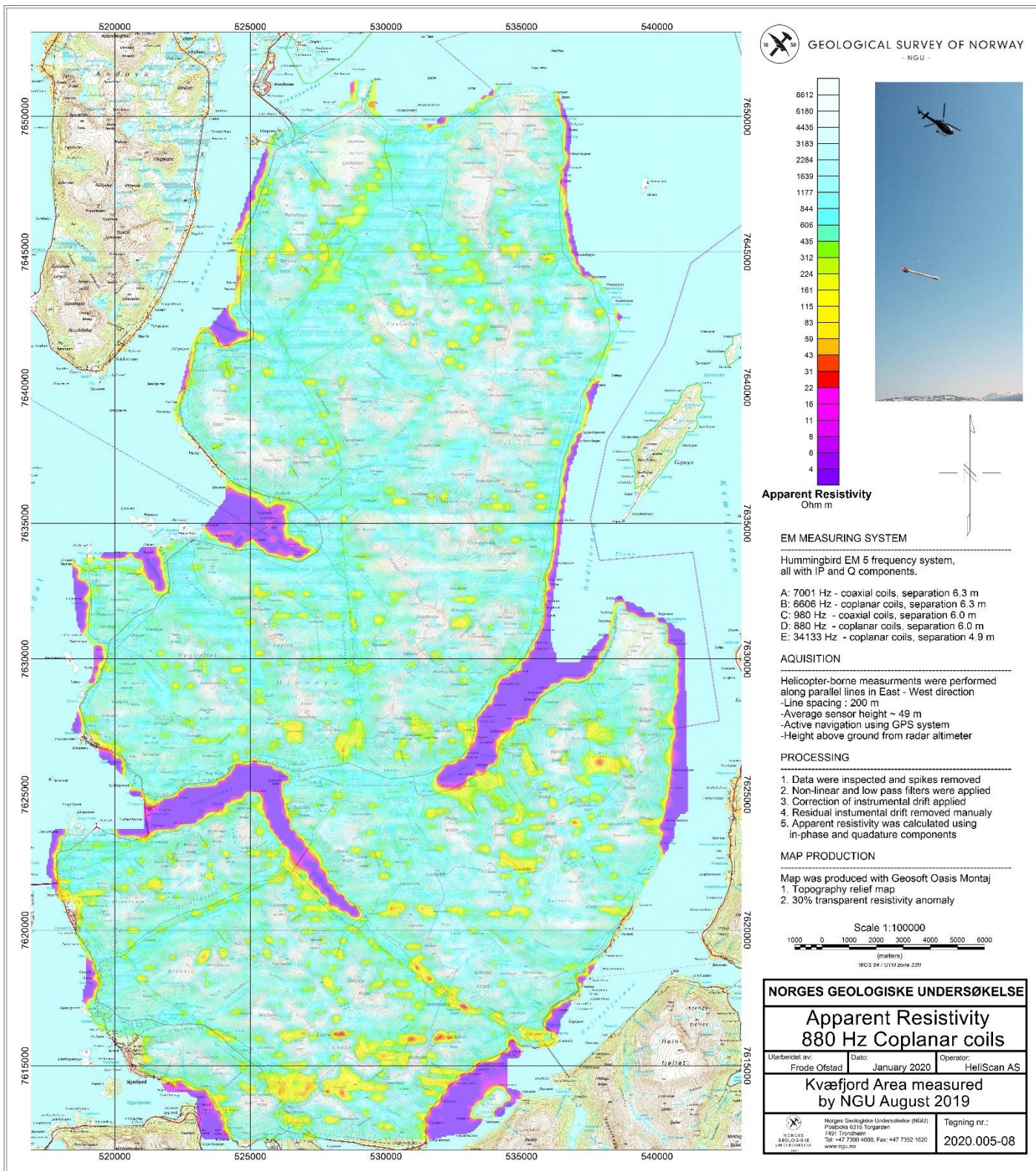
Figure 12: Apparent resistivity. Frequency 880 Hz, Coplanar coils
