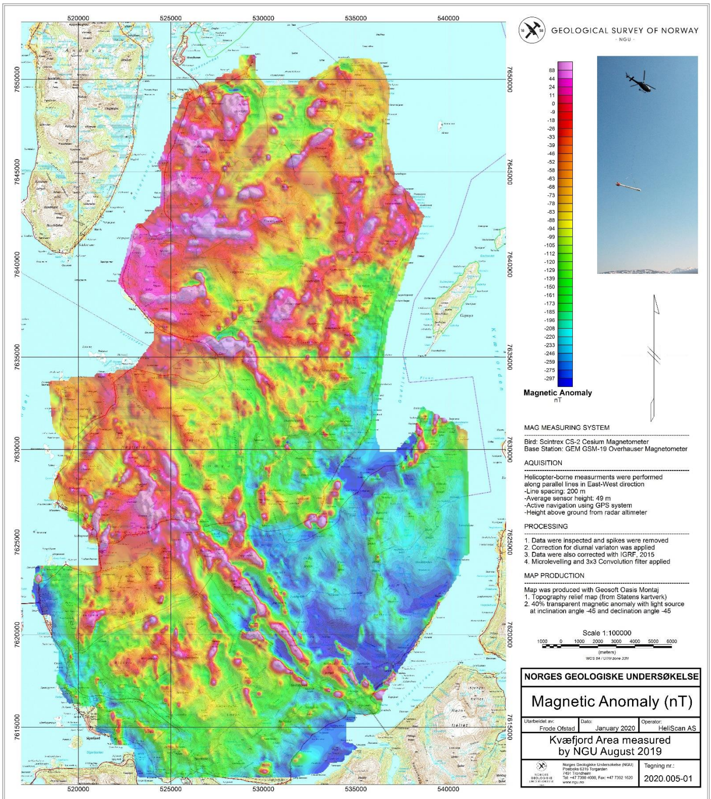
Figure 5: Total Magnetic Field
