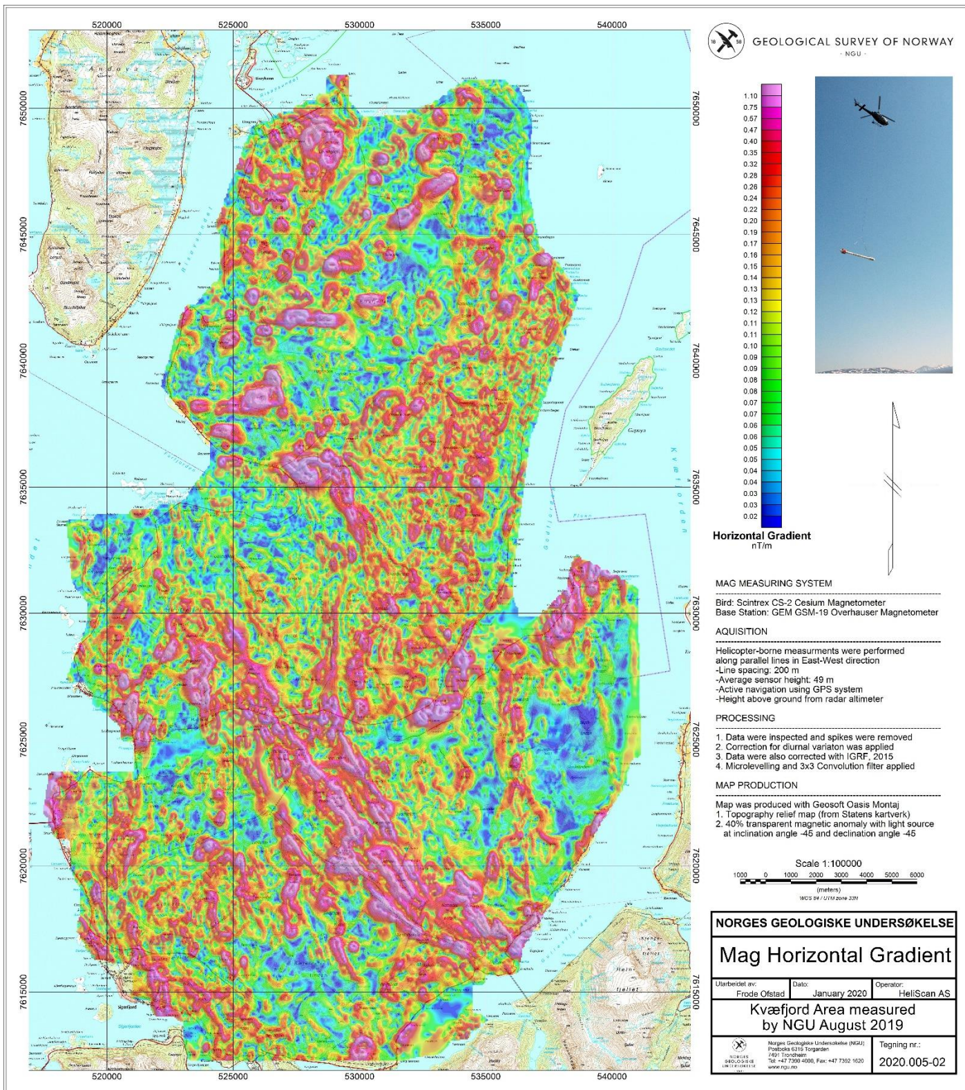
Figure 6: Magnetic Horizontal Gradient
