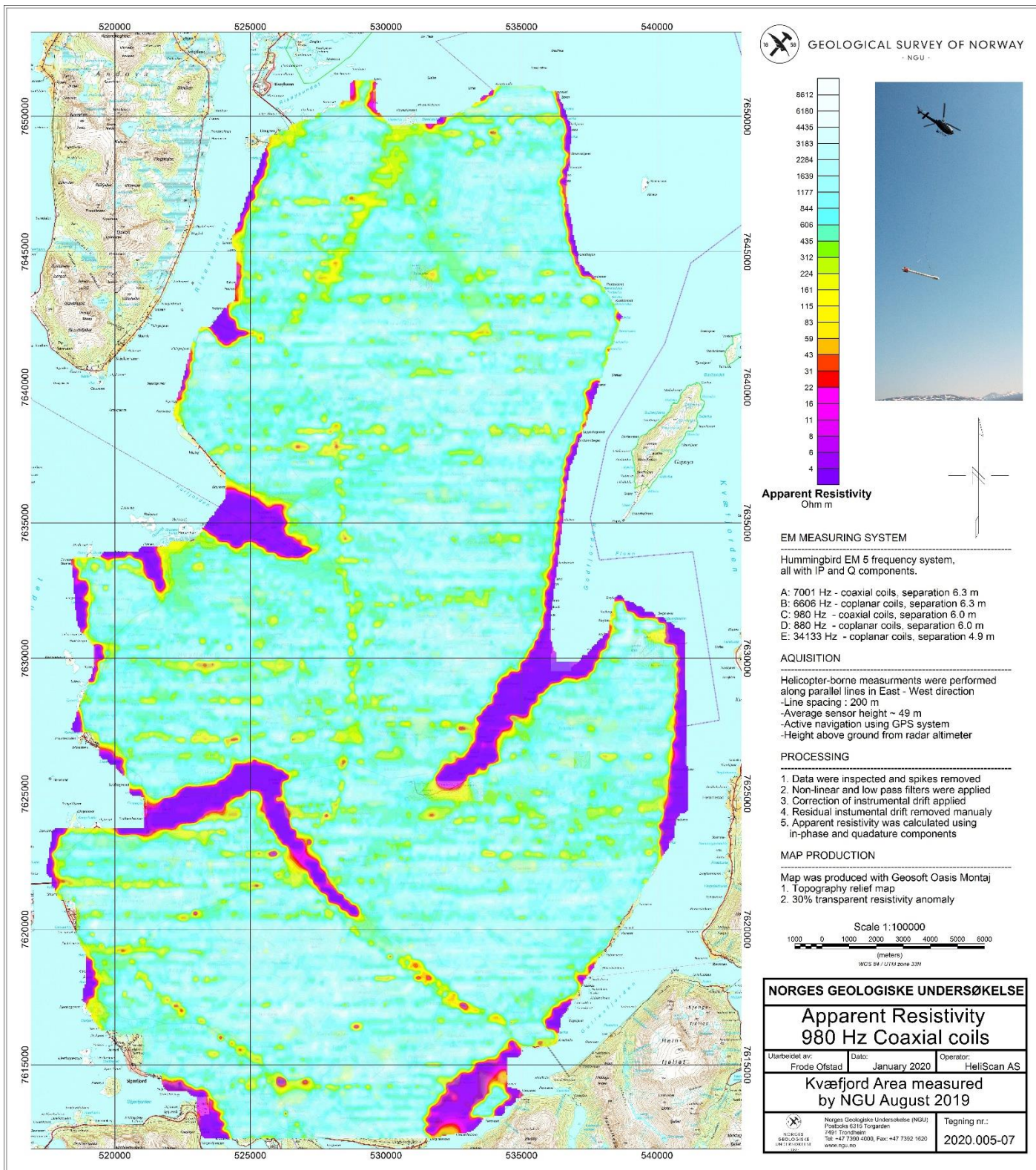
Figure 11: Apparent resistivity. Frequency 980 Hz, Coaxial coils
