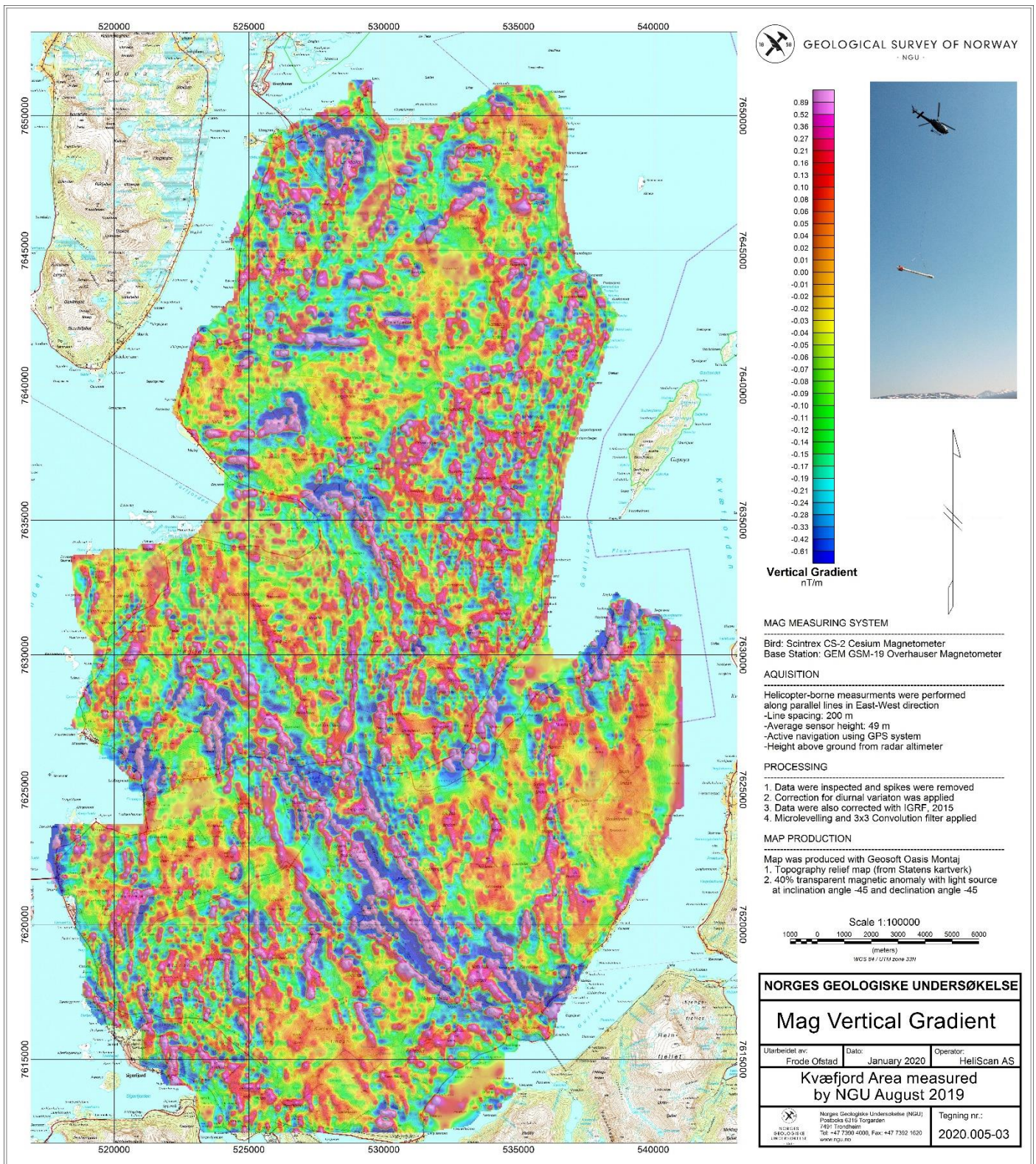
Figure 7: Magnetic Vertical Derivative
