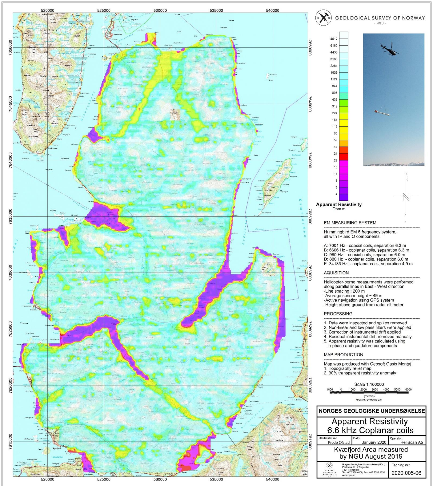
Figure 10: Apparent resistivity. Frequency 6600 Hz, Coplanar coils
