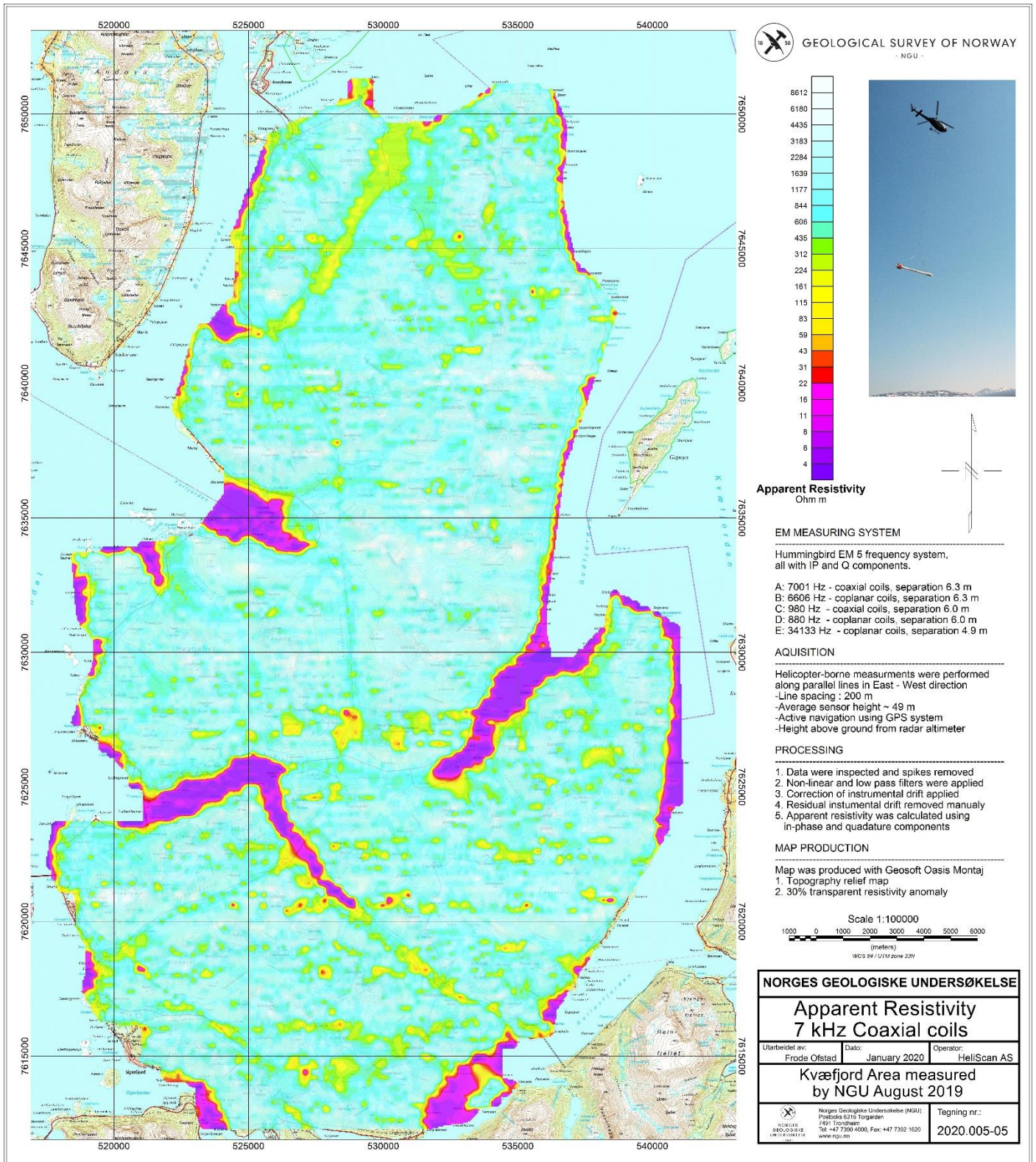
Figure 9: Apparent resistivity. Frequency 7000 Hz, Coaxial coils
