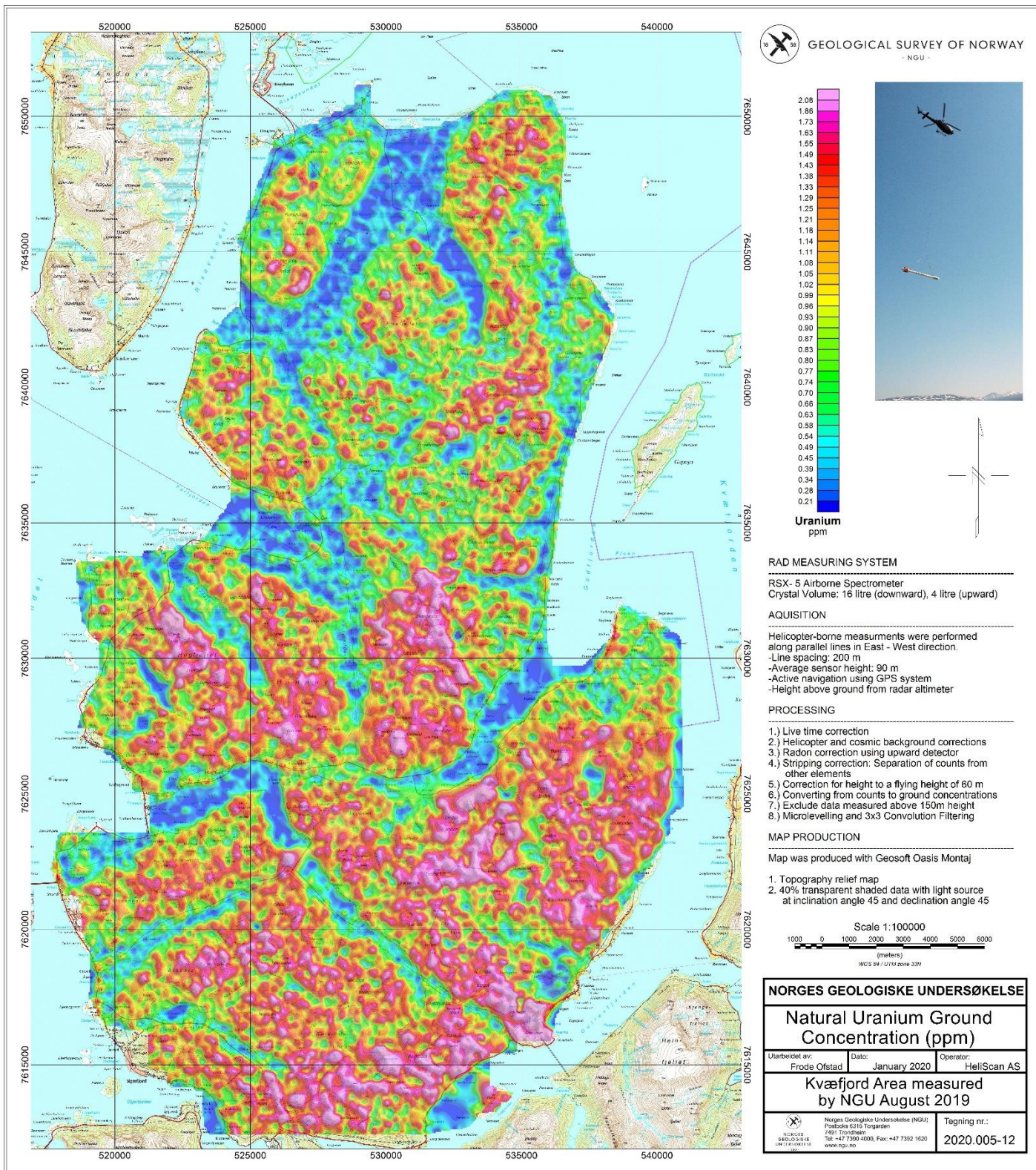
Figure 16: Uranium ground concentration
