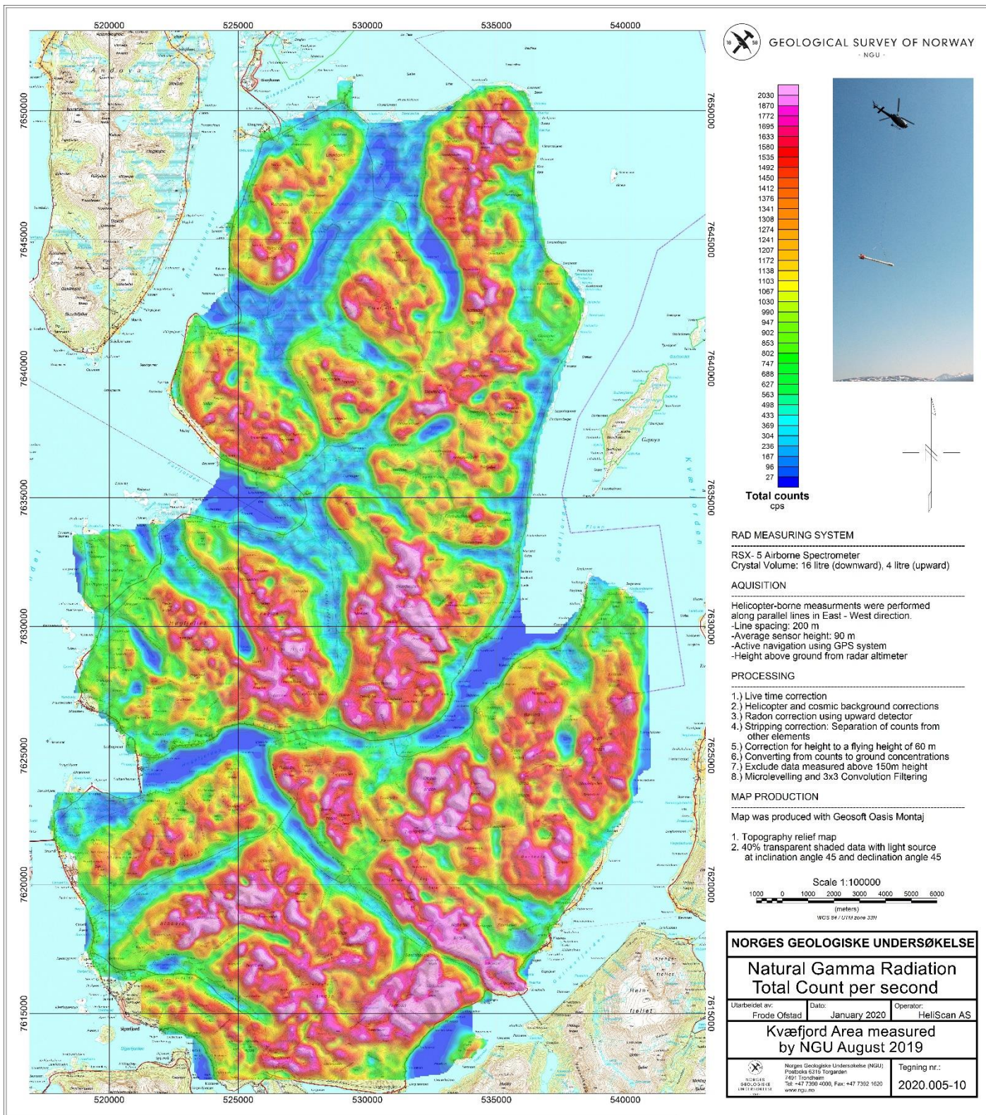
Figure 14: Radiometric Total counts
