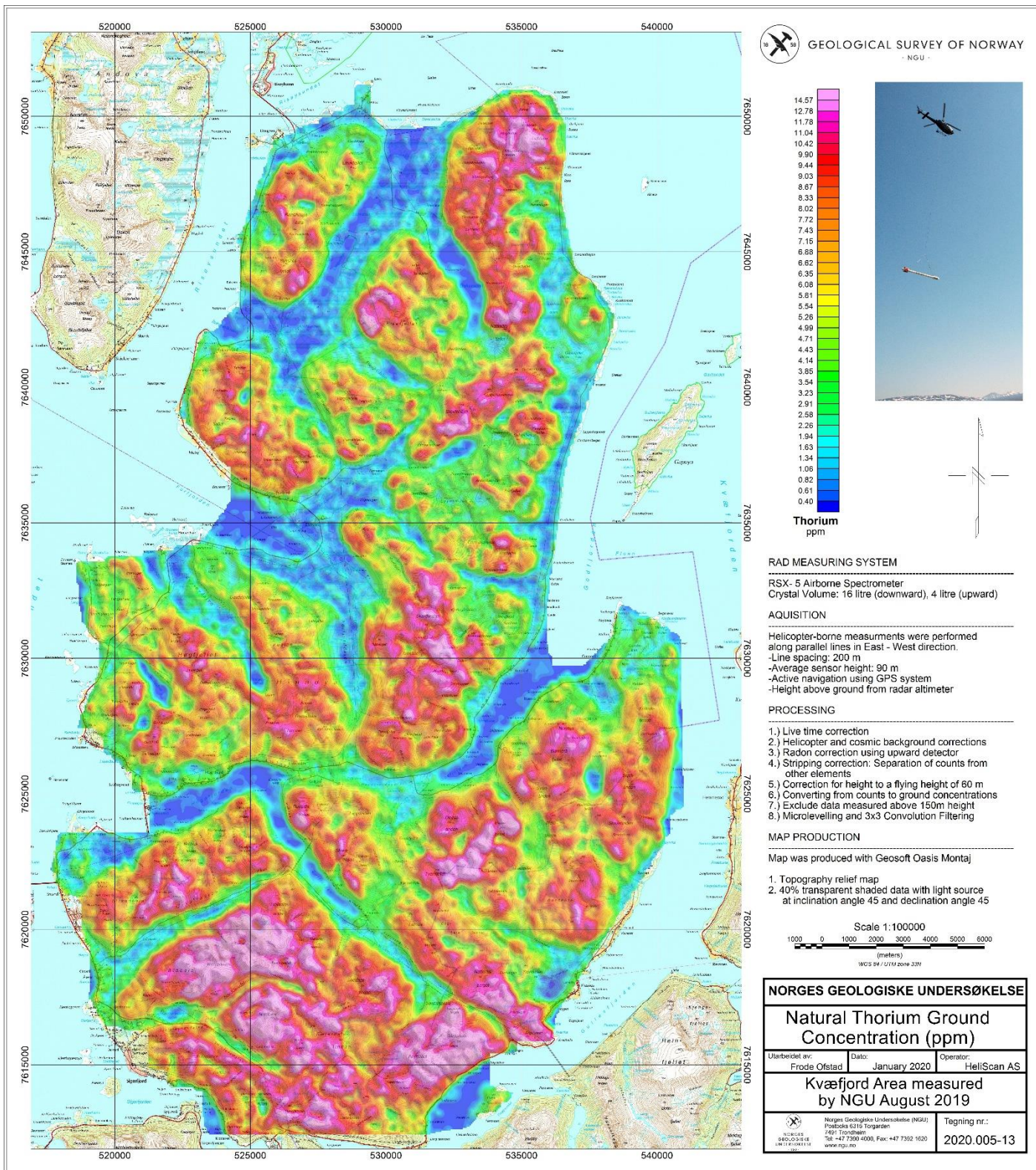
Figure 17: Thorium ground concentration
