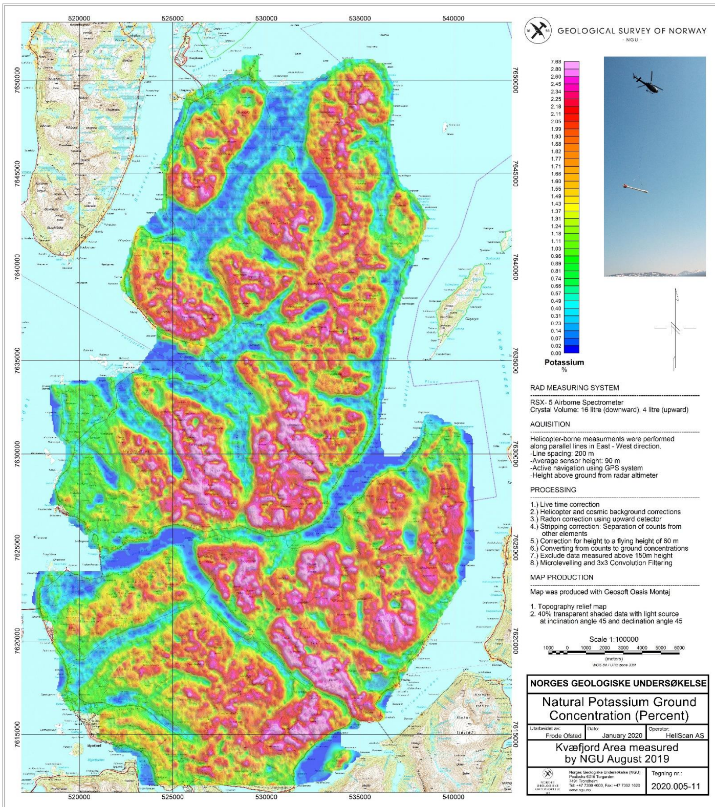
Figure 15: Potassium ground concentration
