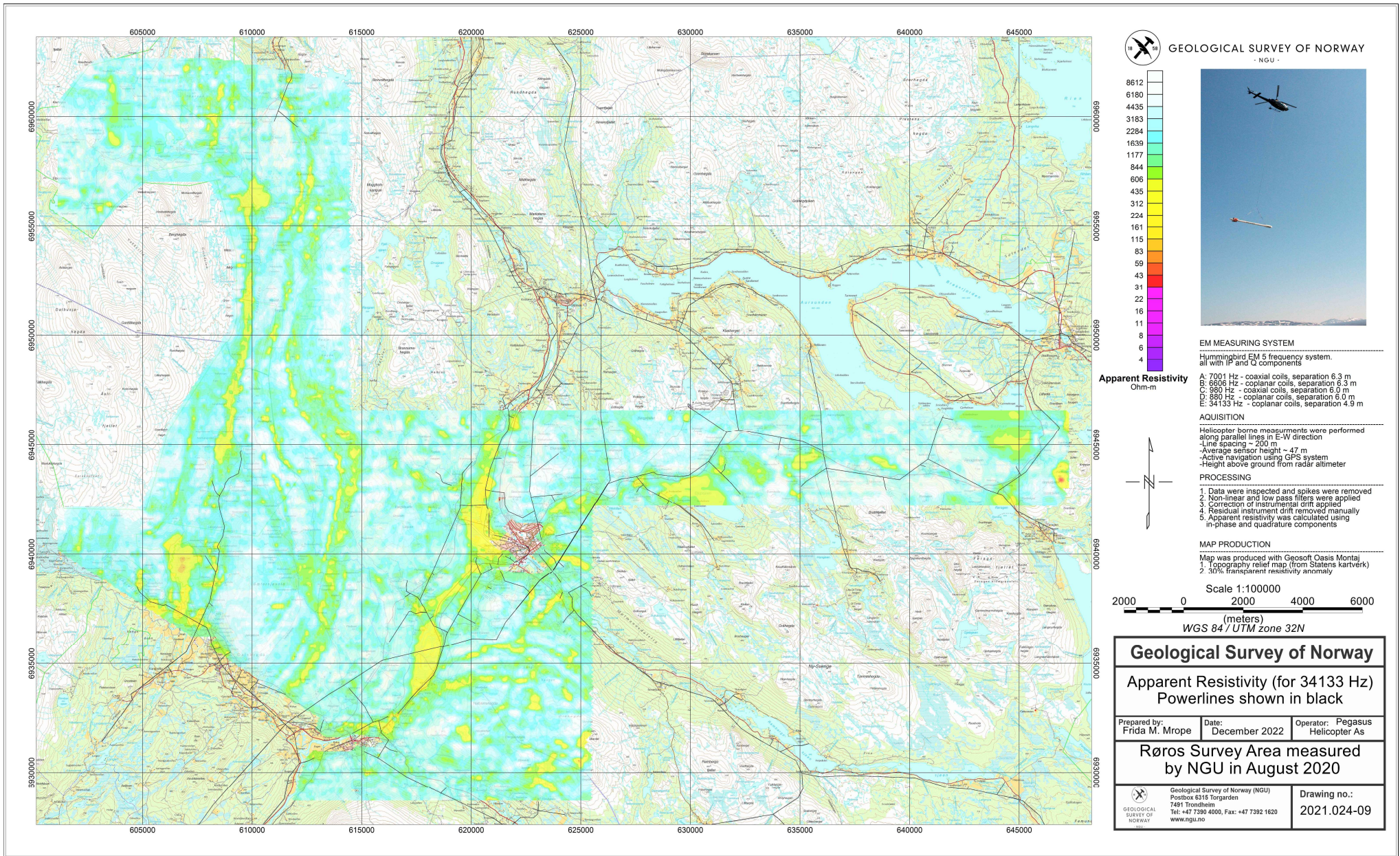
Figure 13 Apparent resistivity. Frequency 34133 Hz, Coplanar coils.
