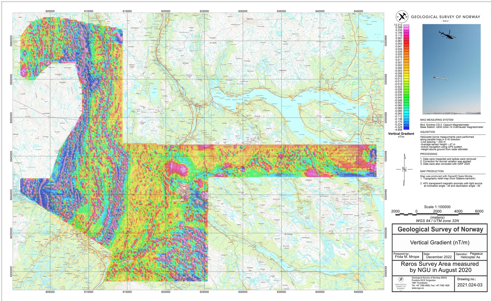
Figure 7: Magnetic Vertical Derivative.
