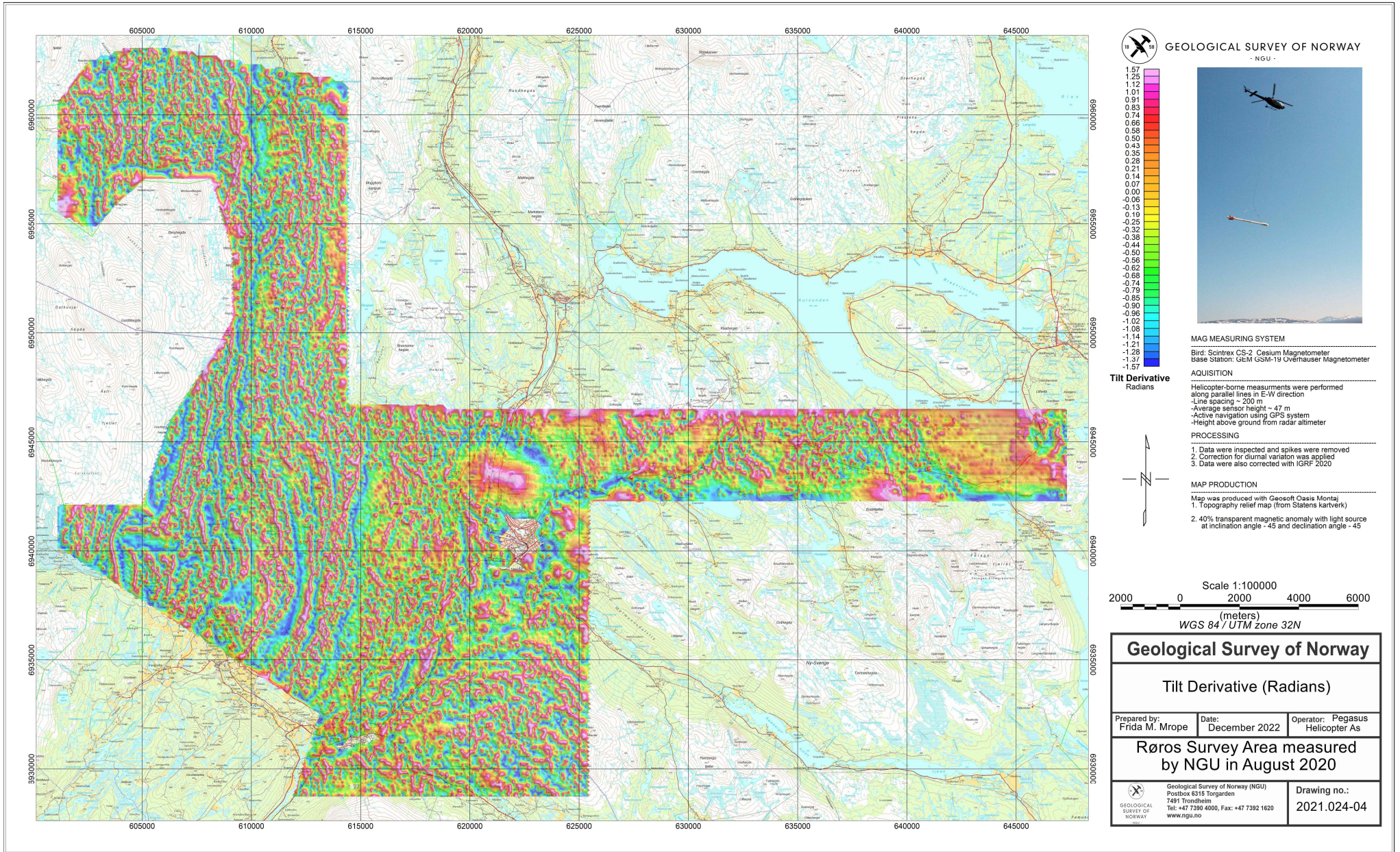
Figure 8: Magnetic Tilt Derivative.
