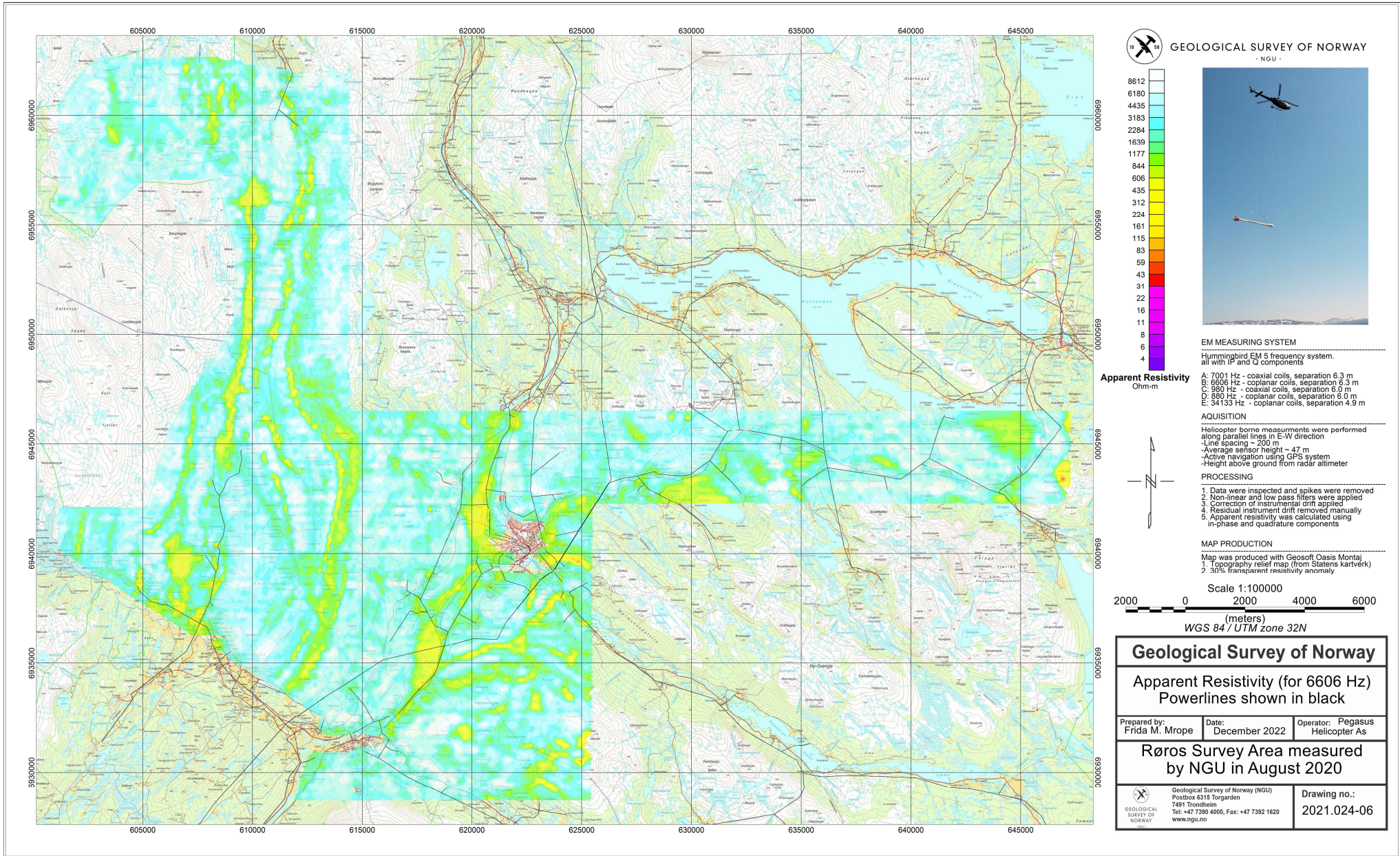
Figure 10: Apparent resistivity. Frequency 6606 Hz, Coplanar coils.
