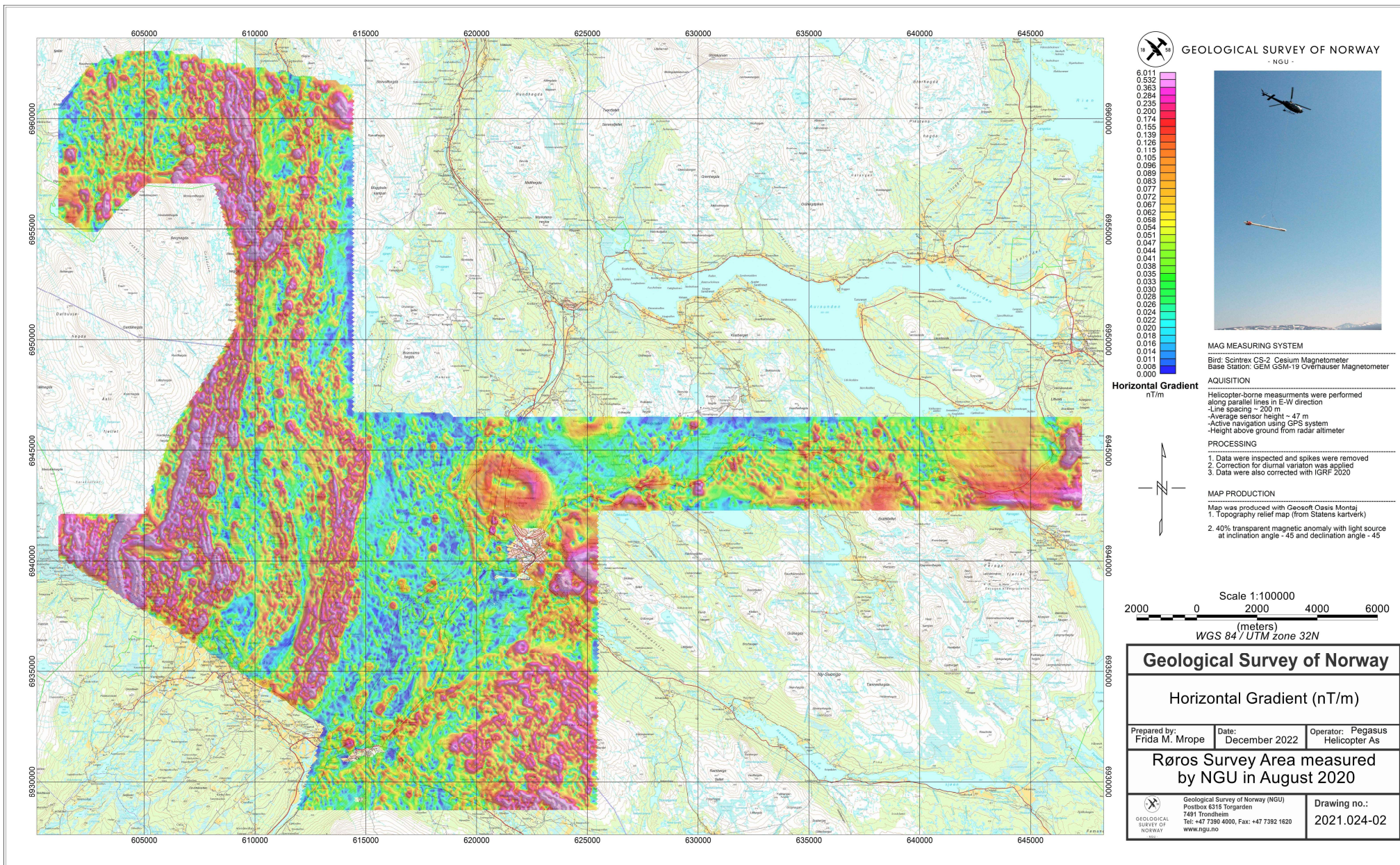
Figure 6: Magnetic Horizontal Gradient.
