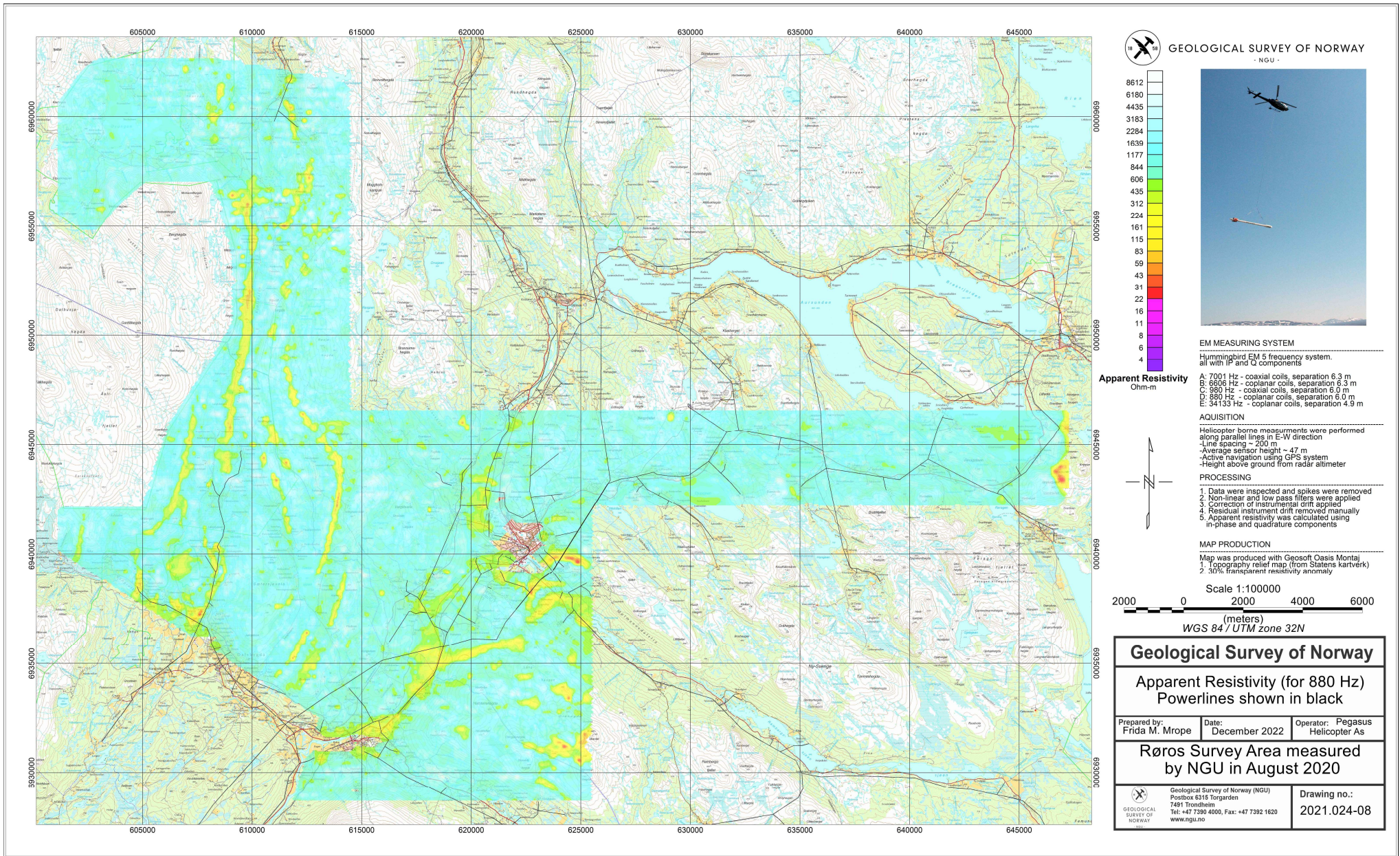
Figure 12: Apparent resistivity. Frequency 880 Hz, Coplanar coils.
