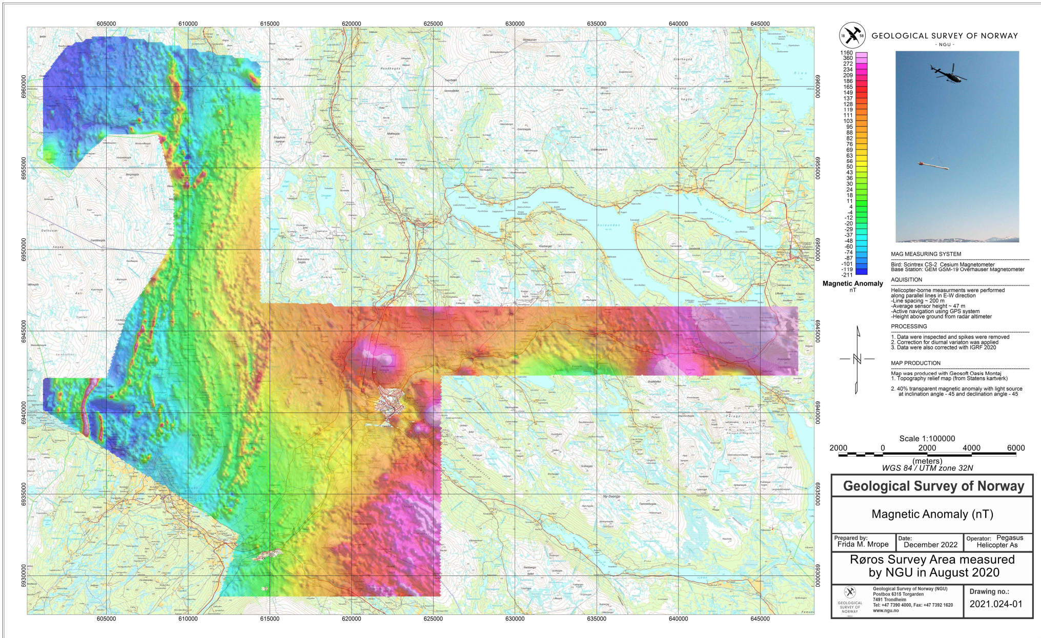
Figure 5: Total Magnetic Field.
