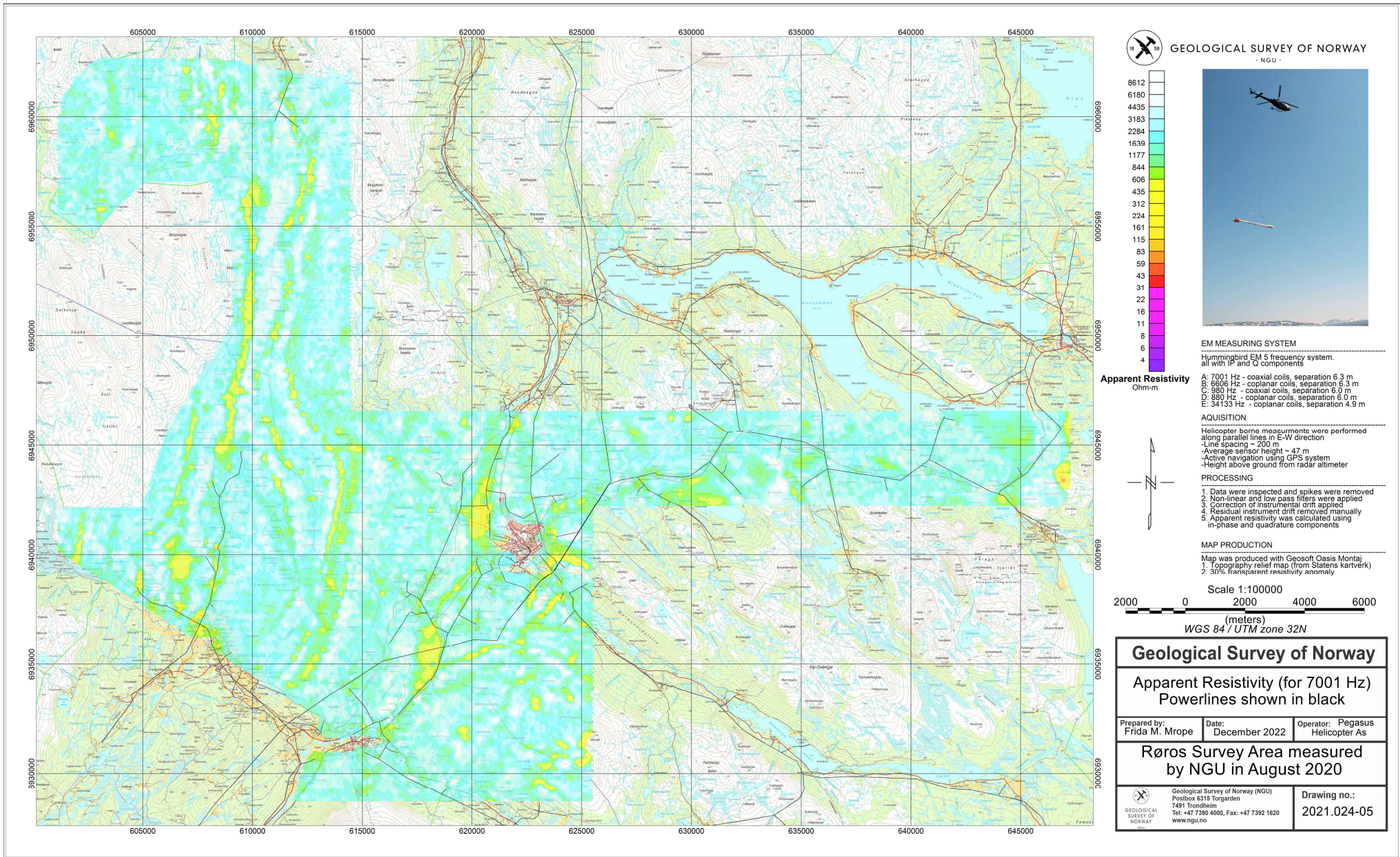
Figure 9: Apparent resistivity. Frequency 7001 Hz, Coaxial coils.
