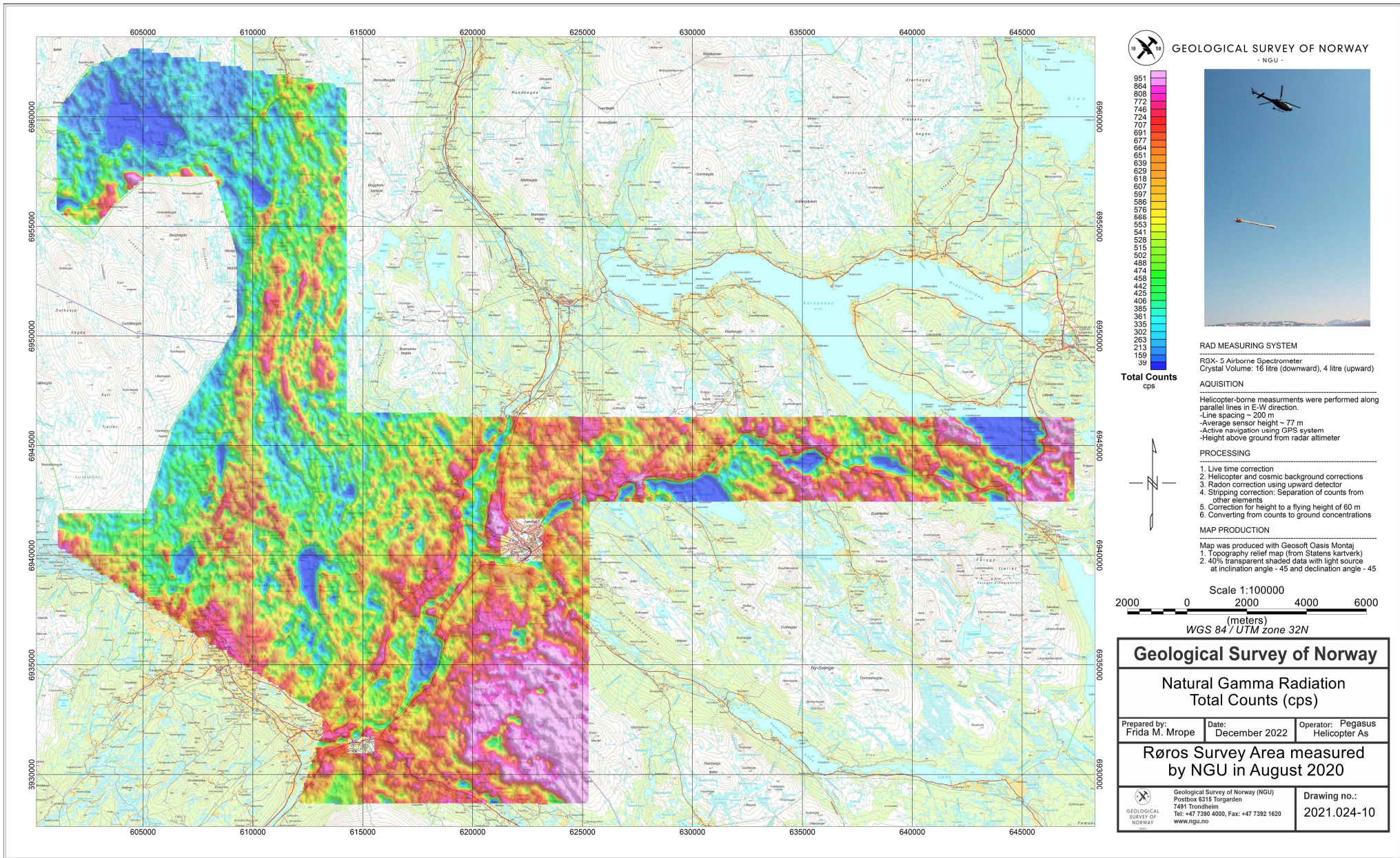
Figure 14: Radiometric Total counts.
