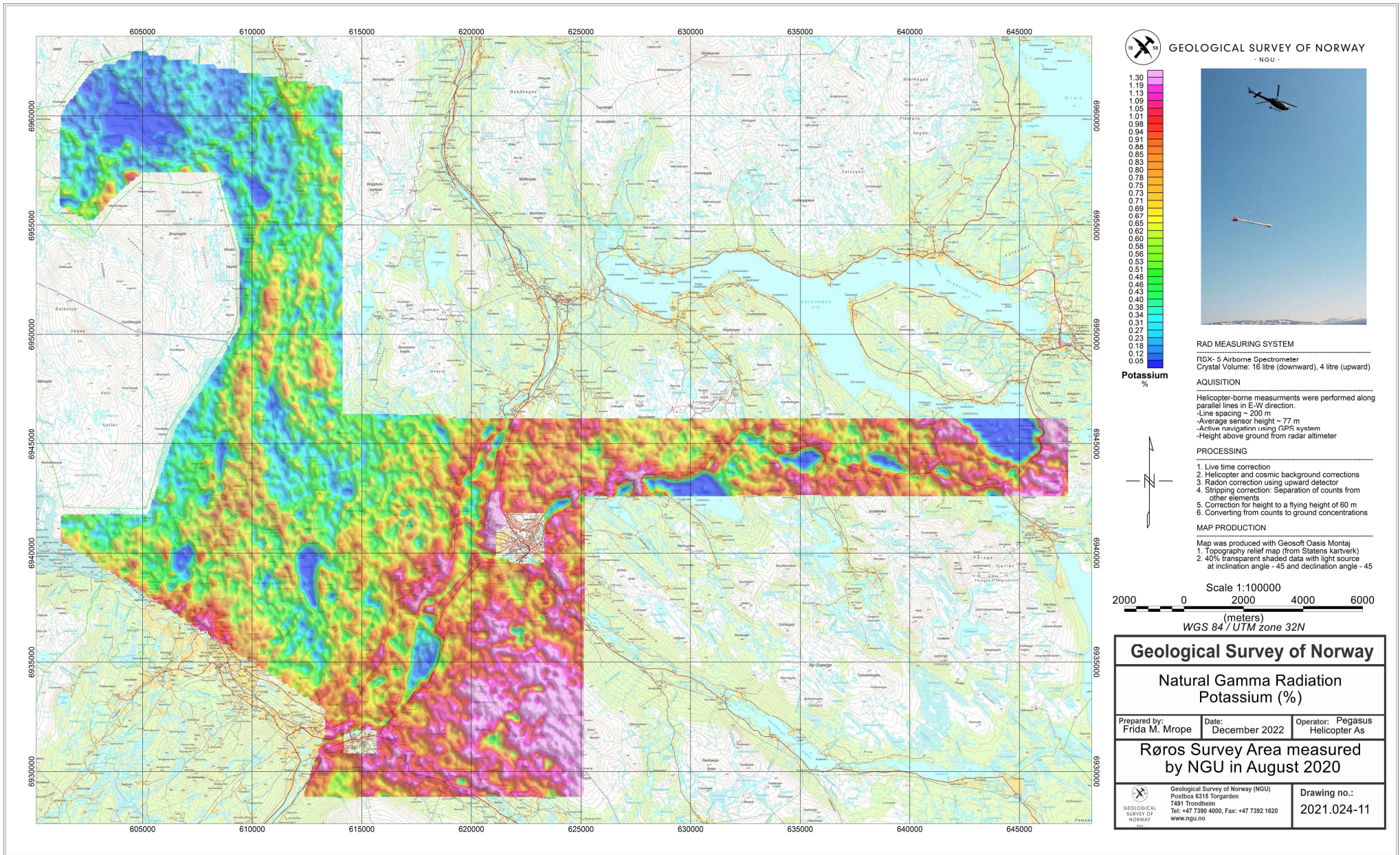
Figure 15: Potassium ground concentration.
