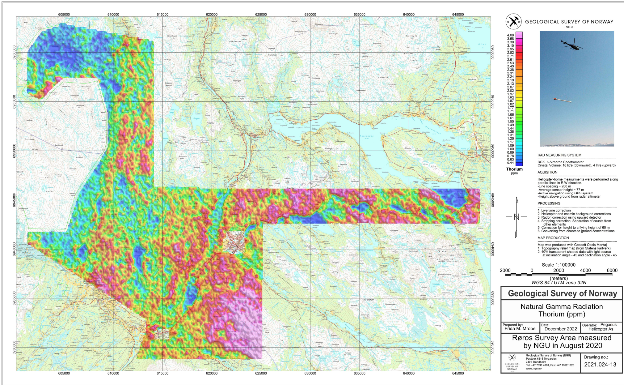
Figure 17: Thorium ground concentration.
