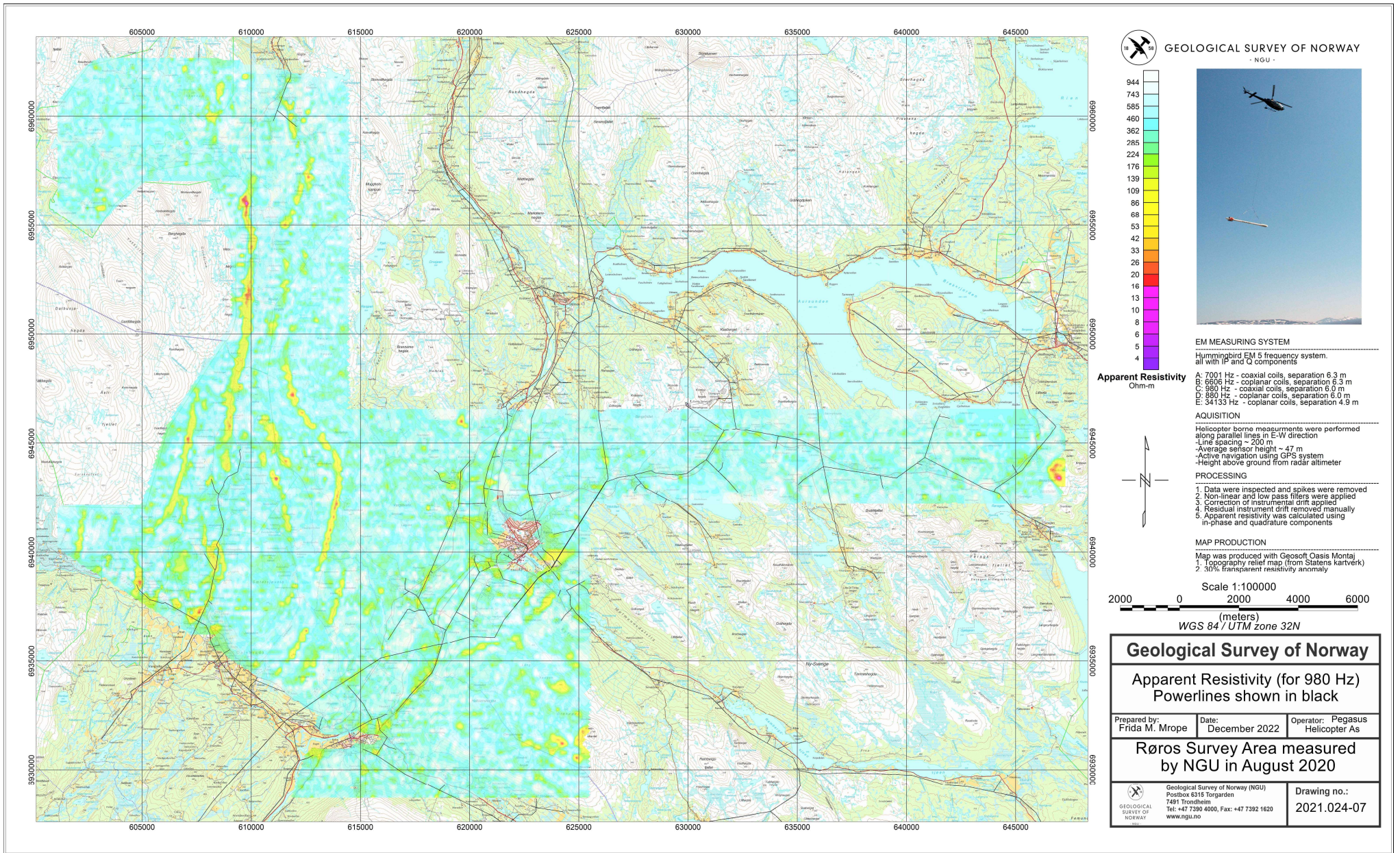
Figure 11: Apparent resistivity. Frequency 980 Hz, Coaxial coils.
