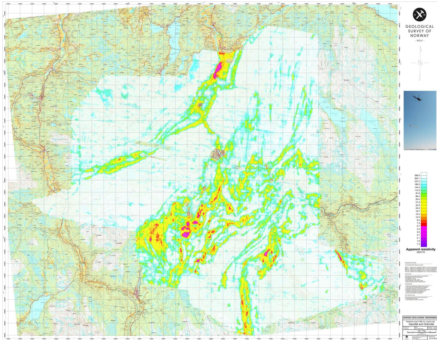
Figure 12: Apparent resistivity. Frequency 980 Hz, Coaxial coils
