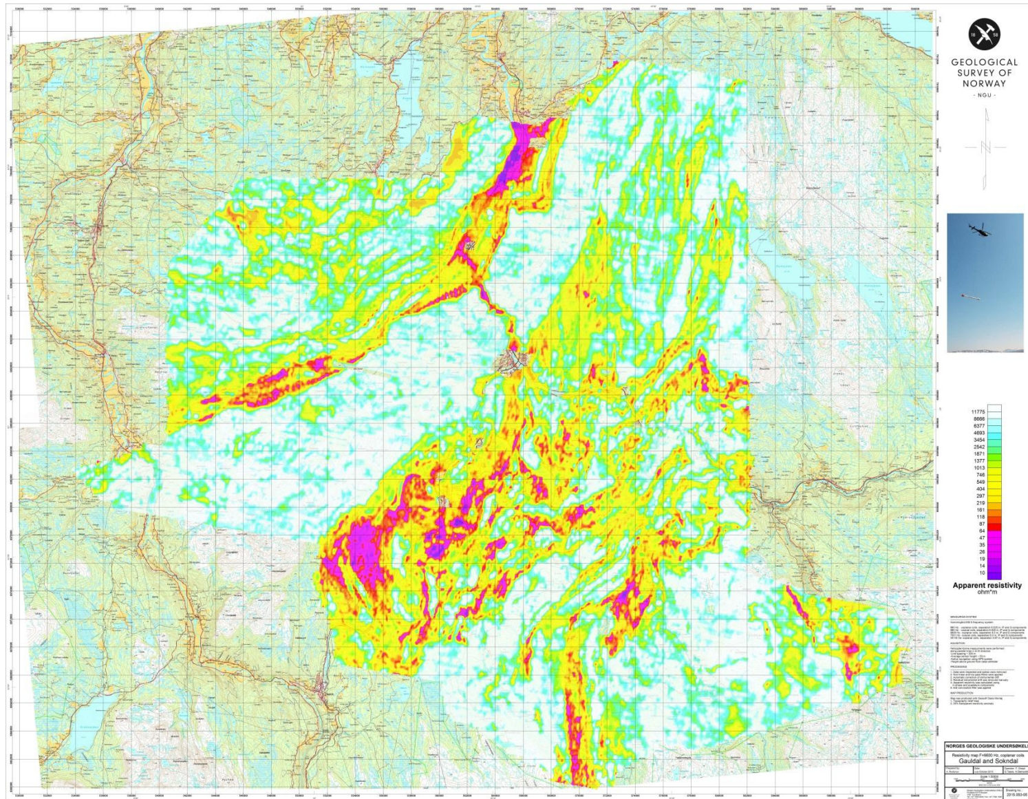
Figure 9: Apparent resistivity. Frequency 6600 Hz, Coplanar coils
