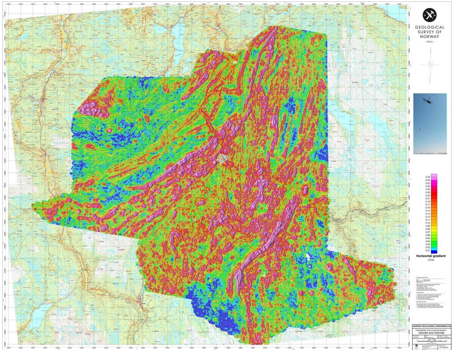
Figure 8: Magnetic Horizontal Gradient
