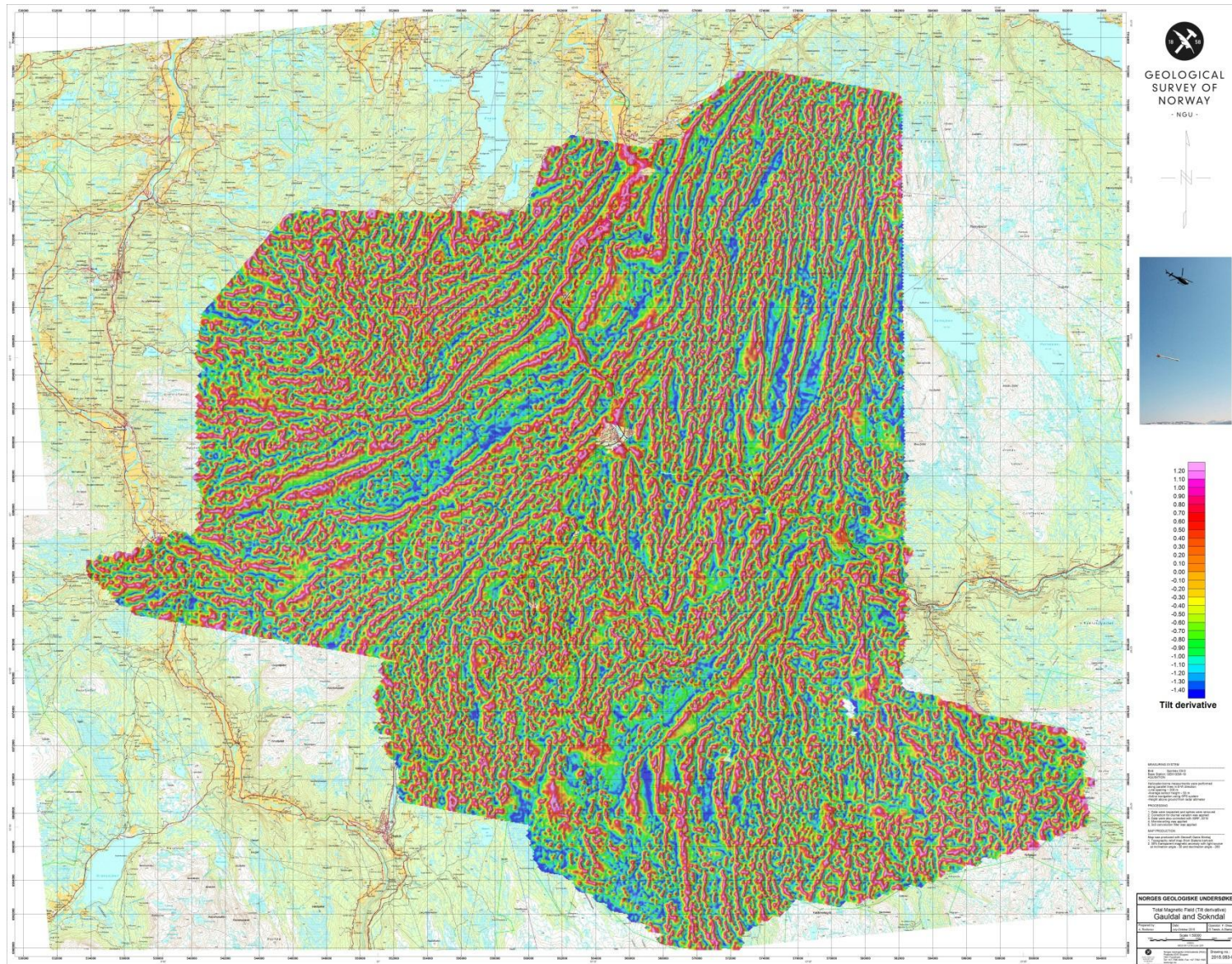
Figure 7: Magnetic Tilt Derivative
