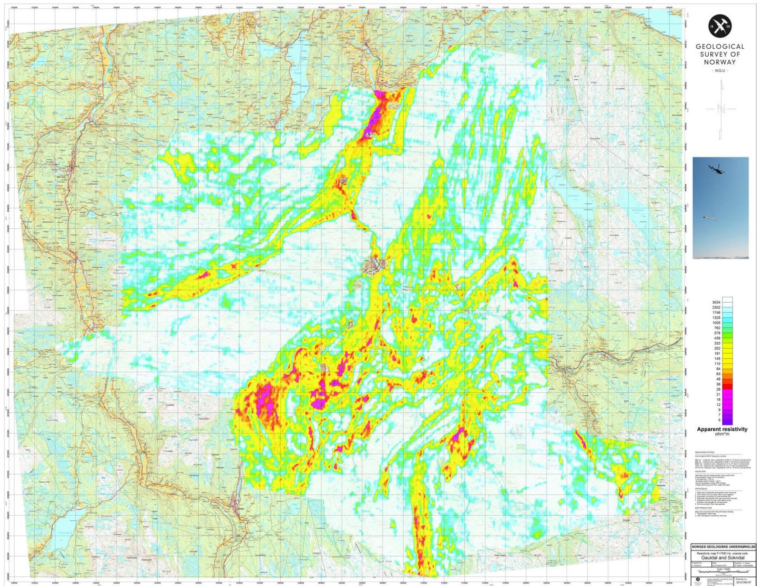
Figure 11: Apparent resistivity. Frequency 7000 Hz, Coaxial coils
