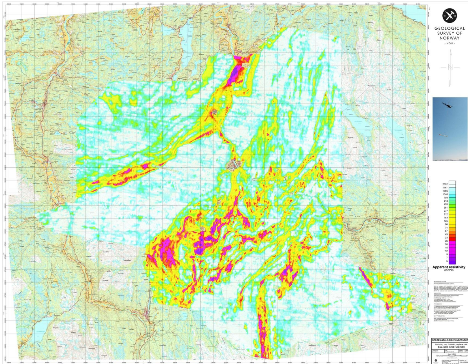
Figure 10: Apparent resistivity. Frequency 880 Hz, Coplanar coils
