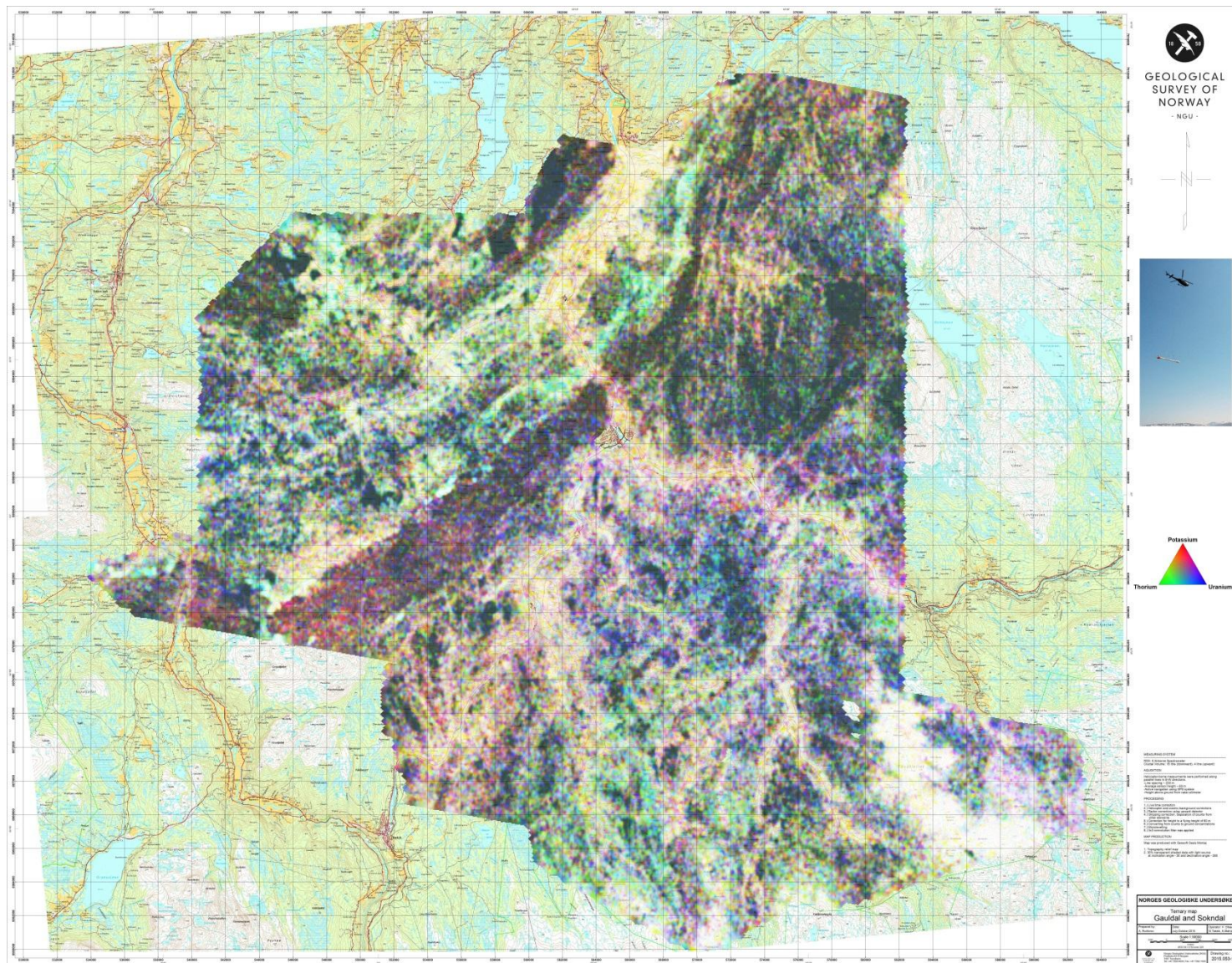
Figure 16: Radiometric Ternary map
