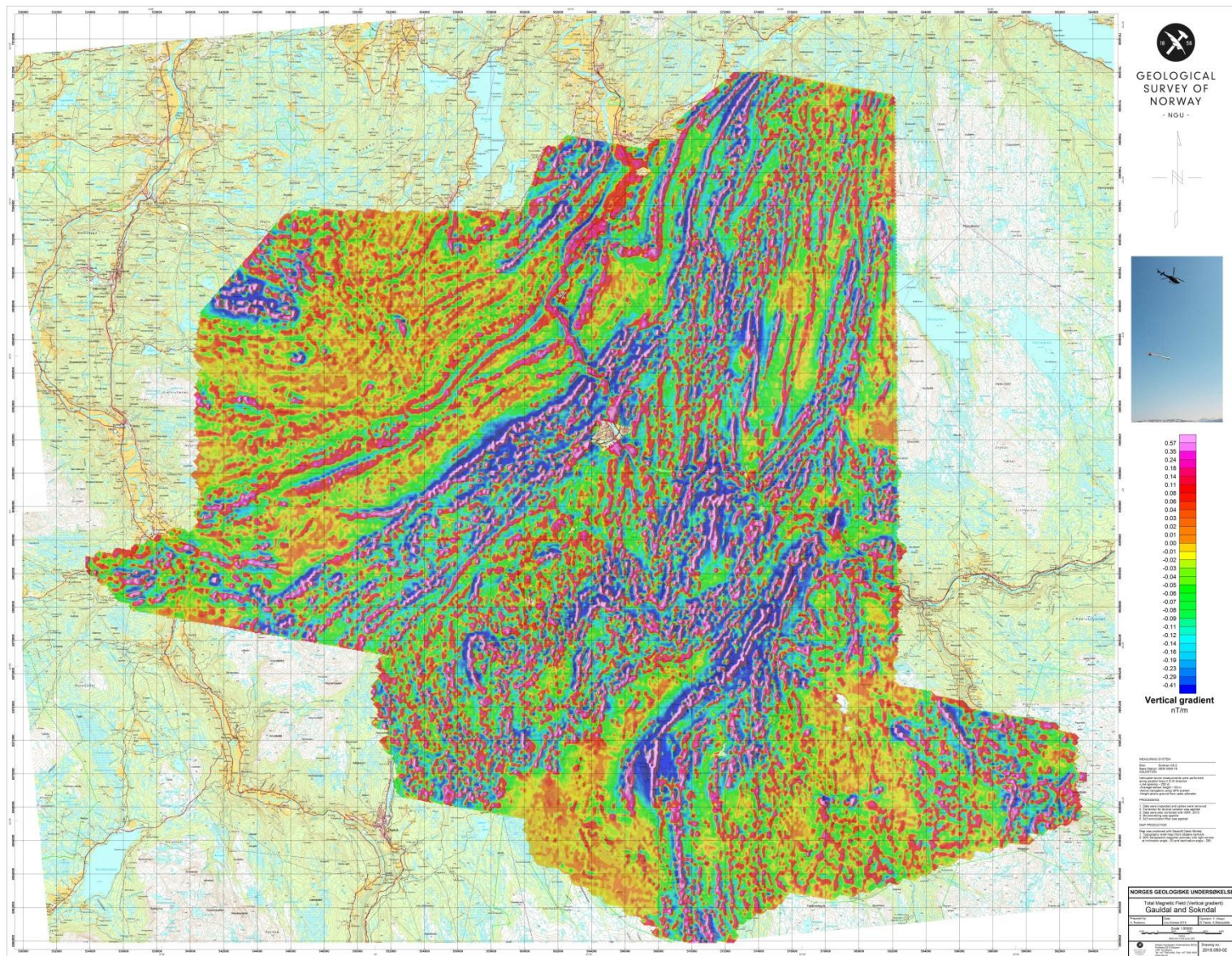
Figure 6: Magnetic Vertical Derivative
