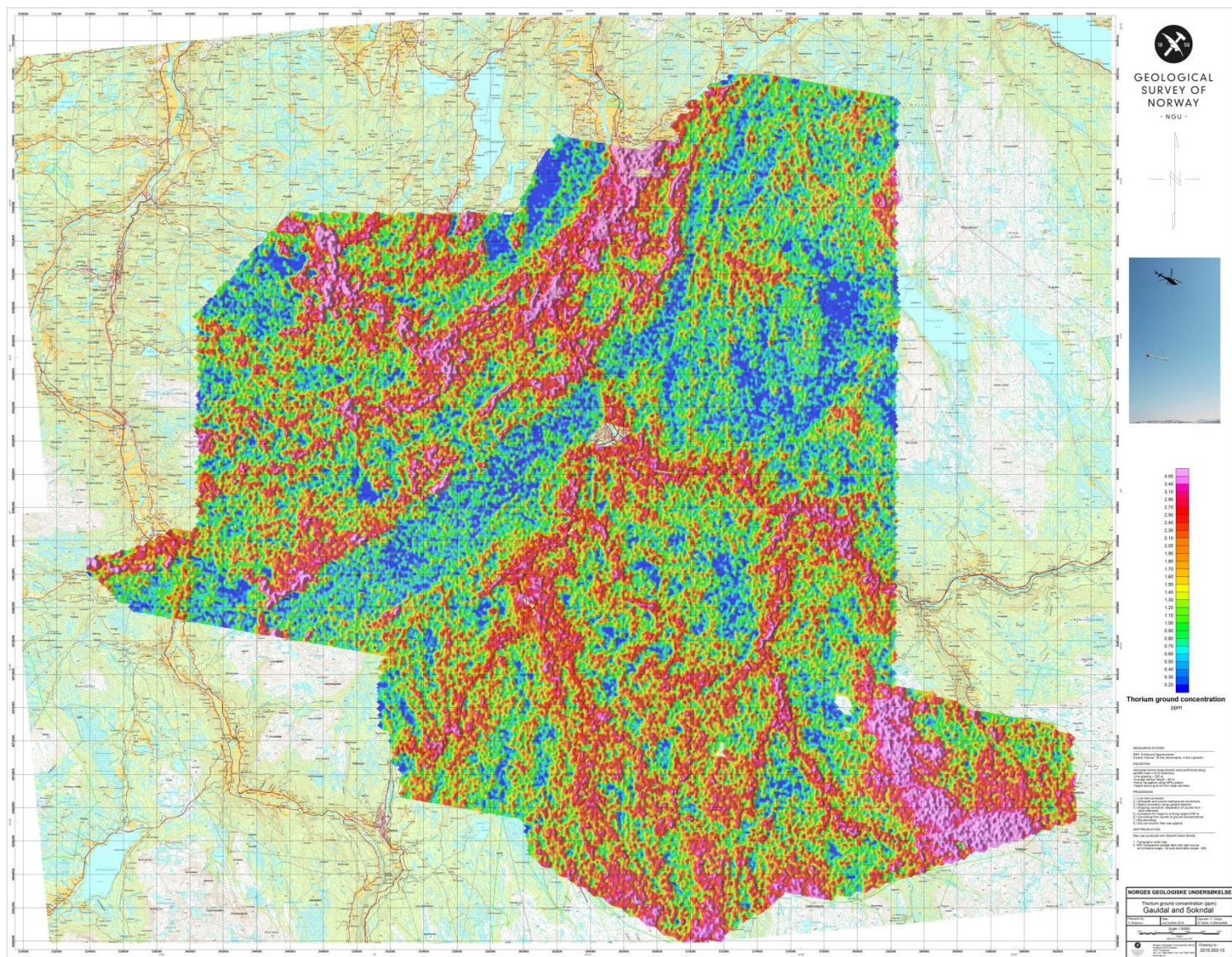
Figure 14: Thorium ground concentration
