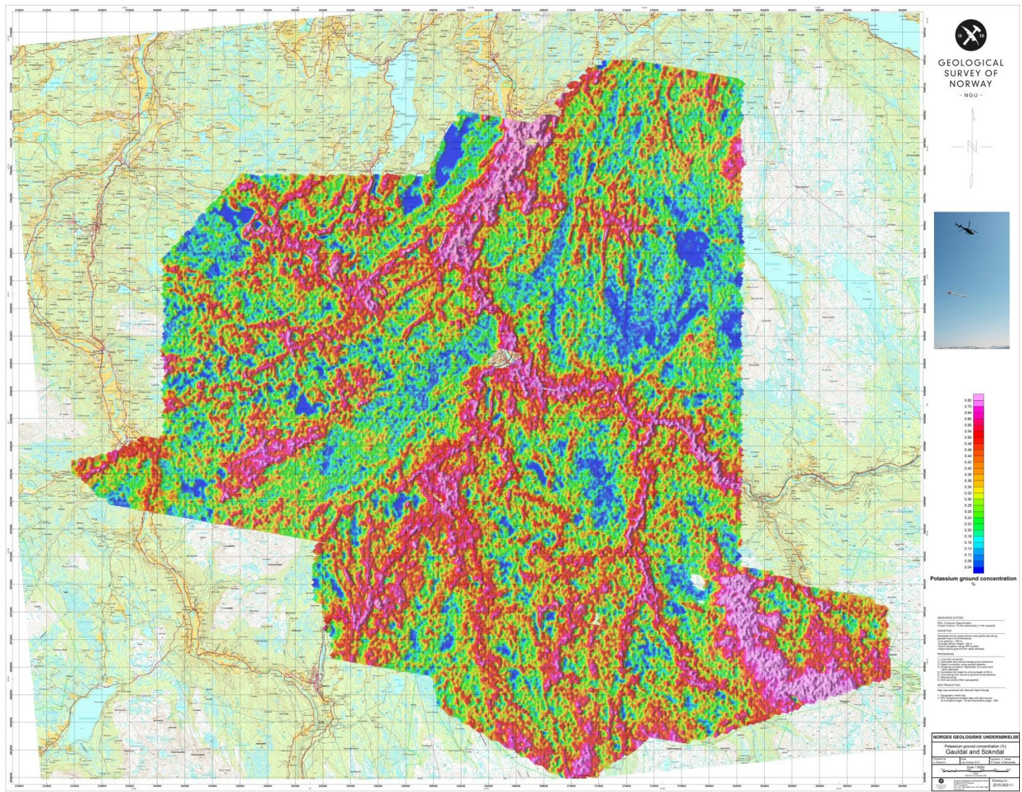
Figure 15: Potassium ground concentration
