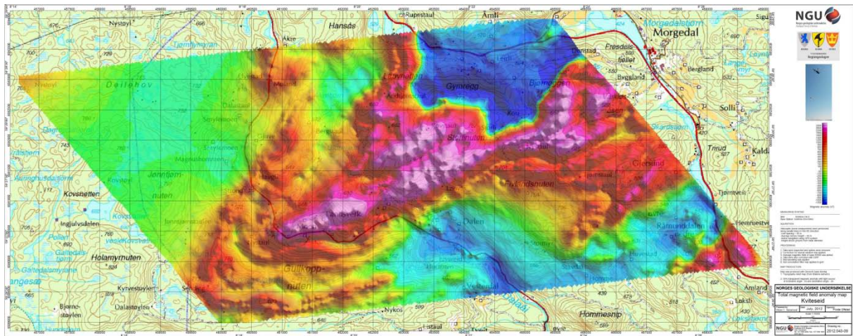
Figure 11. Total magnetic field anomaly map of Kviteseid with 50 m line spacing
