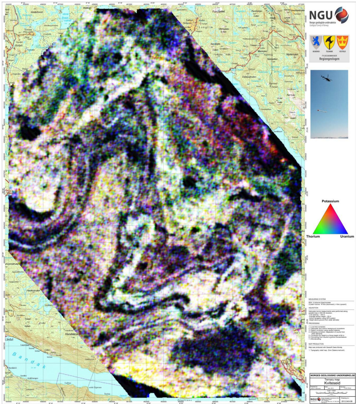
Figure 10. Ternary map of Kviteseid with 100 m line spacing
