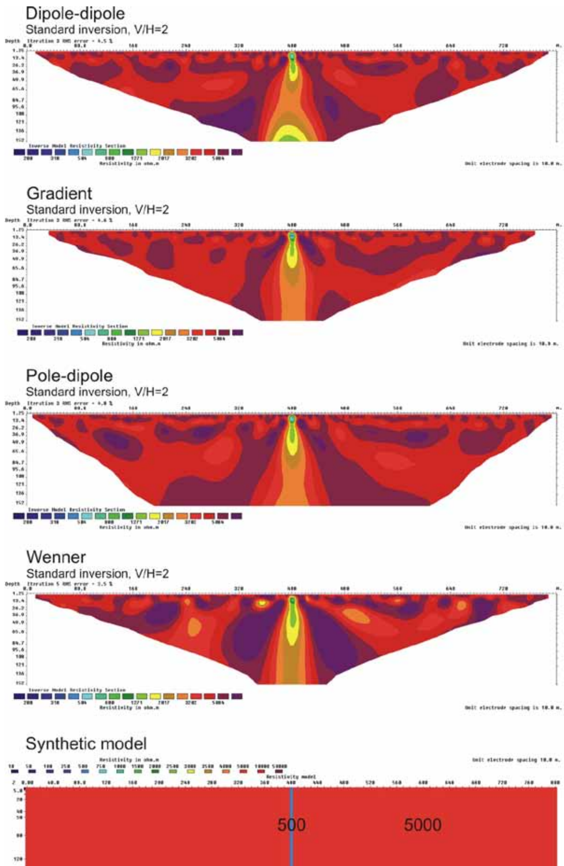
Figure 3.2.12: 5 m zone (500 ohmm), V/H=2
