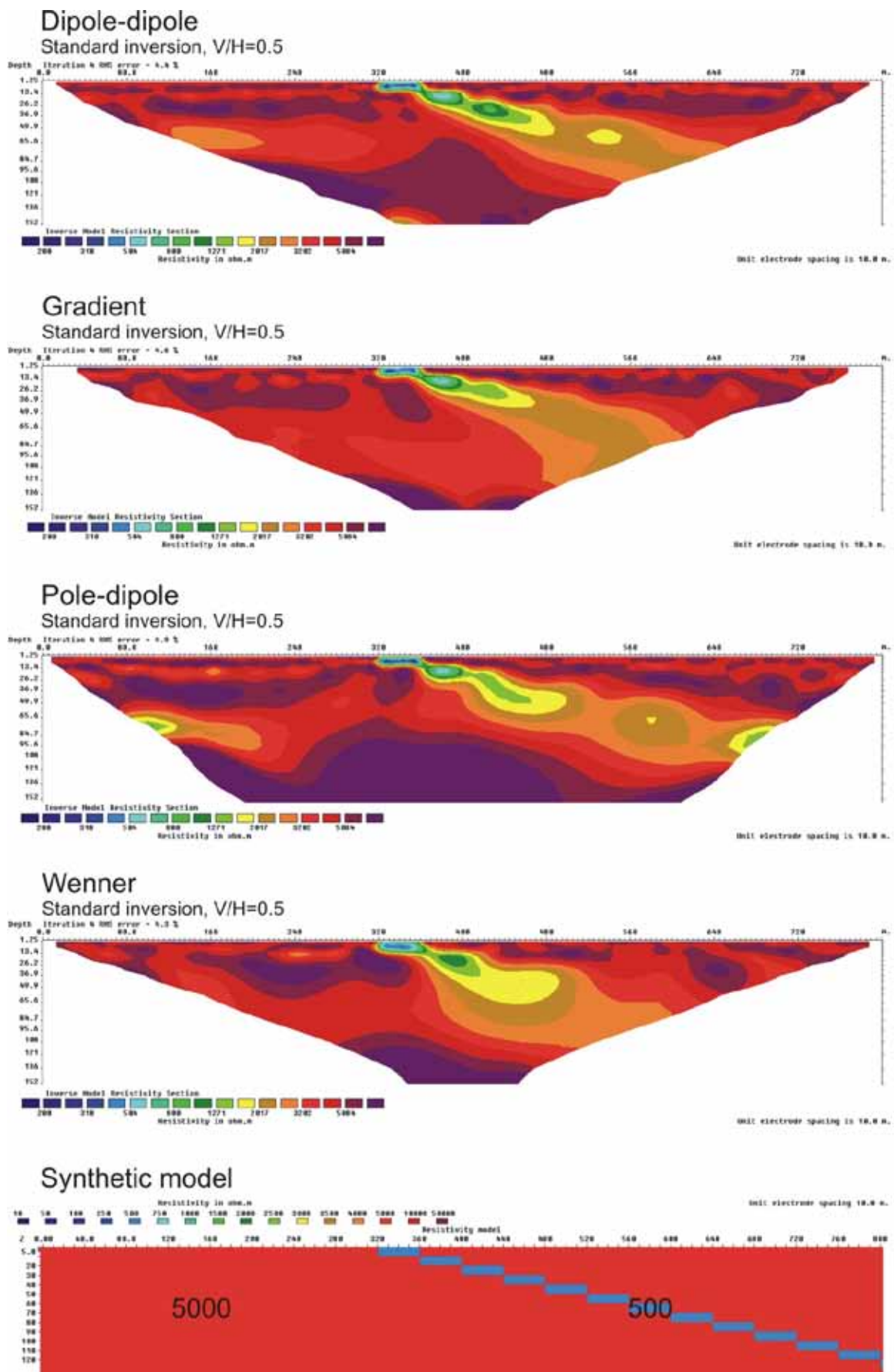
Figure 3.4.37: 10 m zone (500 ohmm) dipping with 15 degrees, V/H=0.5
