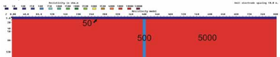
Figure 3.5.62: 10 m zone (500 ohmm) below a 5 m layer (50 ohmm), V/H=1
