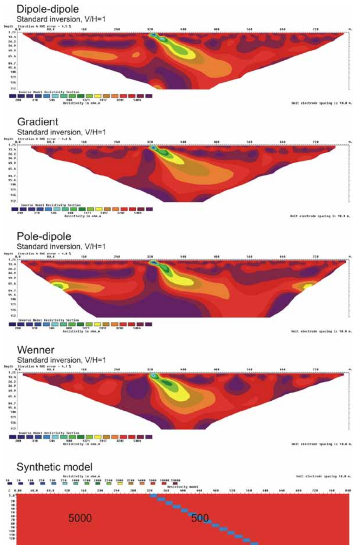
Figure 3.4.34: 10 m zone (500 ohmm) dipping with 30 degrees, V/H=1
