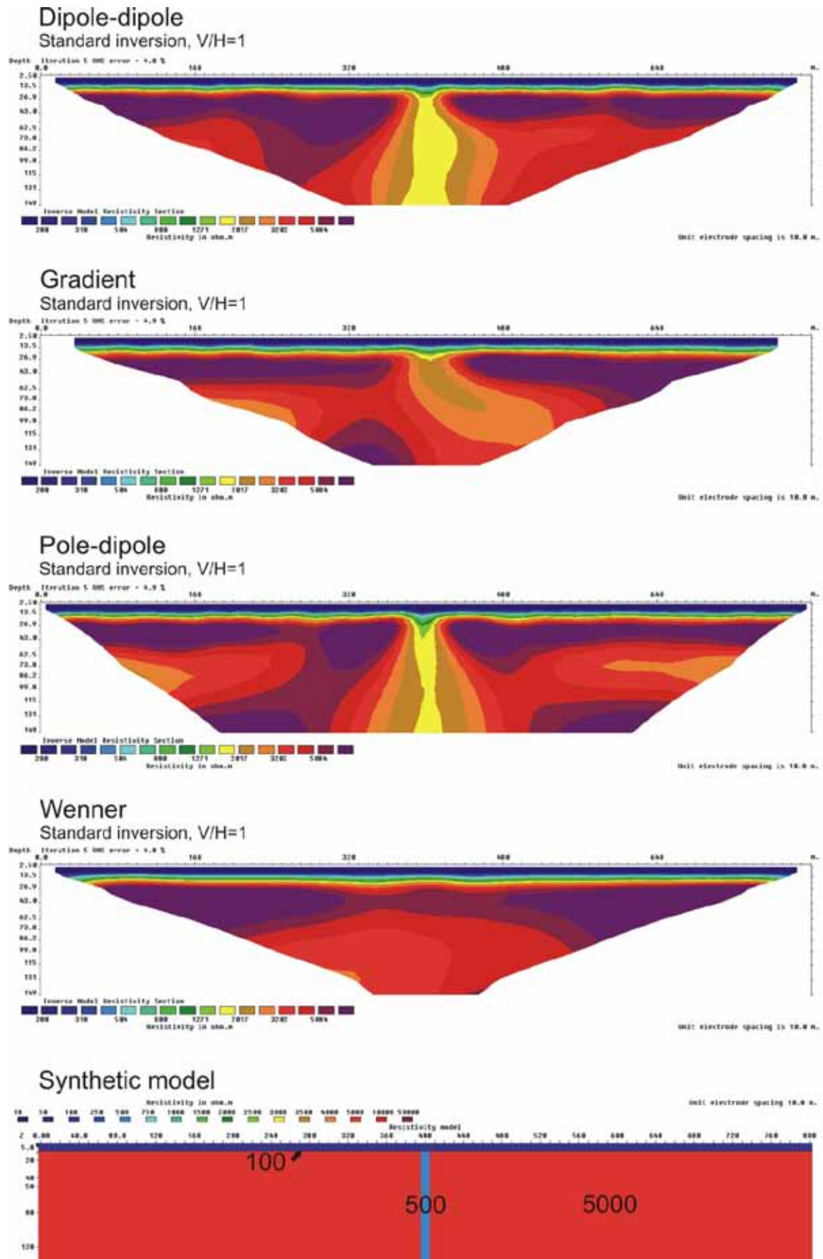
Figure 3.5.56: 10 m zone (500 ohmm) below a 10 m layer (100 ohmm), V/H=1
