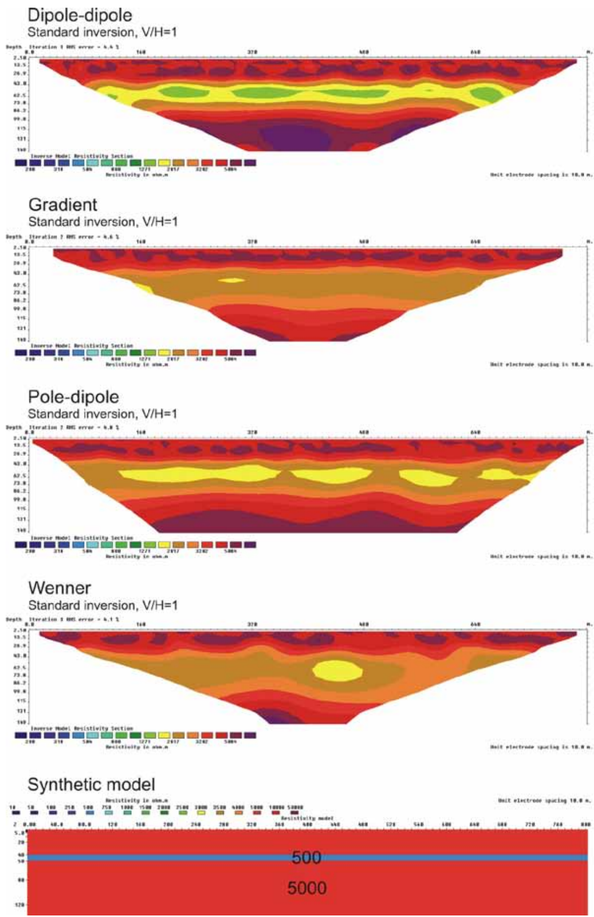
Figure 3.6.86: 10 m zone (500 ohmm) at a depth of 40m, V/H=1
