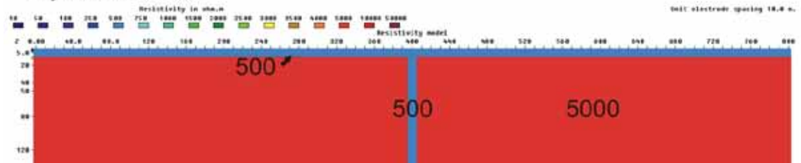
Figure 3.5.49: 10 m zone (500 ohmm) below a 10 m layer (500 ohmm), V/H=2
