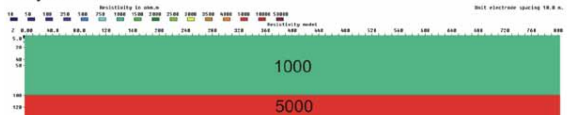
Figure 3.6.76: 2-layer model (1000 ohmm over 5000 ohmm), V/H=1
