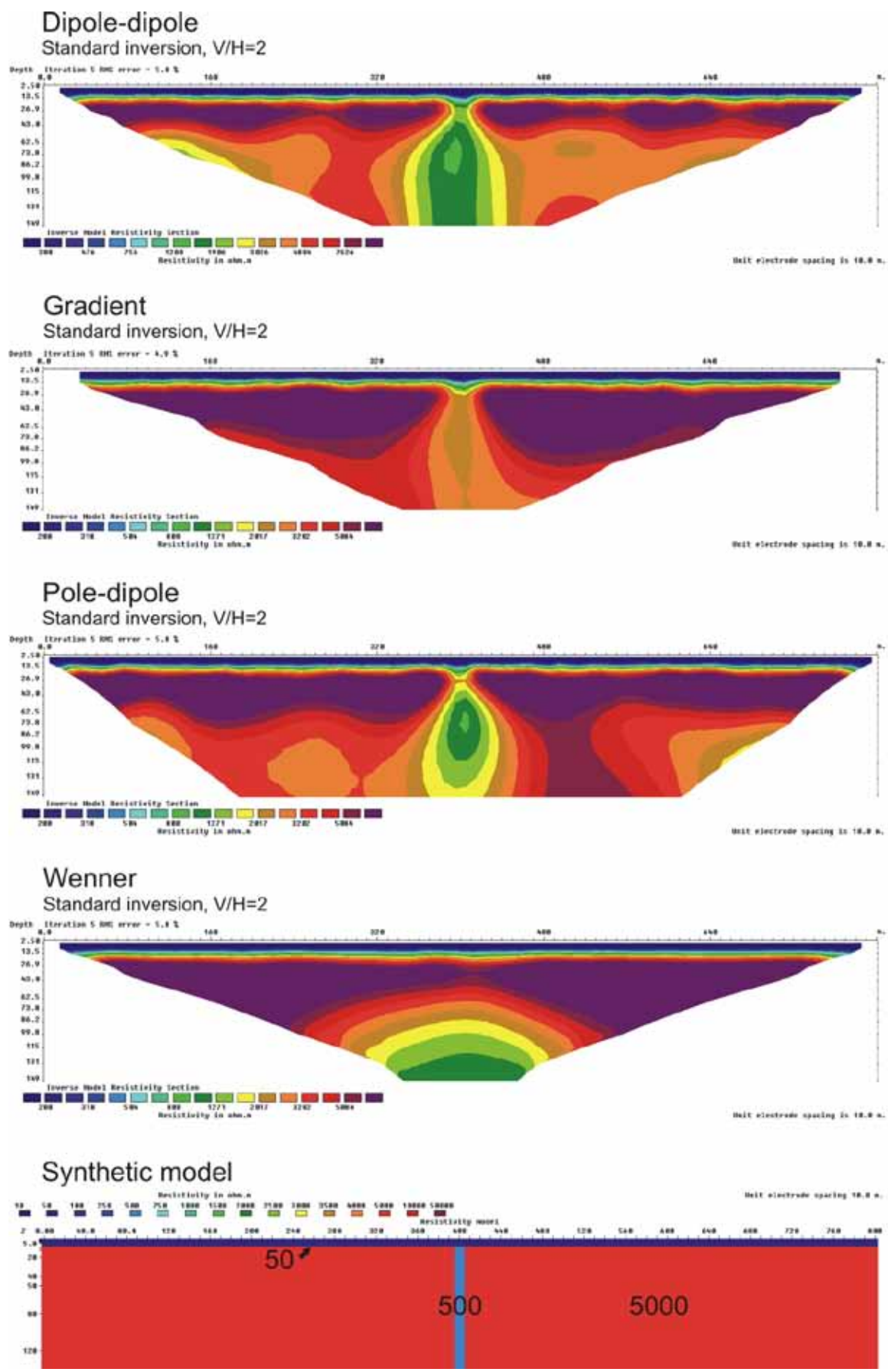
Figure 3.5.63: 10 m zone (500 ohmm) below a 5 m layer (50 ohmm), V/H=2
