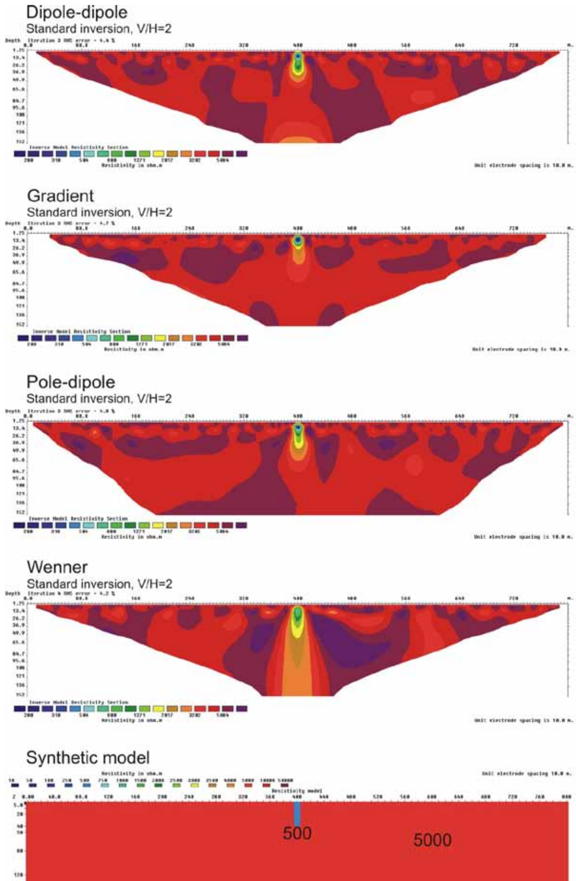
Figure 3.1.6: 10 m zone (500 ohmm) with a depth of 40 m, V/H=2
