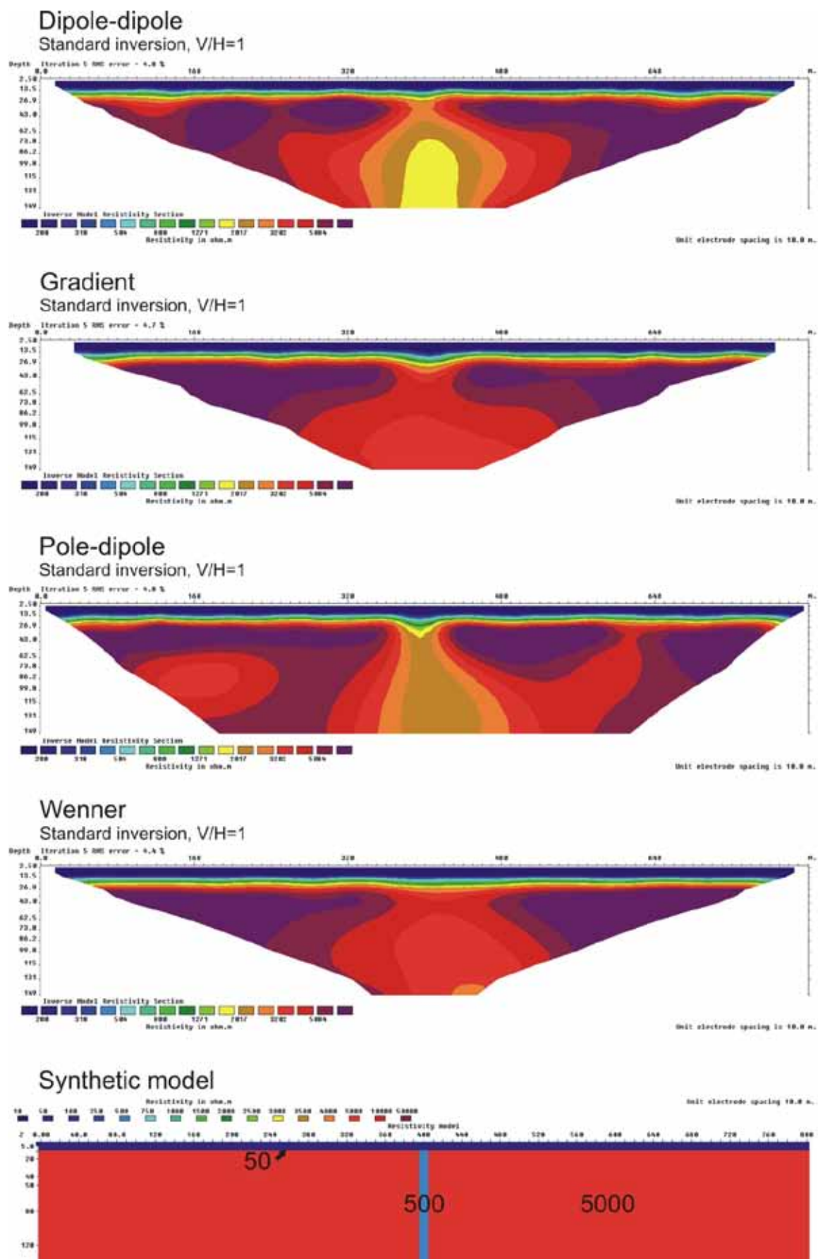
Figure 3.5.64: 10 m zone (500 ohmm) below a 10 m layer (50 ohmm), V/H=1
