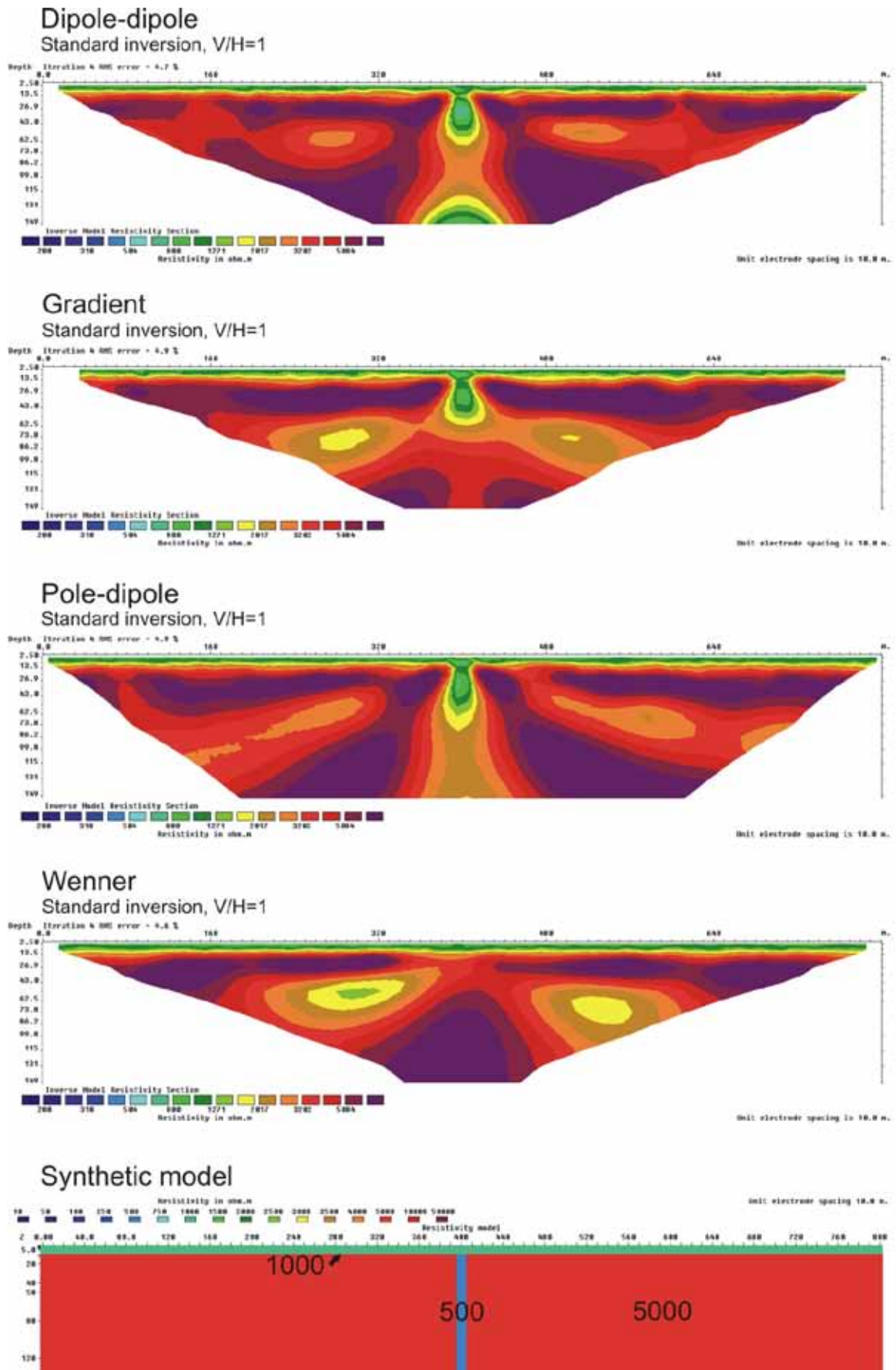
Figure 3.5.40: 10 m zone (500 ohm) below a 10 m layer (1000 ohm), V/H=1
