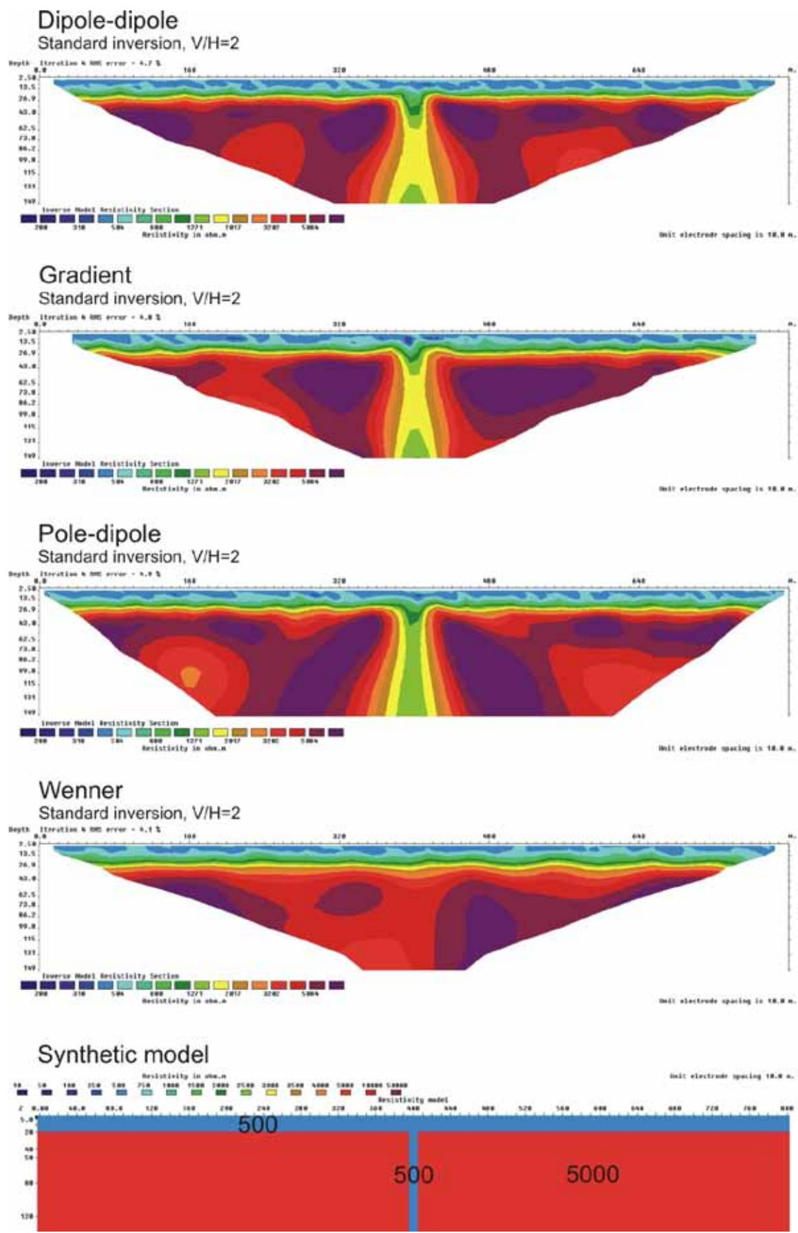
Figure 3.5.51: 10 m zone (500 ohmm) below a 20 m layer (500 ohmm), V/H=2
