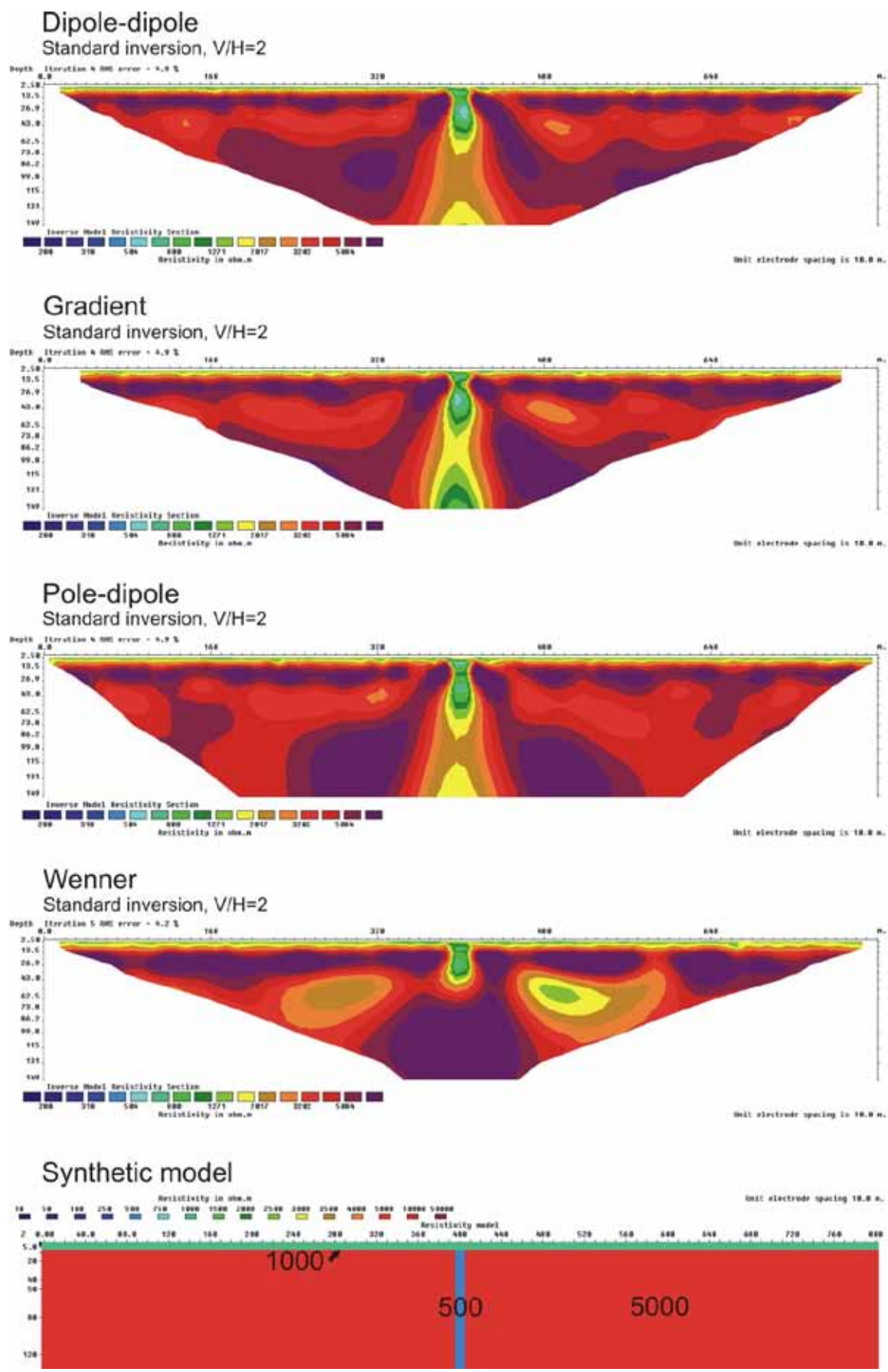
Figure 3.5.39: 10 m zone (500 ohmm) below a 5 m layer (1000 ohmm), V/H=2
