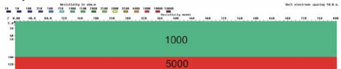
Figure 3.6.77: 2-layer model (1000 ohmm over 5000 ohmm), V/H=0.5
