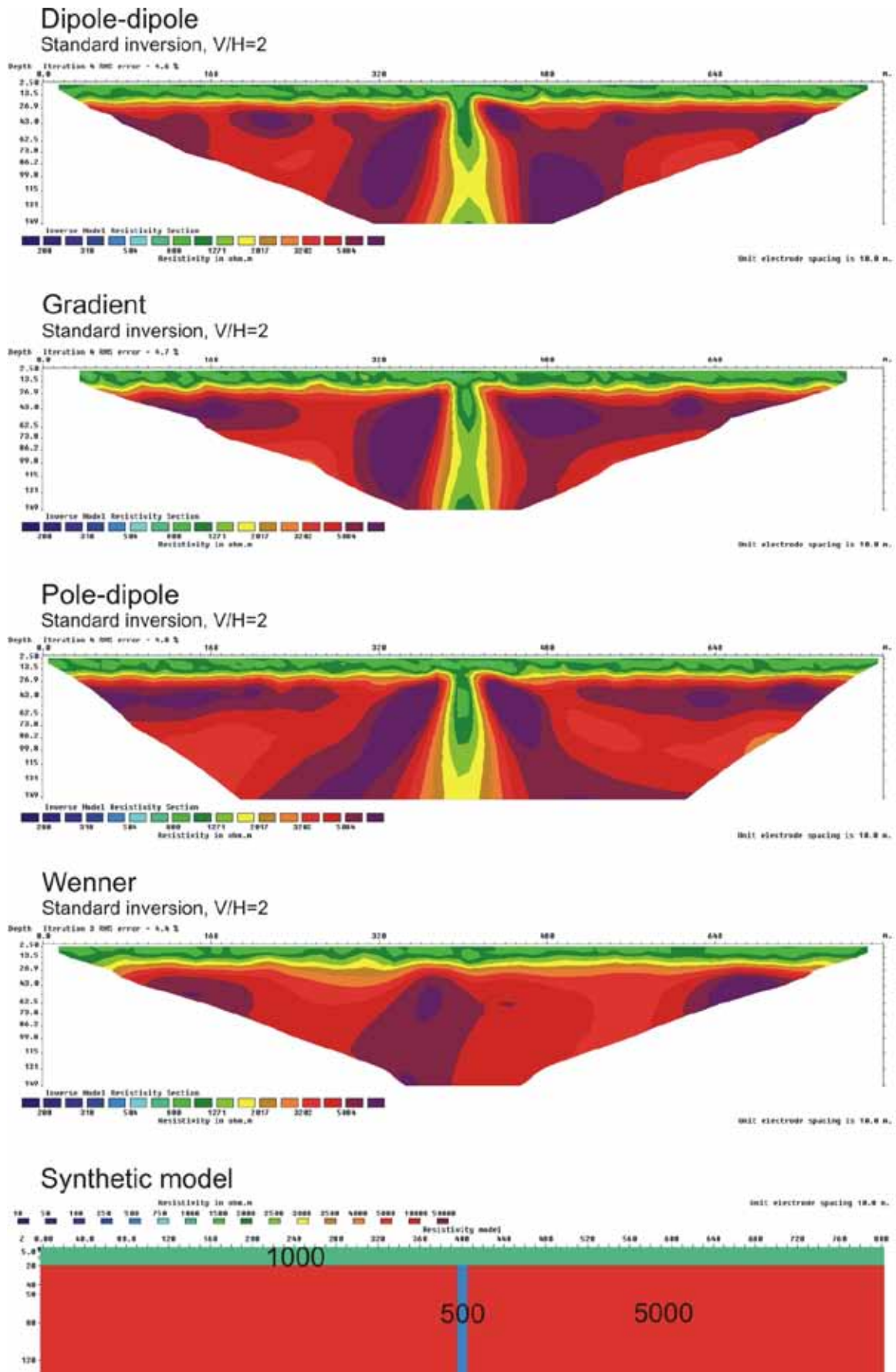
Figure 3.5.43: 10 m zone (500 ohmm) below a 20 m layer (1000 ohmm), V/H=2
