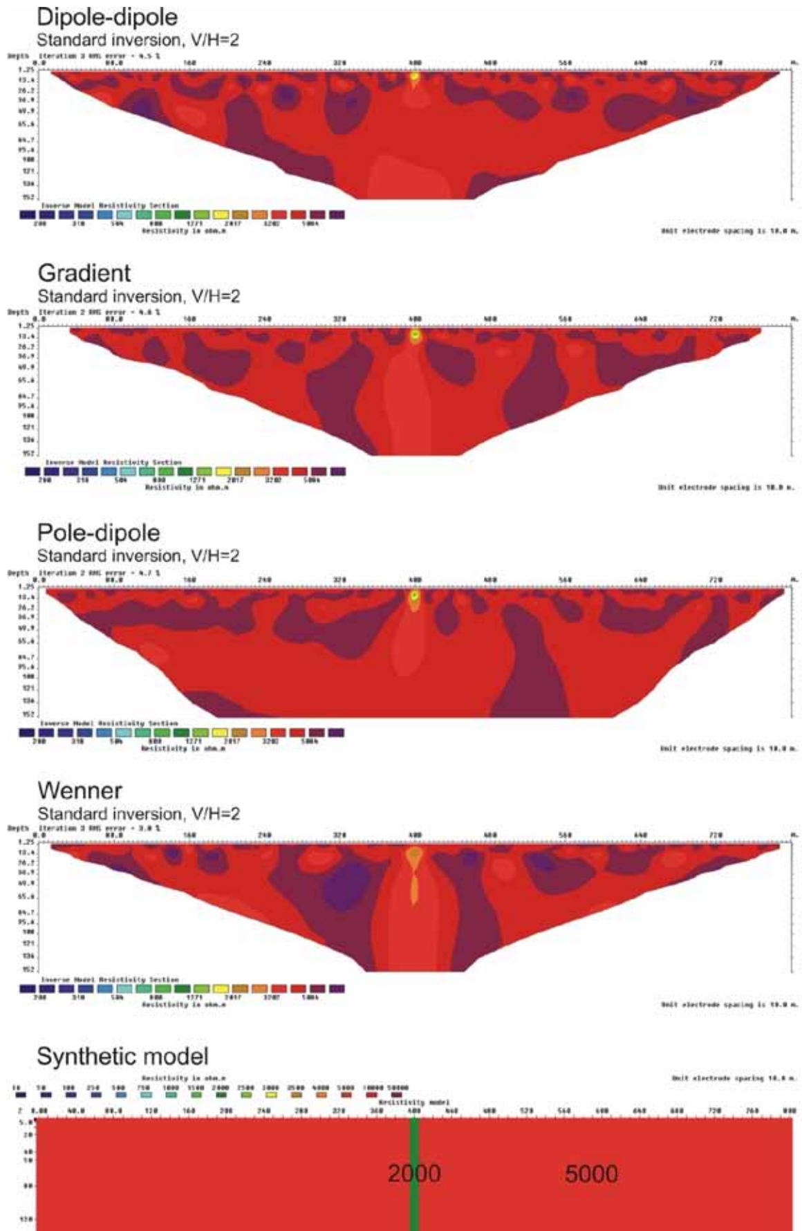
Figure 3.3.26: 10 m zone (2000 ohm) in bedrock (5000 ohm), V/H=2
