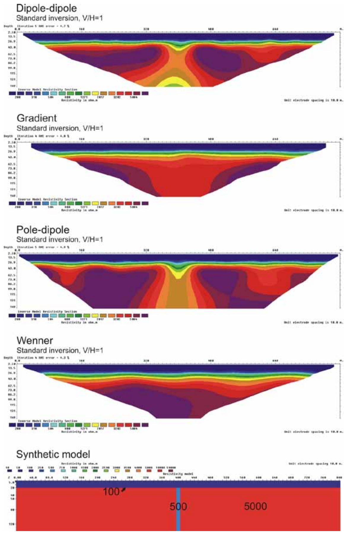
Figure 3.5.58: 10 m zone (500 ohmm) below a 20 m layer (100 ohmm), V/H=1
