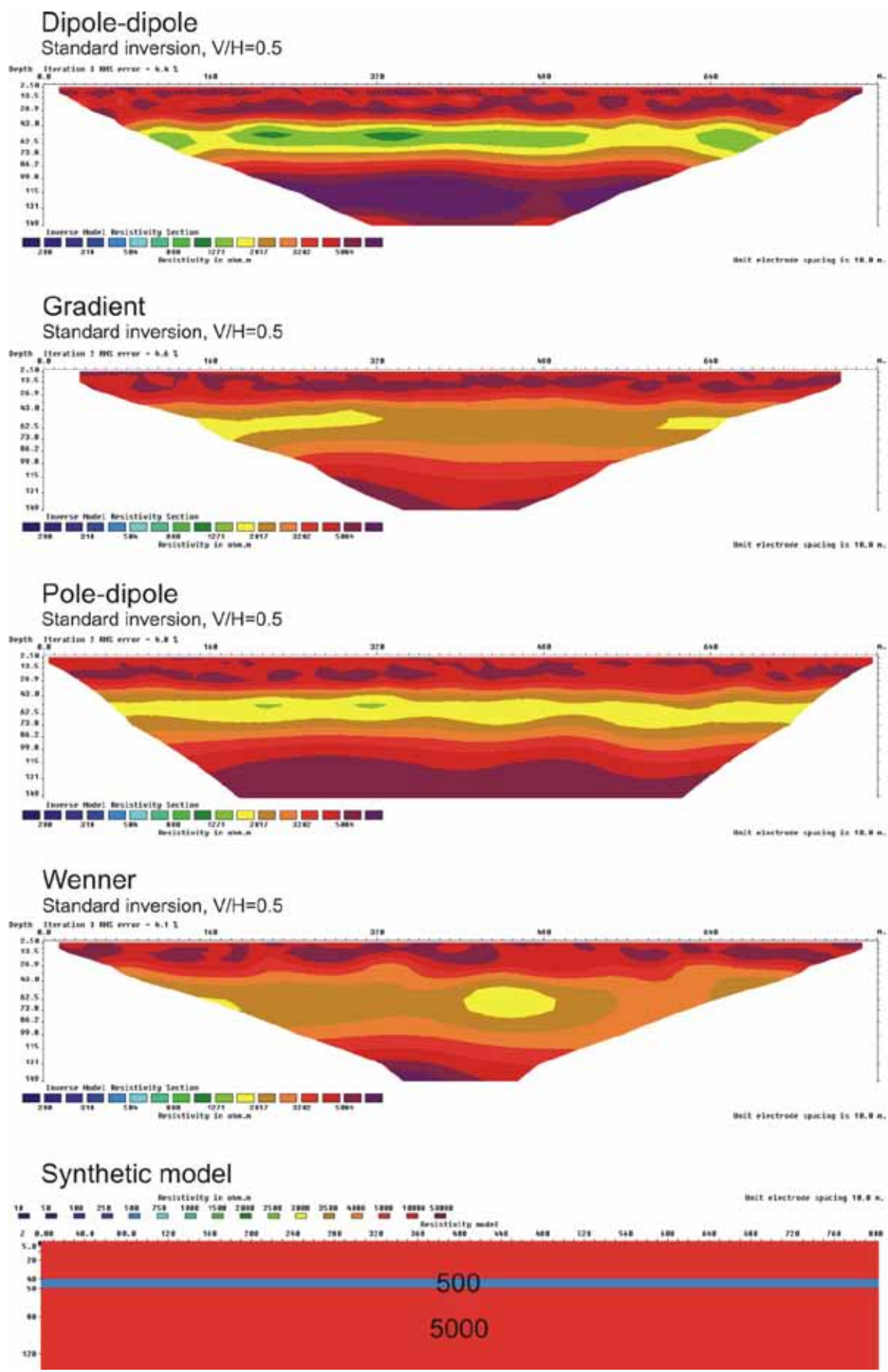
Figure 3.6.87: 10 m zone (500 ohmm) at a depth of 40m, V/H=0.5
