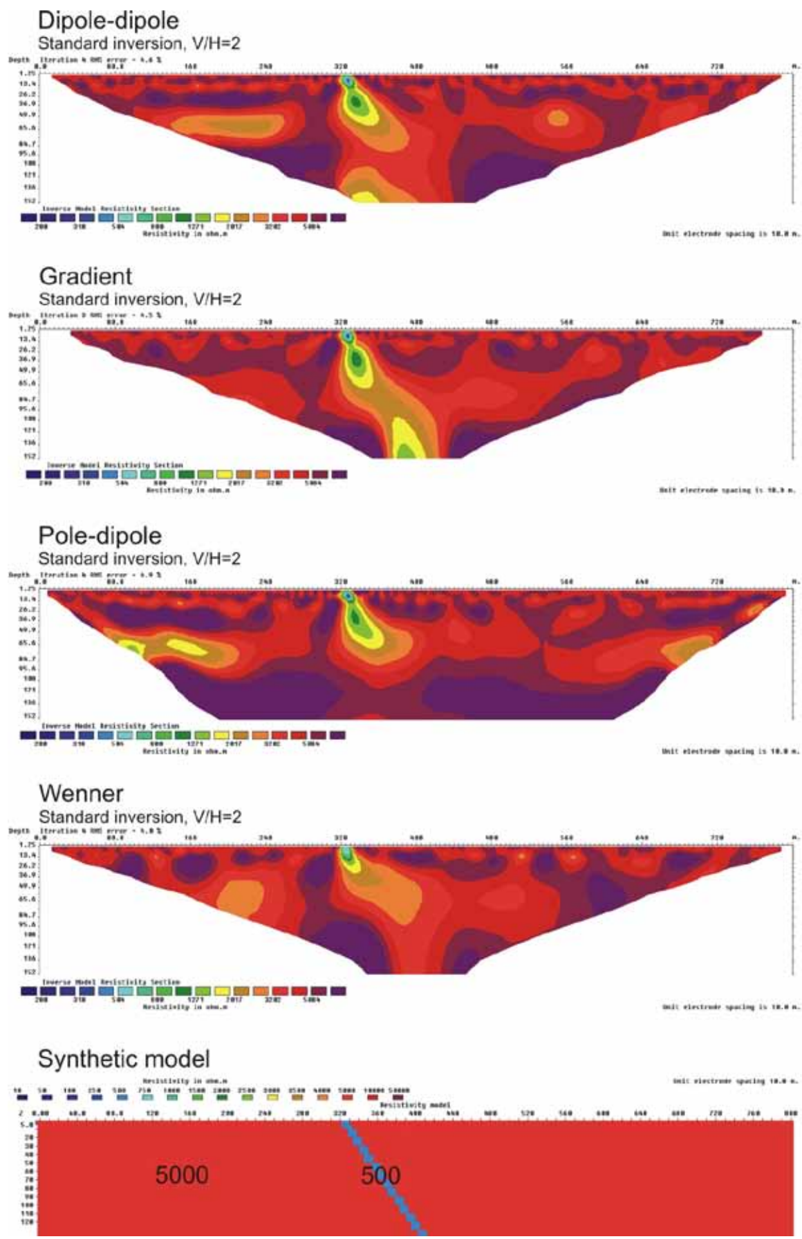
Figure 3.4.32: 10 m zone (500 ohm) dipping with 60 degrees, V/H=2
