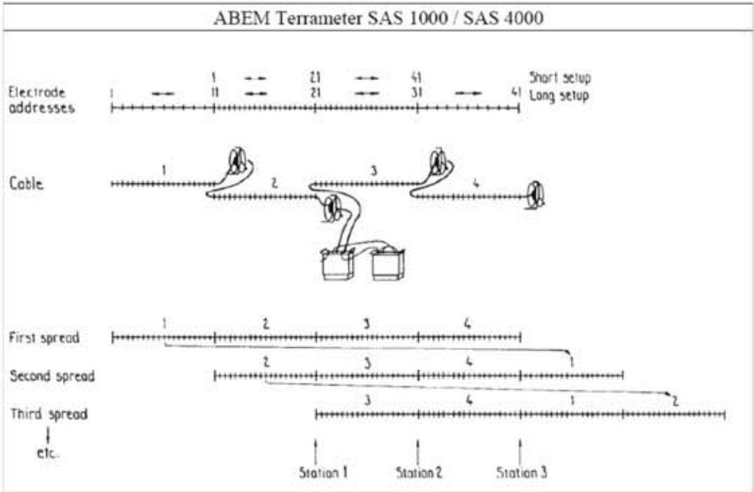
Figure 2.2: Measuring procedure in the field using 4 cables in a spread (From Dahlin 1993).
