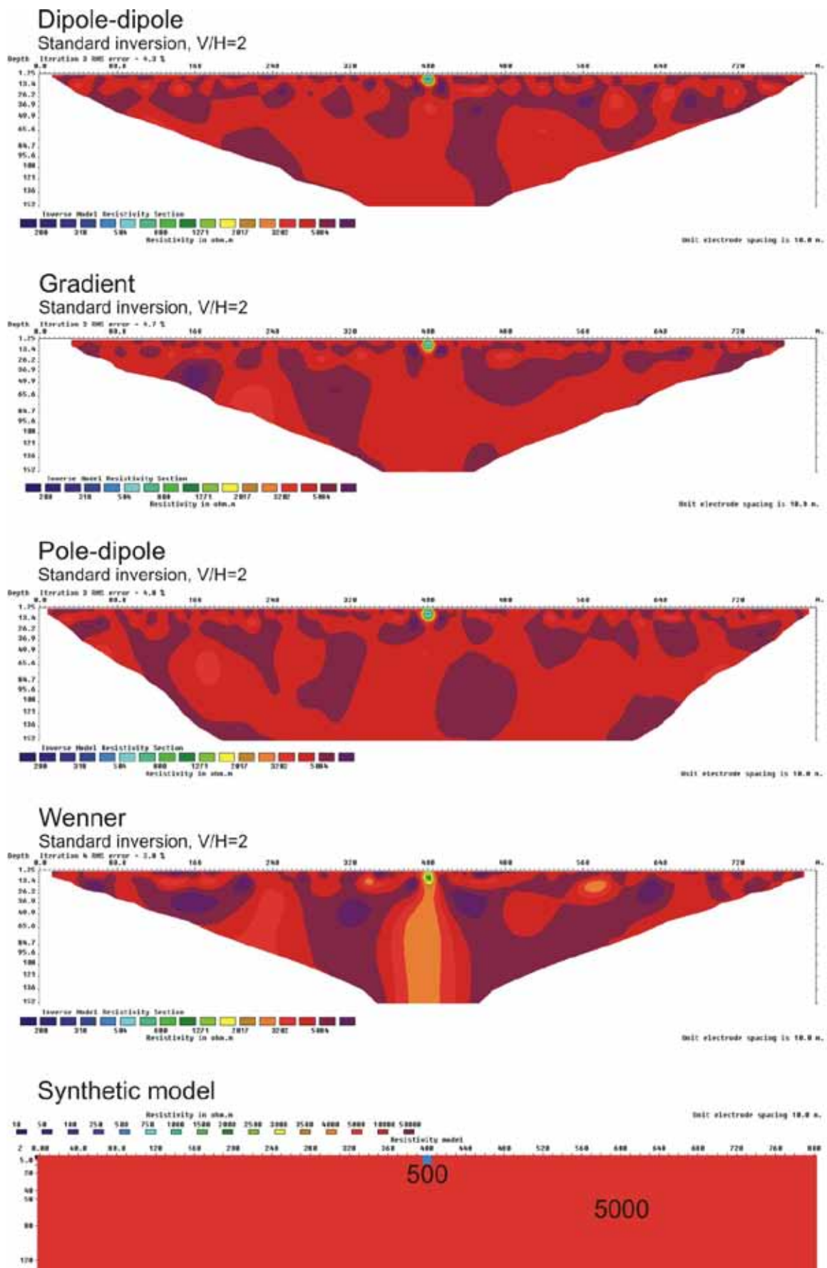
Figure 3.1.2: 10 m zone (500 ohmm) with a depth of 10 m, V/H=2
