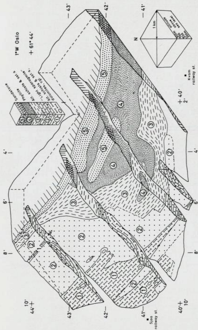
Fig. 1. Tectonogram of an area at the north side of the Gudbrandsdalen valley between
